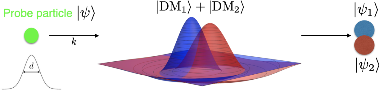
Figure 1: The basic setup of the problem; this figure is taken from our previous paper Ref. [1]. Suppose there is some piece of matter that primarily only interacts gravitationally, dark matter, and it forms a dark-matter-Schrödinger-cat-state (DMSCS). This is defined as a quantum superposition of two different configurations of some piece of the DM, |\text{DM}_1\rangle + |\text{DM}_2\rangle , as illustrated by the blue and red distributions. The distributions can differ in the center of mass position and/or profile of the mass distribution or, for light bosonic DM, the phase of the oscillating DM field. Now also suppose there is a probe particle (wave packet with wavenumber k and width d ) in state |\psi\rangle which passes through; its gravitational interaction with the DMSCS ensures that it evolves into a superposition of states |\psi_1\rangle and |\psi_2\rangle , and so it is then entangled with the DM.
