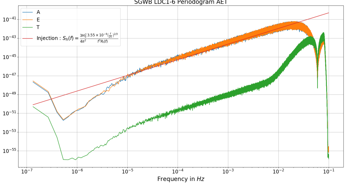
FIG. 3. Periodogram of the channels ( A, E, T ) of the SGWB from MLDC ( LDC1-6 noiseless) with an single background ( \Omega_{GW}(f) = 3.55 \times 10^{-9} \left(\frac{f}{25\text{Hz}}\right)^{2/3} )
