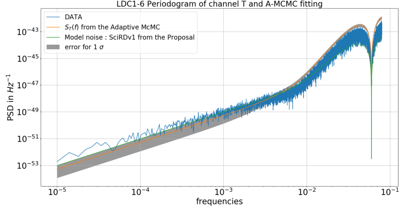
FIG. 4. Power spectral density of the channel T from the MLDC (in blue) [17]. The green line represents the analytic noise model of the power spectral density of the channel T with the parameters from the proposal [33]. The orange line is the model from Eq. 23 with the values fit with the MCMC. In grey is the 1\sigma error. This is the uncertainty calculated from Eq. 37, where we take dPSD_T with dN_{pos} = \sigma_{N_{pos}} and dN_{acc} = \sigma_{N_{acc}} ; \sigma is the standard deviation of the posterior estimation. See Fig. 5 and Eq. 26.
