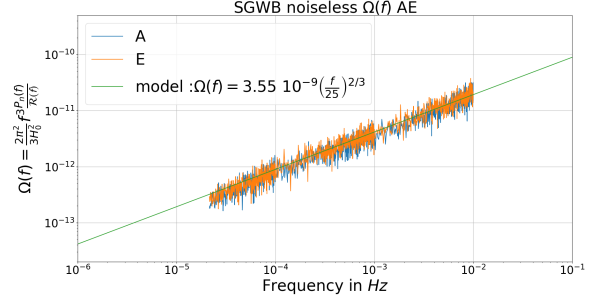
(b) Reduce frequency band 2.15 \times 10^{-5} to 9.98 \times 10^{-3} Hz of Channels A and E
