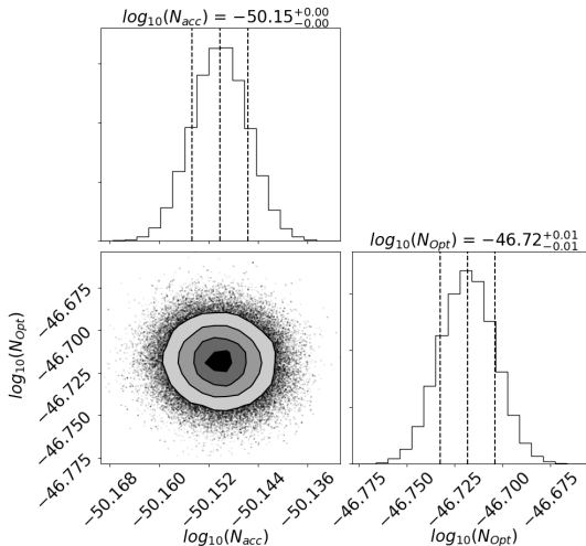
FIG. 5. Corner plot of the A-MCMC of the power spectral density of the Channel T of the MLDC dataset, fitting of the two magnitudes of the LISA noise model from the proposal [33], the vertical dash lines on the posterior distribution represent from left to right the quantiles [16%, 50%, 84%].
