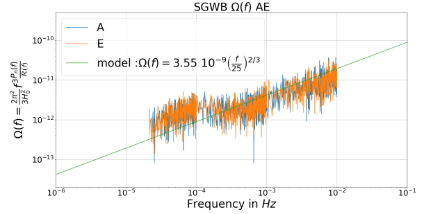
(b) Reduce frequency band 2.15 \times 10^{-5} to 9.98 \times 10^{-3} Hz of Channels A and E
