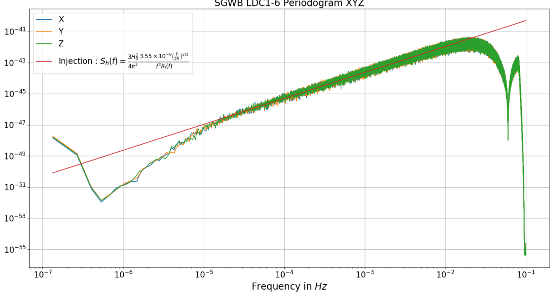
FIG. 2. Periodogram of the channels ( X, Y, Z ) of the SGWB from MLDC ( LDC1-6 noiseless) with a single background ( \Omega_{GW}(f) = 3.55 \times 10^{-9} \left(\frac{f}{25\text{Hz}}\right)^{2/3} )
