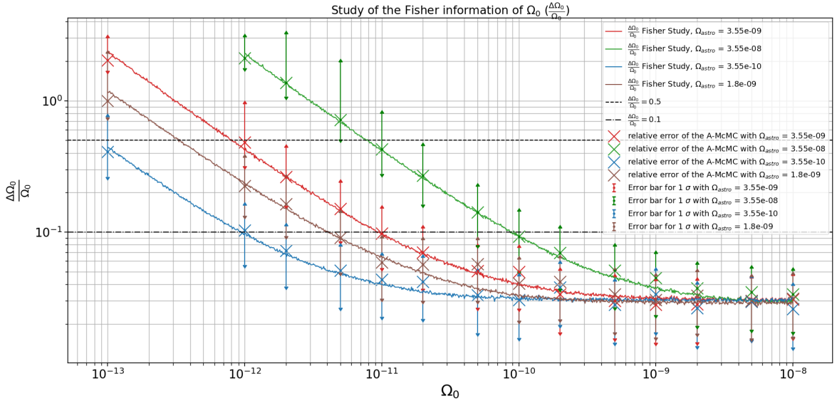
FIG. 11. Uncertainty of the estimation of the parameter \Omega_0 (the spectral energy density of the cosmological SGWB) from the Fisher Information study (displayed with lines), and the parametric estimation from the A-MCMC (with the scatter points) for the channel A and E , with the noise channel T . We conduct the study with different value for the astrophysical magnitude \Omega_{astro} . There are error bars for the four sets of A-MCMC runs; see Eq. 32. The horizontal dashed line represents the error level of 50%. This is the limit fixed to be where it is possible to measure the cosmological SGWB. The semi-dashed line represents the 10% error.
