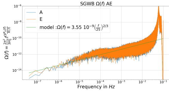
(a) Total frequency band of Channels A and E
