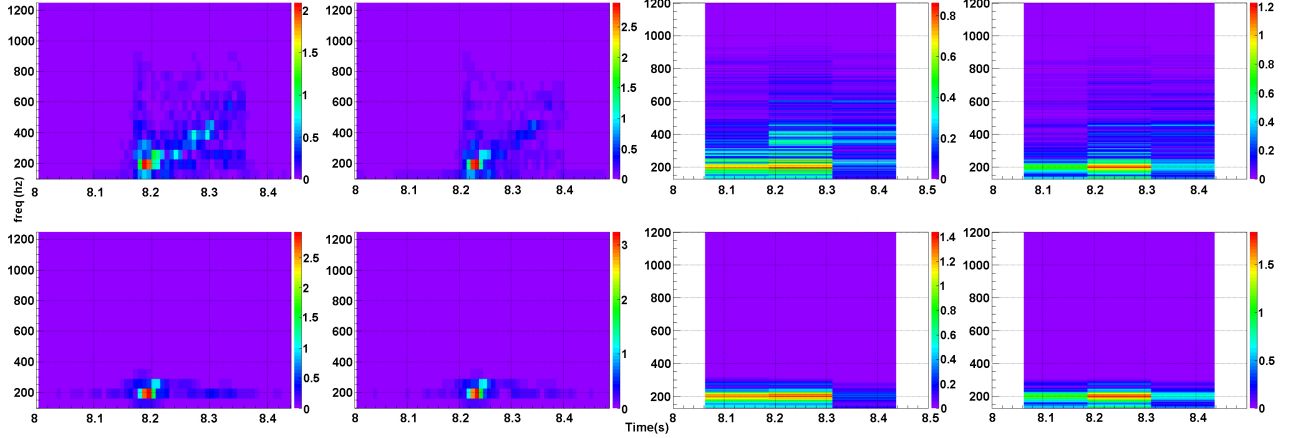
FIG. 30. The figure shows the reconstruction of the detected signal spectrum at the H1 and L1 detectors for Kuroda 2017 s11 waveforms as obtained by the cWB and the MuLaSECC pipelines for an injection with SNR 15. In this figure, the cWB results are in the two left hand columns and the MuLaSECC results are in the two right hand columns. For each pipeline, the left hand column presents results from H1 and the right hand column present results from L1. The top panels show the time-frequency plots for the band-limited signal. The bottom panels display the same for the reconstructed signal.
