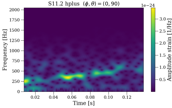
FIG. 6. The figure shows the spectrogram of the Kuroda 2017 S11 waveform. Only h_+ is seen here.
