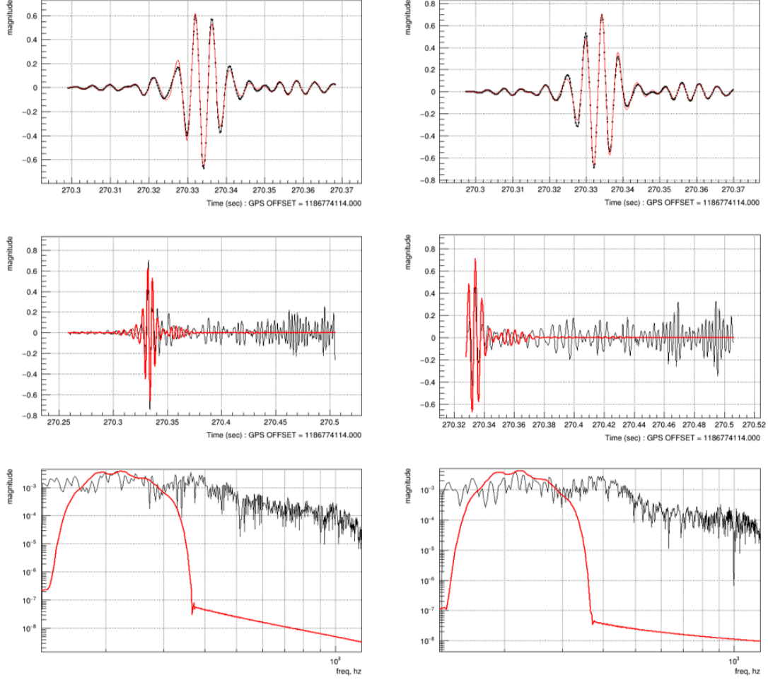
FIG. 17. The figure shows the reconstruction of the detected Ott 2013 s27 signal waveform at the H1 and L1 detectors. In this figure, the L1 results are in the left hand column and the H1 results are in the right hand column. The top panels show the band-limited signal with the original in black and the reconstructed signal in red. The middle panels show the Injected (in black) vs reconstructed (in red) whitened signal timeseries. The bottom panels display the amplitude spectra of the injected (black) vs reconstructed (red) whitened signal data.
