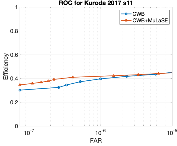
FIG. 15. The figure shows the receiver operating characteristics (ROC) of the Kuroda 2017 s11 waveform.
