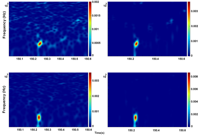
FIG. 28. This figure shows the spectrogram of signal detected at an output SNR of 14.7 by the cWB pipeline (left column, H1 at the top and L1 at the bottom); MuLaSECC pipeline (right column, H1 at the top and L1 at the bottom) detected an output SNR of 20.8. The injected Kuroda 2017 s11 signal was at SNR=15.
