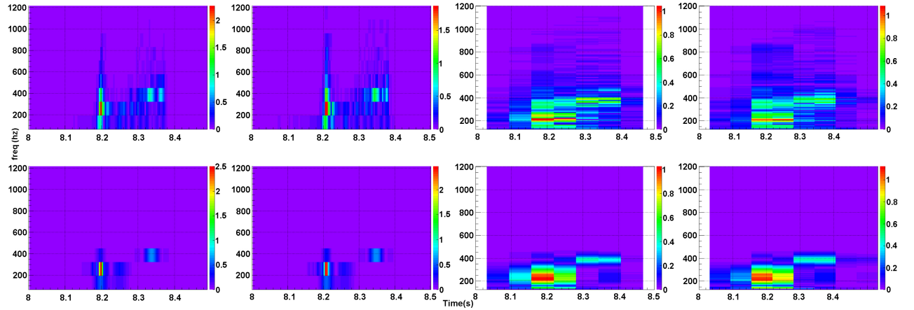
FIG. 33. The figure shows the reconstruction of the detected signal spectrum at the H1 and L1 detectors for Ott 2013 s27 waveforms as obtained by the cWB and the MuLaSECC pipelines for an injection with SNR 15. In this figure, the cWB results are in the two left hand columns and the MuLaSECC results are in the two right hand columns. For each pipeline, the left hand column presents results from H1 and the right hand column present results from L1. The top panels show the time-frequency plots for the band-limited signal. The bottom panels display the same for the reconstructed signal.
