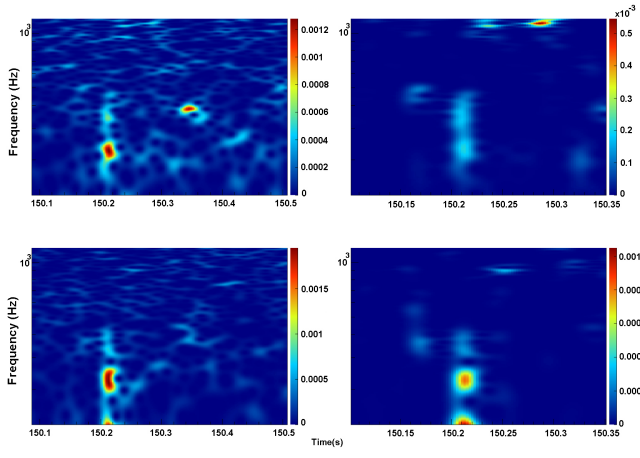
FIG. 25. This figure shows the spectrogram of signal detected at an output SNR of 10.6 by the cWB pipeline (left column, H1 at the top and L1 at the bottom); MuLaSECC pipeline (right column, H1 at the top and L1 at the bottom) detected an output SNR of 11.9. The injected Ott 2013 s11 signal was at SNR=10.
