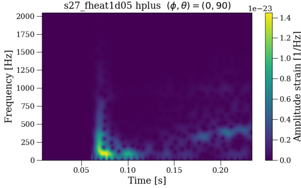
FIG. 9. The figure shows the spectrogram of the Ott 2013 S27 waveform. Only h_+ is seen here.
