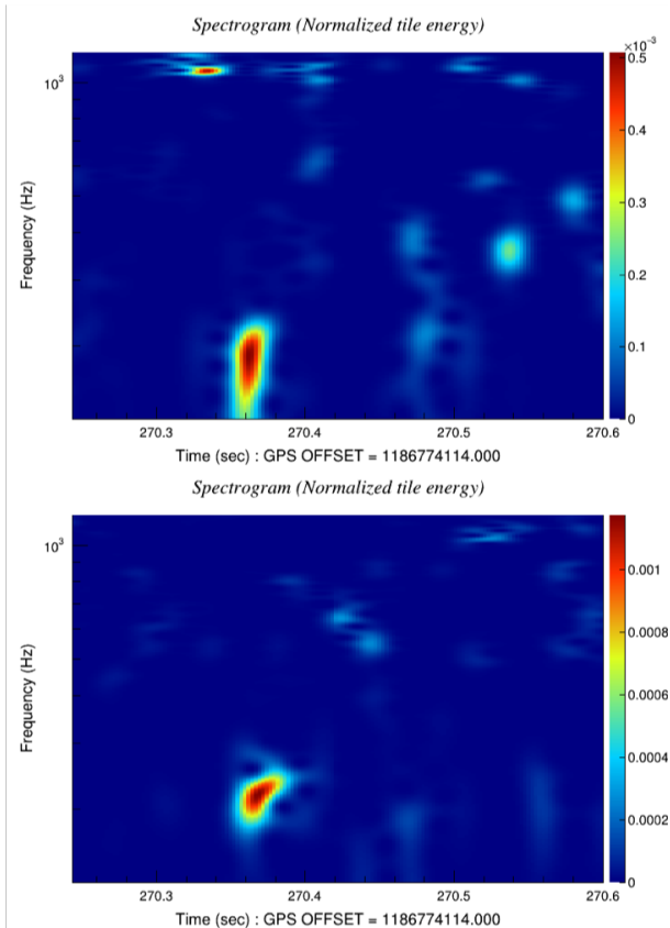
FIG. 19. This figure shows the spectrogram of the Kuroda 2017 s11 signal detected at an output SNR of 7.8 by the MuLaSECC pipeline for the L1 (bottom panel) and the H1 (top panel) detectors.
