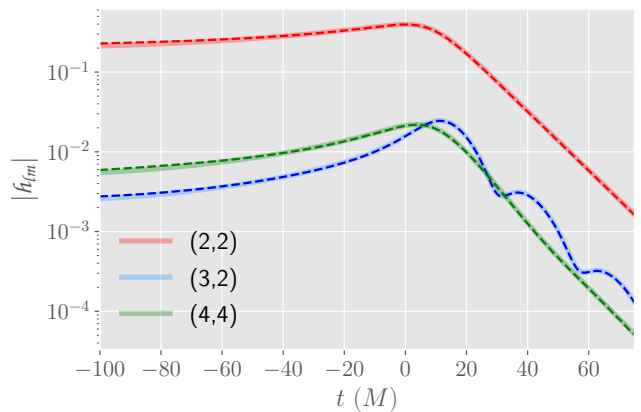
Figure 9. The absolute values of different spherical-harmonic modes are shown as dashed (solid) curves for the surrogate (NR) for SXS:BBH:2308, for which the surrogate produces largest flat noise mismatch ( \sim 0.04 ). The parameter values for this waveform are: e_{\text{ref}} = 0.176 and l_{\text{ref}} = 2.51 . Mode mixing for the (3, 2) mode is clearly seen in the ringdown signal of the NR waveform and is accurately reproduced by the surrogate.
