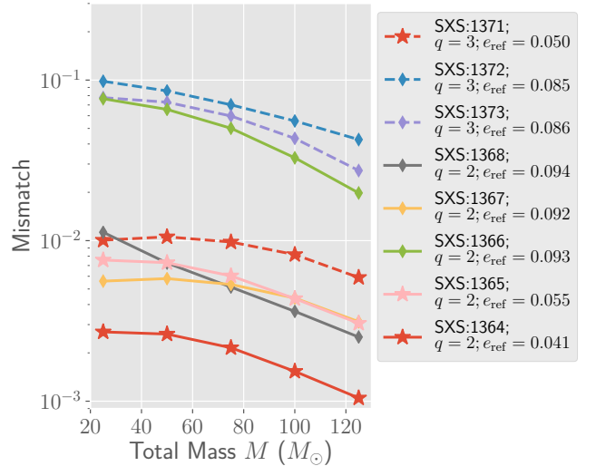
Figure 11. Mismatches against NR for the NRSur2dq1Ecc+ model (a simple extension of NRSur2dq1Ecc ) when the surrogate is evaluated beyond its training parameter range ( q = 1 ). The mismatches are shown as a function of the binary total mass M (at \iota = \pi/3 , \varphi_0 = 0.0 ), and are computed using the advanced LIGO design sensitivity noise curve. We show mismatches for q = 2 ( q = 3 ) as solid lines (dashed lines). We use star markers to denote waveforms with e_{\text{ref}} smaller than \sim 0.05 and diamond markers for the rest. All eccentricity values are computed at a reference time of t_{\text{ref}} = -2000M .
