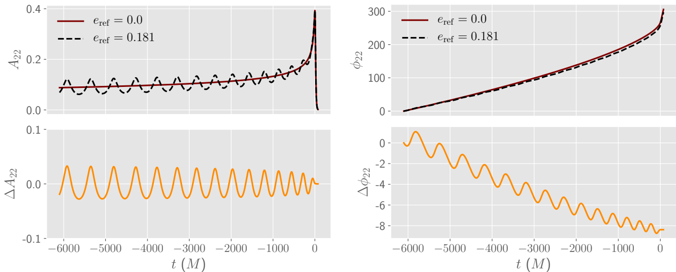
Figure 4. Example decomposition of the amplitude and phase of the (2, 2) mode. Upper left: Amplitude A_{22} of the eccentric waveform SXS:BBH:2304 (with eccentricity e_{\text{ref}} = 0.181 ) along with the amplitude A_{22}^0 of the noneccentric waveform SXS:BBH:1155. Lower left: The residual amplitude \Delta A_{22} = A_{22} - A_{22}^0 . Upper right: Phase \phi_{22} of the eccentric waveform SXS:BBH:2304 and the phase \phi_{22}^0 of the noneccentric waveform SXS:BBH:1155. Lower right: The residual phase \Delta\phi_{22} = \phi_{22} - \phi_{22}^0 . In this work we model \Delta A_{22} and \Delta\phi_{22}
