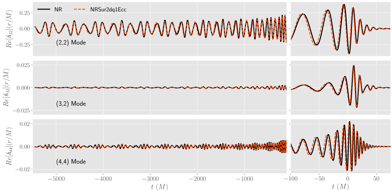
Figure 8. Real part of the waveform modes for the case that results in the largest flat noise mismatch ( \sim 0.04 ) for NRSur2dq1Ecc (red dashed line) in the left panel of Fig 7. We also show the corresponding NR waveform, SXS:BBH:2308 (black solid line). The parameter values for this waveform are: e_{\text{ref}} = 0.176 and l_{\text{ref}} = 2.51 . Note that this plot is generated using a trial surrogate that was not trained using this NR waveform data.
