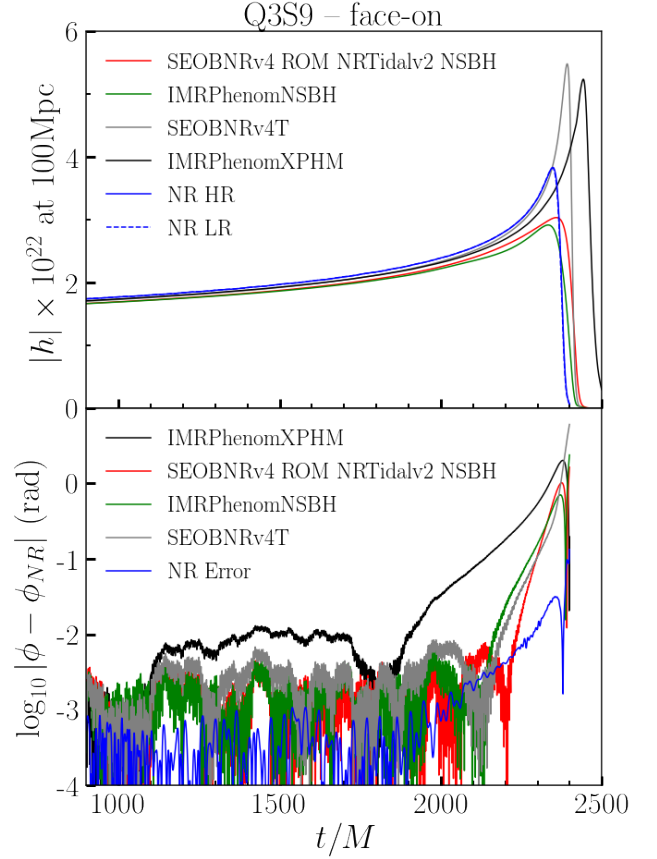
FIG. 14. Top : Amplitude of the complex strain h = h_+ + ih_\times for system Q3S9 seen face-on. We show results for our low- and high-resolution simulations, for the two BHNS models, as well as for one tidal model that does not include neutron star disruption and one BBH model that includes precession and higher-order modes. Bottom : Phase difference between the models and the high-resolution numerical result. All signals are aligned by minimizing the phase difference in the time interval t \in [500, 2000]M .
