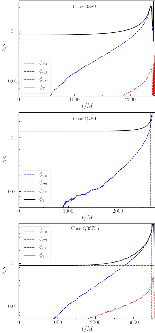
FIG. 4. Estimates of the phase error for the (2, 2) mode of the GW signal in each simulation. We include the impact of mass losses ( \Phi_{\text{dM}} ), extrapolation error ( \Phi_{\text{ext}} ), and grid resolution ( \Phi_{\text{dis}} ), following the methods described in [16] and Sec. III B. The vertical dot-dashed curves indicate t_{\text{peak}} .
