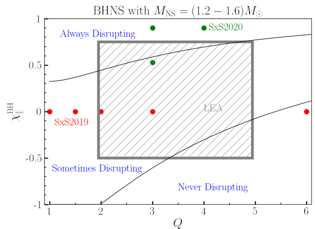
FIG. 2. Distribution of the BHNS simulations in the SXS catalogue projected in the Q - \chi_{\text{BH}}^{\text{BH}} plane. Simulations from [16] are red dots (SXS2019), while simulations from this work are green dots (SXS2020). The region of parameter space covered by 134 short waveforms from [10] is shown in grey (LEA). For context, we also show the regions of parameter space where (1.2 - 1.6)M_{\odot} neutron stars satisfying the equations of state constraints of [27] always disrupt, disrupt for some equations of state and/or neutron star masses only, or never disrupt, according to the fitting formula from [34].
