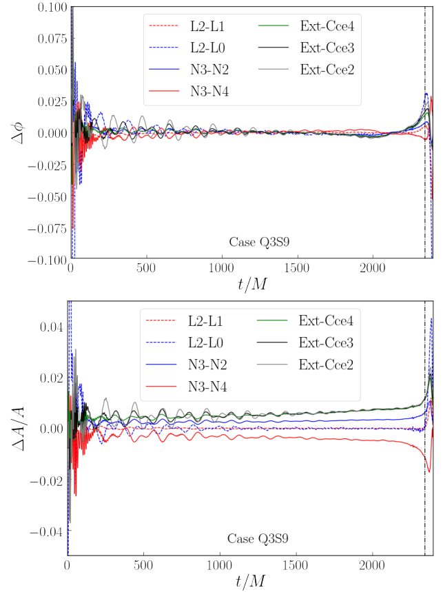
FIG. 11. Same as Fig. 10, but after applying a highpass filter to all signals to remove the drift in the average value of the strain ( 10^{\text{th}} order Butterworth filter with critical frequency of 0.002M^{-1} \approx 72 \text{ Hz} ). We note that this filter leads to changes in the phase of the signal that are larger than any of the errors displayed here; this plot indicates that most of the error observer in Fig. 10 is indeed due to a slow drift in the average value of the strain, but the filtering does not provide us with a better waveform template.
