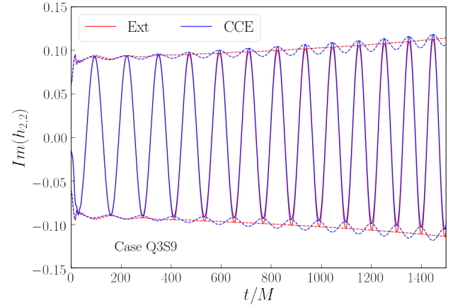
FIG. 9. Imaginary part of the (2,2) mode of the GW strain ( h_\times polarization) using CCE extraction from R = 400M and extrapolation with N = 3 . The dotted line show the amplitude of the signal ( \sqrt{|h|^2} ). In the CCE results, the average value of the strain is shifted away from 0 during the first \Delta t \sim 1000M .
