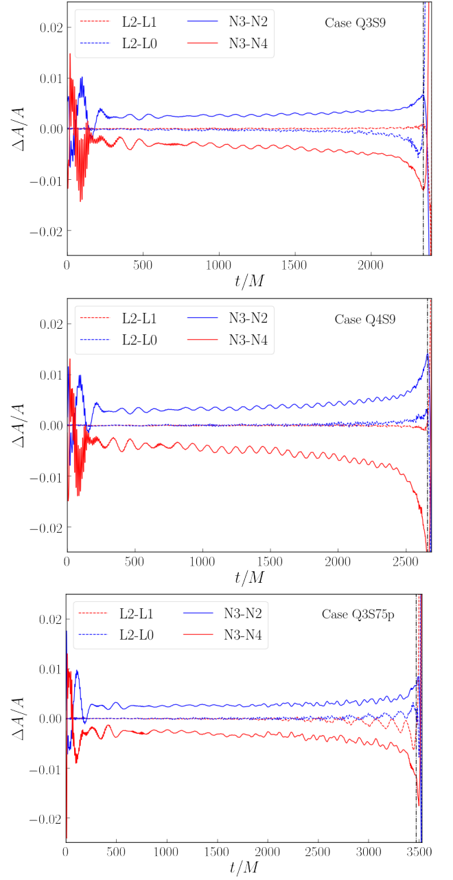
FIG. 5. Estimates of the relative error in the amplitude of the (2, 2) mode of the GW signal for each simulation. From top to bottom, we show results for Q3S9, Q4S9, and Q3S75p. Dashed curves show comparisons between the amplitude obtained with different numerical resolutions ( L0 , L1 , L2 ), while the solid curves show comparisons between the amplitude for different extrapolation orders ( N2 , N3 , N4 ). The vertical dot-dashed curves indicate t_{\text{peak}} . We clearly see that extrapolation is the main source of error when estimating the GW amplitude. Amplitude errors are \lesssim 1\% , except for simulation Q4S9 at the time of merger.
