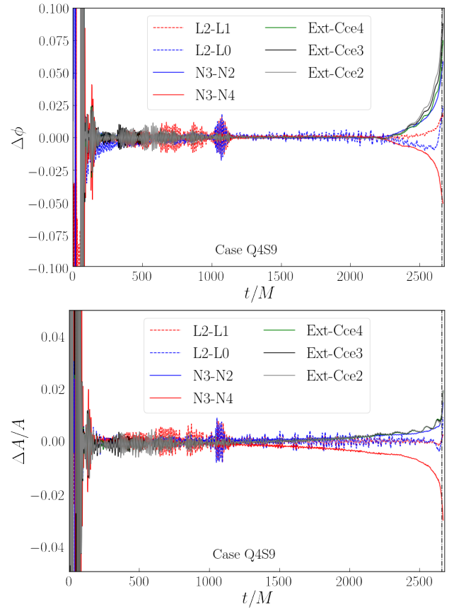
FIG. 7. Same as Fig. 6, but for the (2,2) mode of \Psi_4 in the Q4S9 configuration. We find very similar results, including very good agreement between all CCE results and the N = 2 extrapolation results.
