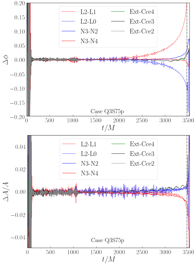
FIG. 8. Same as Fig. 6, but for the (2,2) mode of \Psi_4 in the Q3S75p configuration.
