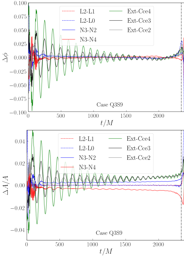
FIG. 10. Same as Fig. 6, but for the (2, 2) mode of the GW strain. For all CCE waveforms, we subtract a constant value from the strain (see text). Early-time oscillation in the CCE results are due to the initial drift in the average value of the GW strain.
