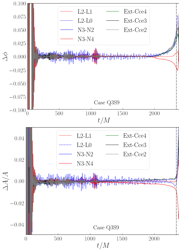
FIG. 6. Difference in the phase of the (2,2) mode for various estimates of \Psi_4 in system Q3S9, after application of a time and phase shift minimizing the phase error in the window t \in [500, 2300] . We show phase differences between our numerical resolutions (L0,L1,L2), between different extrapolation orders (N2,N3,N4, for the highest resolution simulation), and between the highest resolution simulation with N = 3 and the waveforms obtained using CCE from data extracted at R = 200M (Cce2), R = 300M (Cce3), and R = 400M (Cce4). We see very good agreement between the various CCE waveforms, and between N = 2 extrapolation (solid blue curve) and CCE.
