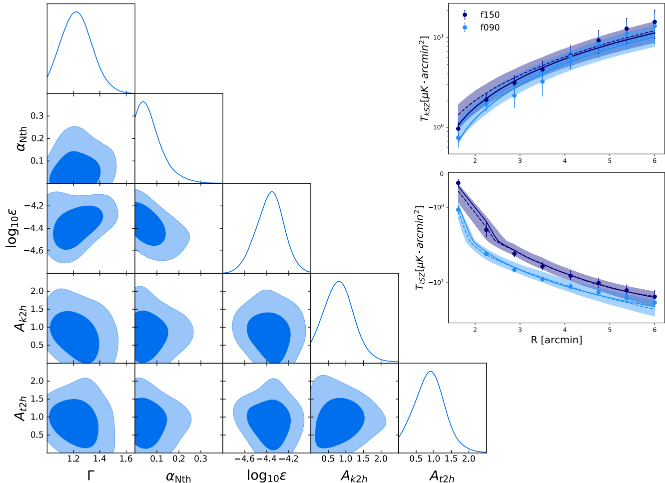
FIG. 1. Constraints on the polytropic index, \Gamma , the amplitude of the non-thermal pressure profile, \alpha_{\text{Nth}} , the feedback efficiency parameter, \epsilon , and the amplitudes of the two-halo terms of the density and pressure profiles, A_{k2h} and A_{t2h} , obtained by fitting the OBB model to combined kSZ and tSZ measurements by [18]. The radial data have large correlations (see Fig. 7 in [18]) that are accounted for in the analysis. The triangle plot shows one and two dimensional projections of the posterior probability distributions of the free parameters. We assume uniform priors within: 1 < \Gamma < 5/3 , 0 < \alpha_{\text{Nth}} < 0.8 , -4.8 < \log_{10} \epsilon < -4.0 , 0 < A_{k2h} < 5 , 0 < A_{t2h} < 5 . The top right panels show the observed kSZ and tSZ profiles (points) with the best-fit and the 2\sigma range (2nd-98th percentiles) of the distribution of the models obtained from the MCMC chains.
