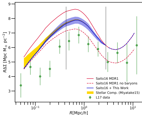
FIG. 5. CMASS galaxy-galaxy lensing signal. Data from [26] (green circles) are compared to HOD model predictions from [95] (MDR1, red line) and our model that include a baryons correction (blue line) to the MDR1. This correction uses the best fit density profile from kSZ measurements (Section III B and Figure 3). The gold band illustrates the uncertainty in the model from the stellar component and the vertical grey lines show the radial range in which we have kSZ observations; outside this radial range we are extrapolating. The baryon correction that we estimated to the MDR1 model reduces the difference between the galaxy-galaxy measurements and HOD model predictions by half (50%), but does not reconcile it. The dashed red line illustrates the maximum correction to the MDR1 model, which is to remove all baryons without altering the dark matter profile. This extreme model still does not reconcile this model and observations below 500 kpc/h.
