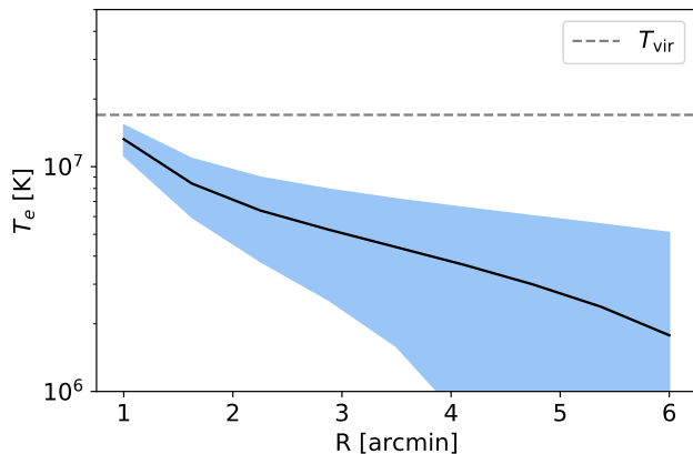
FIG. 2. Average, inferred electron temperature profile of CMASS galaxies halos weighted by density obtained from the joint kSZ+tSZ fit to the OBB model using the MCMC chains. The black line is the median profile, the blue band indicates the 2\sigma range of the models obtained from the MCMC chains. For comparison, the grey dashed line indicates the expected virial temperature for an isothermal sphere of mass equal to the mean mass of our CMASS sample ( M_{200} = 3.3 \times 10^{13} M_{\odot} ), T_{\text{vir}} = 1.7 \times 10^7 K. The x-axis is converted to arcmins to ease the comparison to the density and pressure profiles. The average temperatures of the CMASS galaxies are closer to 10^7 K than they are to 10^6 K.
