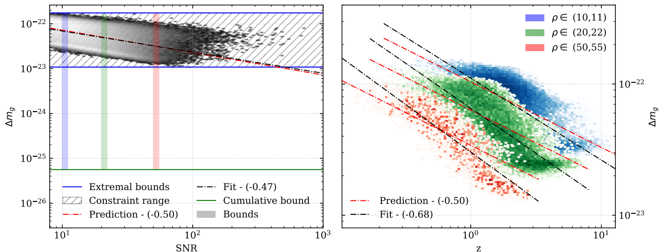
FIG. 25. Result of the scaling analysis outlined in Sec. VIB7 performed on the data synthesized with the HLVKIO8 network and the SPOPS 0 population. The plotting style is the same as in Fig. 12. The left panel shows a heat map of the constraint on m_g versus the SNR of the source. The right panel shows the density of the constraint versus the redshift z , with empirical trends shown in black and predicted trends shown in red. Because of the narrow range of constraints in the catalog and the large enhancement of the cumulative bound over the strongest single observation, stacking observations is quite efficient for this modification. The right panel shows that there is indeed a trend in the \Delta m_g - z relation (although the distributions are moderately wide) which would favor sources far from Earth, and would primarily benefit MBH sources.
