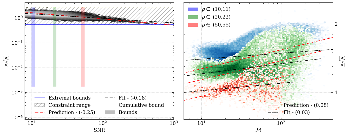
FIG. 16. Result of the scaling analysis outlined in Sec. VIB3 performed on the data synthesized with the HLVKIO8 network and the SPOPS 0 population. The plotting style is the same as in Fig. 12. The left panel shows a heat map of the constraint on \sqrt{\Lambda} versus the SNR of the source. The right panel shows the density of the constraint versus the chirp mass, with empirical trends shown in black and predicted trends shown in red. The small range of constraints from the catalog lead to considerable enhancements of the cumulative bound when stacking observations, and the weak scaling with chirp mass and moderate scaling with SNR further benefit SOBH sources over other source classes.
