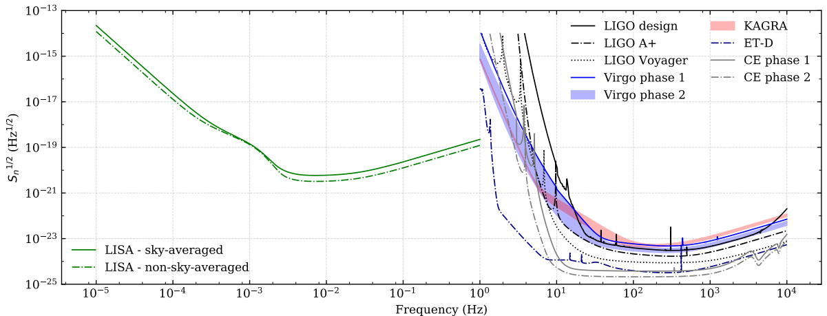
FIG. 2. Noise curves for the various detector configurations studied in this work. The shaded bands observed for the Virgo+phase 2 and KAGRA sensitivities reflect uncertainties in estimates of their anticipated power spectral densities.
