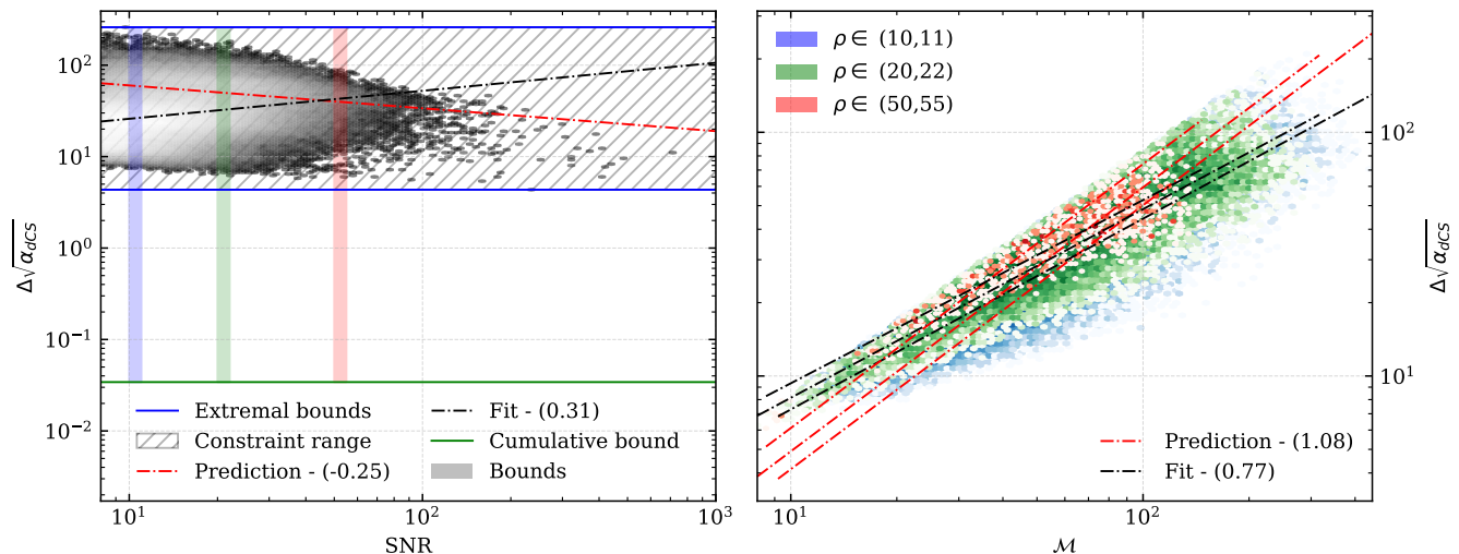
FIG. 18. Result of the scaling analysis outlined in Sec. VIB4 performed on the data synthesized with the HLVKIO8 network and the SPOPS 0 population. The plotting style is the same as in Fig. 12. The left panel shows a heat map of the constraint on \sqrt{\alpha_{dCS}} versus the SNR of the source. The right panel shows the density of the constraint versus the chirp mass, with empirical trends shown in black and predicted trends shown in red. Our prediction for the SNR scaling is considerably less accurate than for previous theories, presumably from covariances with other source parameters and competing scaling trends with the chirp mass. The tight range of constraints and large improvement of the cumulative bound over all other single source constraints, seen in the left panel, indicate strong dependence on the total number of sources in the catalog.
