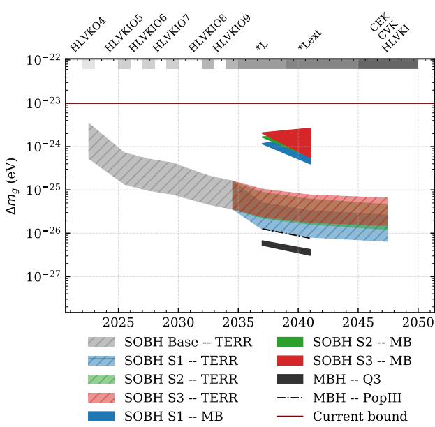
FIG. 24. Projected cumulative constraints on the mass of the graviton, m_g , for the detector networks and population models examined in this paper. Our models show that MBH sources observed by LISA will perform the best at constraining this modification, but only slightly better than the terrestrially-observed only sources. Multiband sources perform the worst, as they received no benefits from the Jacobian and already perform only moderately well for positive PN order effects.
