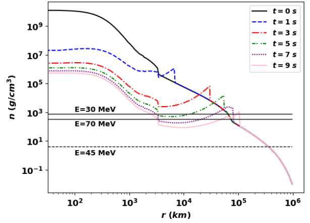
FIG. 2. (Color online) The density for the progenitor model and various post-bounce times. The solid horizontal lines represent the high resonance densities for 30 MeV and 70 MeV neutrinos. The dashed horizontal line represents the low resonance density for a 45 MeV neutrino.
