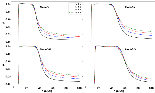
FIG. 4. (Color online) The jumping probability p defined in Eq. (12) for models I-IV calculated as a function of energy at even seconds. At earlier times, the spectral swap is closer to being sharp. But at later times, the splits become less and less sharp in the high energy region.
