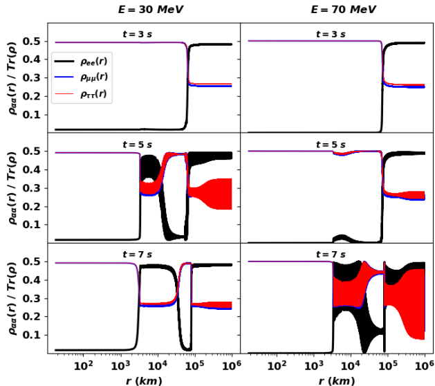
FIG. 6. (Color online) The evolution of 30 MeV (left panels) and 70 MeV (right panels) neutrinos in the case of NH for Model I at 3 s, 5 s, and 7 s. At earlier times neutrinos go through one adiabatic high resonance. At later times, they go through three high resonances and the adiabaticity is temporarily broken for each energy.
