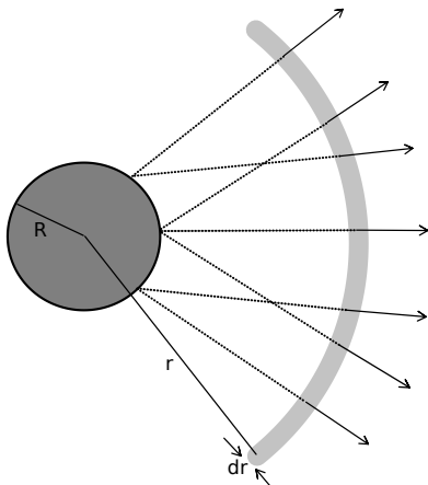
FIG. 1. Schematic picture of neutrino emission from the proto-neutron star, and the neutrino ensemble represented by the density operator \hat{\rho}_t(E, r)dtdE in the neutrino bulb model [27]. See the text for details.
