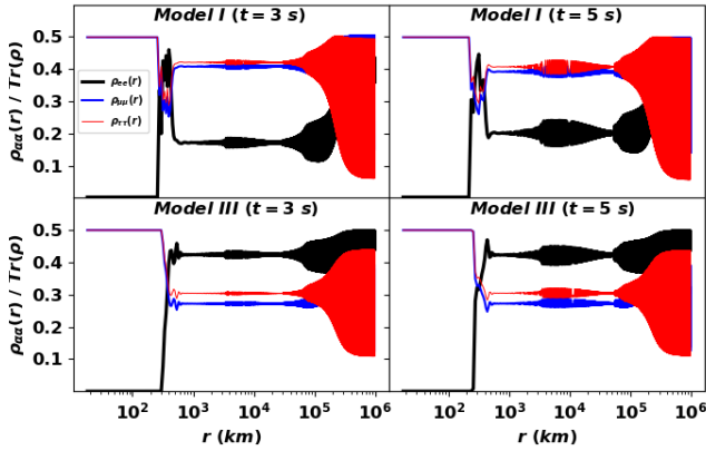
FIG. 5. (Color online) The oscillations of the diagonal elements of the density operator in flavor basis due to the partial adiabaticity of collective oscillations. These examples show a 45 MeV neutrino in IH for models I and III at 3 s and 5 s. For other models, energies, and times, the behaviour is similar.
