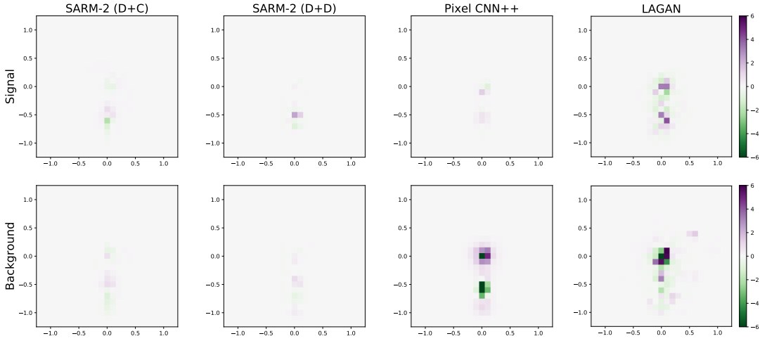
FIG. 15. Error measured by subtracting of the pixel-wise average of the images created by each generative model and the pixel-wise average of the images generated with Pythia. The SARM models have lower error than both Pixel CNN++ and LAGAN with most of the errors are concentrated in the center of the image.
