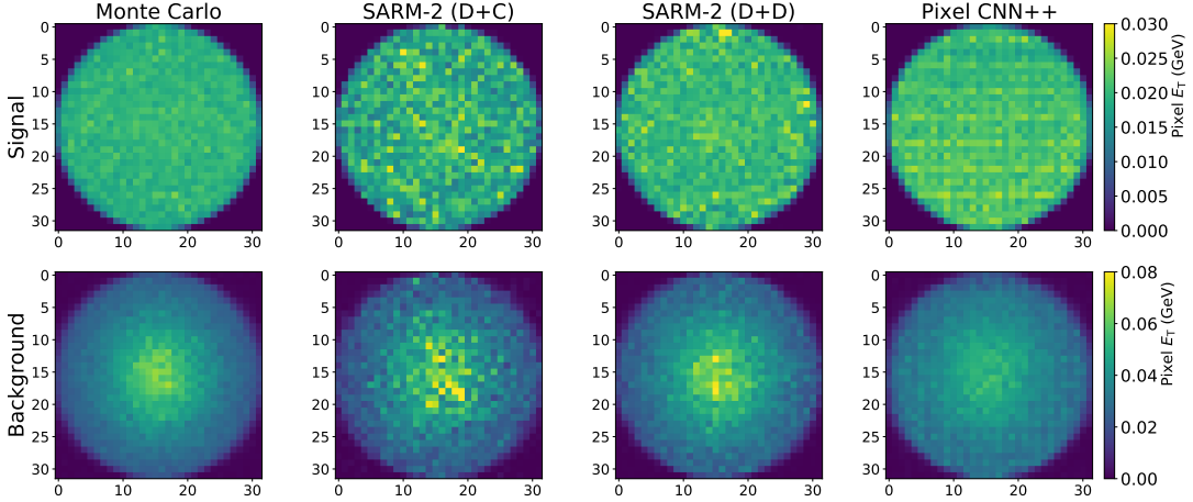
FIG. 11. Pixel-wise averages of calorimeter images in the vicinity of a muon from the generative models as well as the original Monte Carlo generator. Top row shows isolated muons (signal), where little calorimeter activity is expected. The bottom row shows muons produced in association with a jet (background), which deposits significant energy near the muon. A linear scale is used to reveal the differences between signal and background images.
