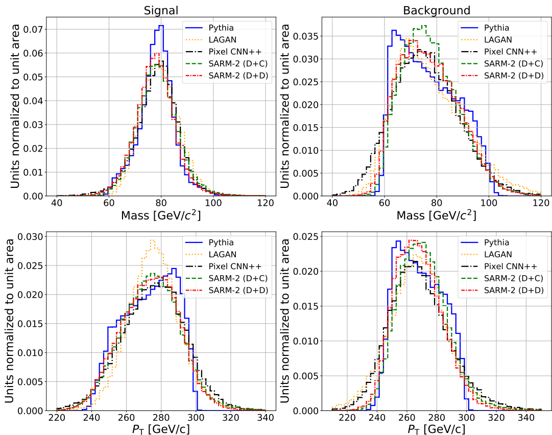
FIG. 8. Distributions of jet observables ( Top: Mass, Bottom: P_T ) calculated from images generated by several generative models and from the original images generated by Pythia. Signal images, with two collimated quarks, are on the left; background images, with a single quark or gluon, are on the right.
