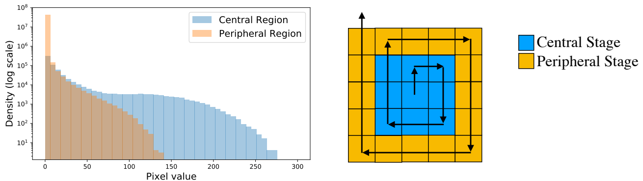
FIG. 5. (Left) Distribution of pixel values in the jet substructure dataset for the 9 pixels in the center of the images (central region) and the rest of the pixels (peripheral region). Note that the majority of the pixels in the peripheral region are zero-valued and in general have lower variance than pixels in the central region. (Right) Two-stage generation for the central and peripheral regions using a spiral path and two different SARM modules. Using different networks for each region improves performance.
