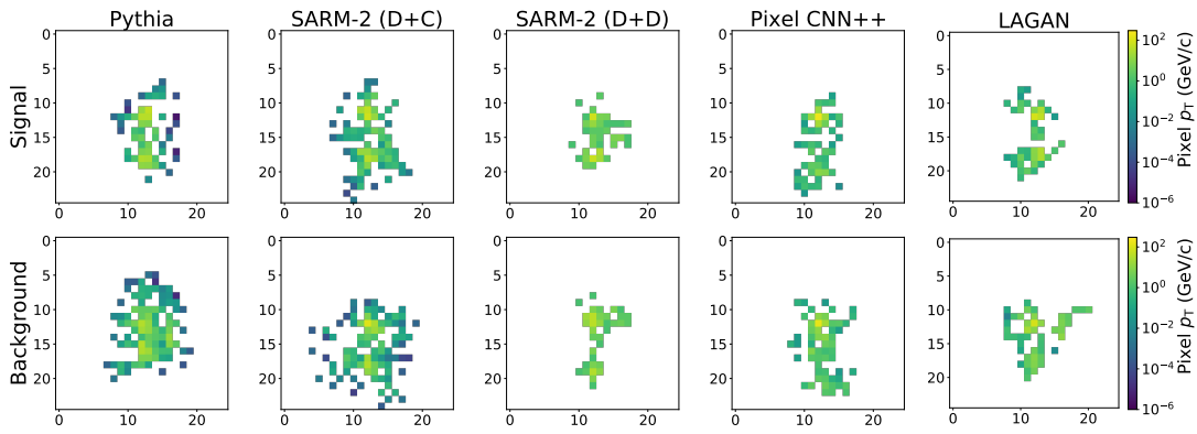
FIG. 6. Example jet images generated from each model. Notice that SARM-2 (D+C) is able to produce small value pixels in the periphery of the images. The intensity of each pixel is shown on a log scale, where the white space represents pixels with value zero.
