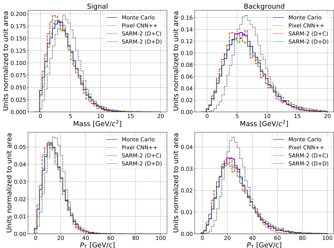
FIG. 12. Distributions of calorimeter observables (top: invariant mass, bottom: total P_T ) calculated from images generated by several generative models and the originals generated by a Monte Carlo generator. Signal images, in the vicinity of an isolated muon, are on the left. Background images, in the vicinity of a muon produced with an associated jet, are on the right.
