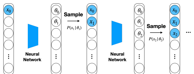
FIG. 3. Generation process of a deep autoregressive model. During generation, the first pixel x_0 is sampled from x_0 \sim P(x_0|\theta_0) . Next, the pixel x_0 is zero-padded to a D dimensional vector and passed to the neural network ARM model, which evaluates the parameters \theta = \{\theta_0, \dots, \theta_{D-1}\} , though only \theta_1 is needed to sample the next pixel x_1 \sim P(x_1|\theta_1) . The pixels x_0 and x_1 are again zero-padded to create a D dimensional vector which is passed into the neural network to generate the next pixel. This process is repeated until all pixels are generated. Note that the same neural network is used at each generation step, and part of its weight connections are disabled to preserve the autoregressive structure.
