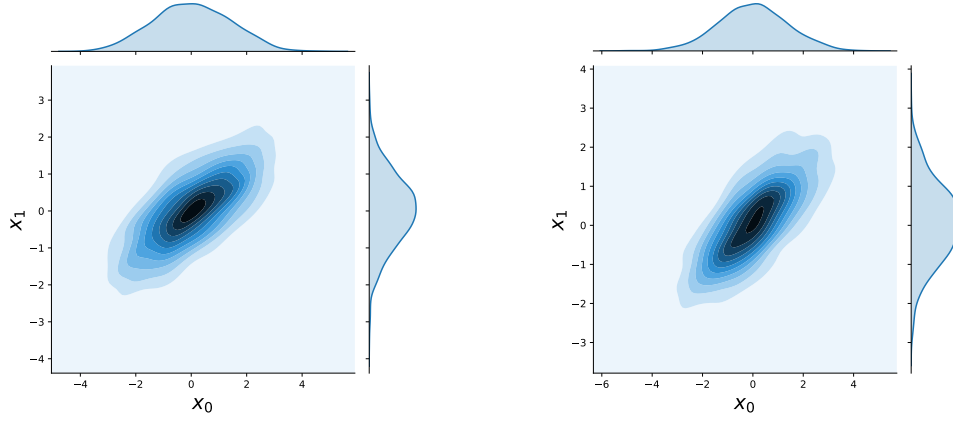
FIG. 14. Left: Density plot of training data. Right: Density plot of generated data. The two distributions are very close, showing the ARM is able to learn the joint distribution of x_0 and x_1 well.
