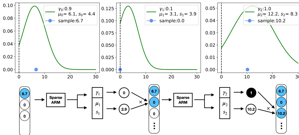
FIG. 4. Generation process for the D+C model. The blue circle dots represent the value sampled for each pixel. For example, given the first pixel value of 6.7, sampled from the empirical distribution of the dataset, the neural network outputs the distribution parameters \gamma_1 = 0.1, \mu_1 = 3.1, s_1 = 3.9 to generate the second pixel. Then a Bernoulli random variable is sampled from z_1 \sim \text{Bern}(\gamma_1) and a logistic random variable is sampled from \tilde{x}_i \sim \text{Logistic}(\mu_i, s_i) . The value of the second pixel x_i is produced by the product of these two variables as: x_i = z_i \cdot \tilde{x}_i = 0 \cdot 2.9 = 0 . This sequential process is repeated until every pixel is generated.
