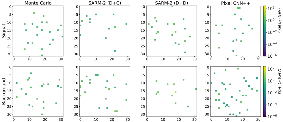
FIG. 10. Example calorimeter images in the vicinity of a muon from the generative models as well as the original Monte Carlo generator. Top row shows isolated muons (signal), while the bottom shows muons produced in association with a jet (background). The intensity of each pixel is shown on a log scale, where the white space represents pixels with value zero.
