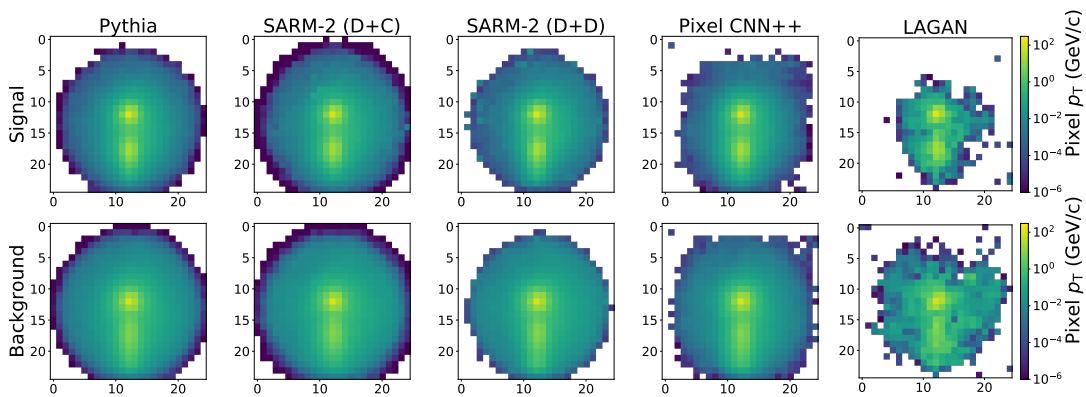
FIG. 7. Pixel-wise average of the images generated by each model. Notice that LAGAN struggles to capture the distribution of low value pixels in the periphery of the images and has a non-smooth radial transition compared to the autoregressive models. The intensity of each pixel is shown on a log scale, where the white space represents pixels with value zero.
