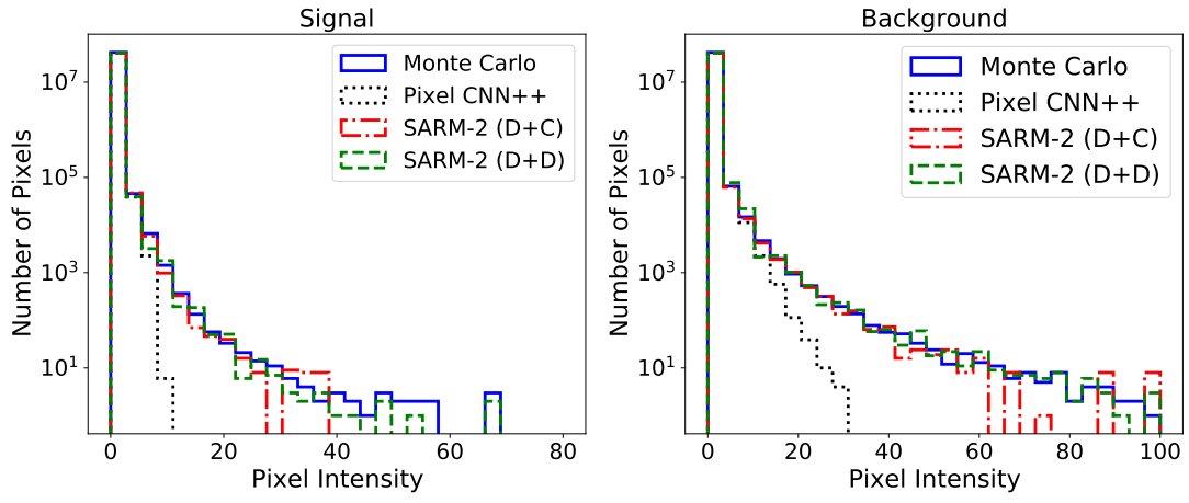
FIG. 21. Distribution of pixel intensity for muon isolation study. Pixel CNN++ under-represents the distribution while the SARM models miss the high pixel values where there are fewer events.
