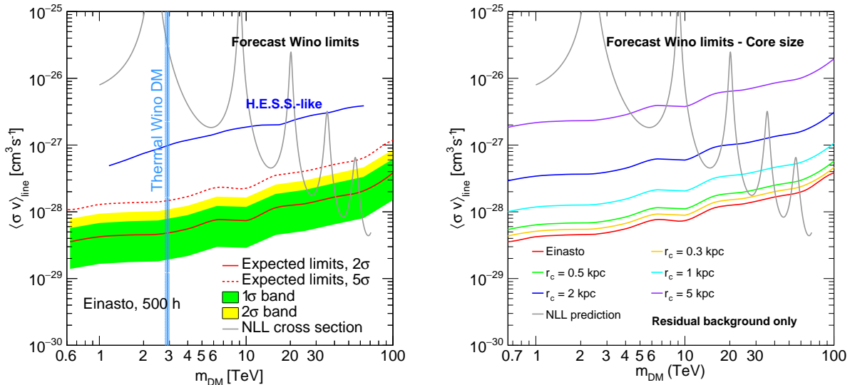
Figure 4. Expected upper limits at 95% C.L on the Wino annihilation cross section as a function of its mass for 500 h of CTA observations towards the GC. The predicted NLL cross section is shown (solid gray line) and the thermal Wino DM mass is marked (cyan solid line and bands). The only background considered here is the residual background. The full Wino spectrum is included in the expected signal. Left panel: Mean expected upper limits at 2\sigma (red solid line) for an Einasto profile are shown together with the 1\sigma (green band) and 2\sigma (yellow band) containment bands. Mean expected upper limits at 5\sigma (red dashed line) are also shown. The H.E.S.S.-like 2\sigma sensitivity extracted from Ref. [68] is shown as a blue solid line. Right panel: The expected limits are shown for cored DM profiles of size from 300 pc to 5 kpc.
