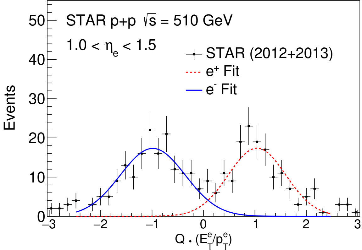
FIG. 5. Double Gaussian fit to measured EEMC Q_e \cdot E_T^e / p_T distribution using the log-likelihood method. The colored lines show individual e^+ (red dashed) and e^- (solid blue) Gaussian distributions resulting from the double-Gaussian fit.
