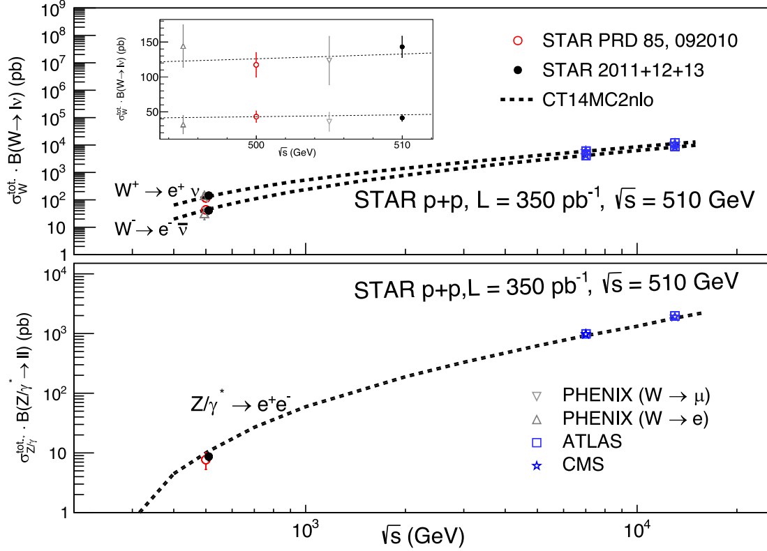
FIG. 9. The measured total W^\pm and Z cross sections for the combined STAR data sets (2011-2013). For clarity the PHENIX measurements are plotted at \sim 5 GeV from \sqrt{s} = 510 GeV ( W \rightarrow \mu ) and 500 GeV ( W \rightarrow e ), respectively. The inset plot in the upper panel highlights the STAR and PHENIX results ( \sqrt{s} \sim 500 GeV). For the Z cross section, the STAR data uses a mass window of 70 \text{ GeV} < m_{e^+e^-} < 110 \text{ GeV} , CT14MC2nlo and CMS use 60 \text{ GeV} < m_{e^+e^-} < 120 \text{ GeV} , and ATLAS uses 66 \text{ GeV} < m_{e^+e^-} < 116 \text{ GeV} . The dashed lines in the figure show the respective W^\pm and Z cross section curves computed using FEWZ and the CT14MC2nlo [56] PDF.
