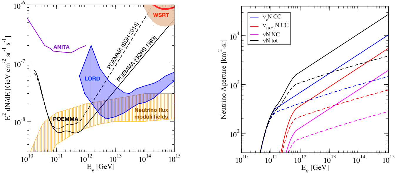
FIG. 28: POEMMA sensitivity to EAS showers produced by neutrinos interacting in the atmosphere. Left: Black curves are POEMMA sensitivity using [141] (solid) and [142] (dashed) cross sections. Predictions for strongly coupled string moduli (orange range) [136], LORD sensitivity (blue band) [139], ANITA I-IV limits (purple) [89], and WSRT [140]. Right: POEMMA neutrino aperture from fluorescence with [141] (solid) and [142] (dashed) cross sections of neutrino-nucleon scattering for CC interactions of \nu_e (blue), \nu_\mu and \nu_\tau (red); NC interactions (pink); and total (black).
