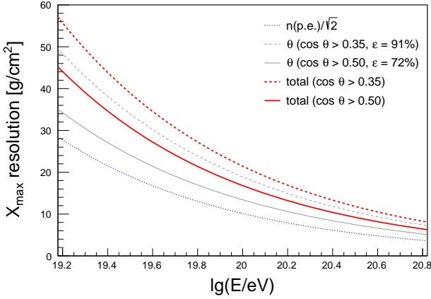
FIG. 17: Preliminary estimate of the X_{\text{max}} resolution of POEMMA in stereo mode. The contributions from the photoelectron statistics and angular resolution are shown in blue and gray respectively. The total resolution, obtained by adding both contributions in quadrature is shown in red for two cuts on the maximum zenith angle.
