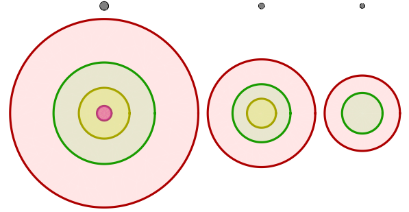
FIG. 20: Circles representing the composition-layered structure of hotspots at different energies, for proton sources (top) and nuclei sources (bottom). The radii of the circles respect the proportions of the angular sizes given by (2), for protons (black), helium (magenta), nitrogen (yellow), silicon (green) and iron (red); and for 40 \text{ EeV} (left), 70 \text{ EeV} (center) and 100 \text{ EeV} (right).
