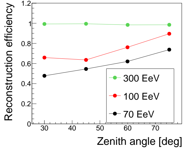
FIG. 34: Efficiency in the angular reconstruction for POEMMA as a function of zenith angle for different EAS energies.
