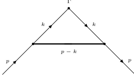
FIG. 5: SDM in the forward limit.
