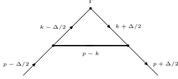
FIG. 3: SDM in a symmetric frame.
