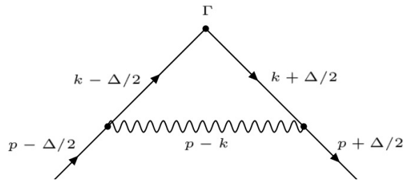
FIG. 1: QTM in a symmetric frame.
