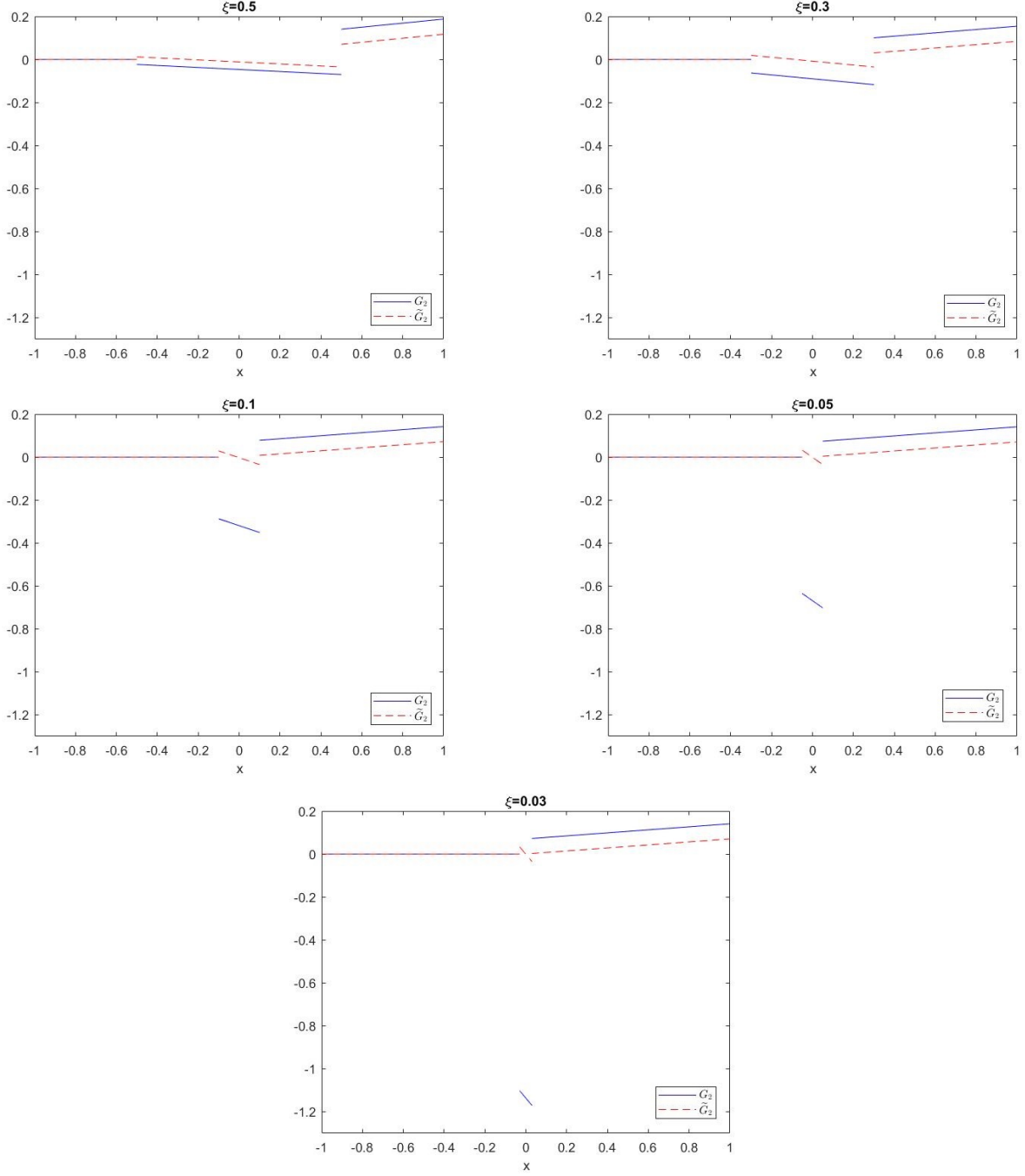
FIG. 2: Discontinuities of the twist-3 GPDs, G_2 and \tilde{G}_2 in QTM for \Lambda_\perp = 2 , and g = 1 .
