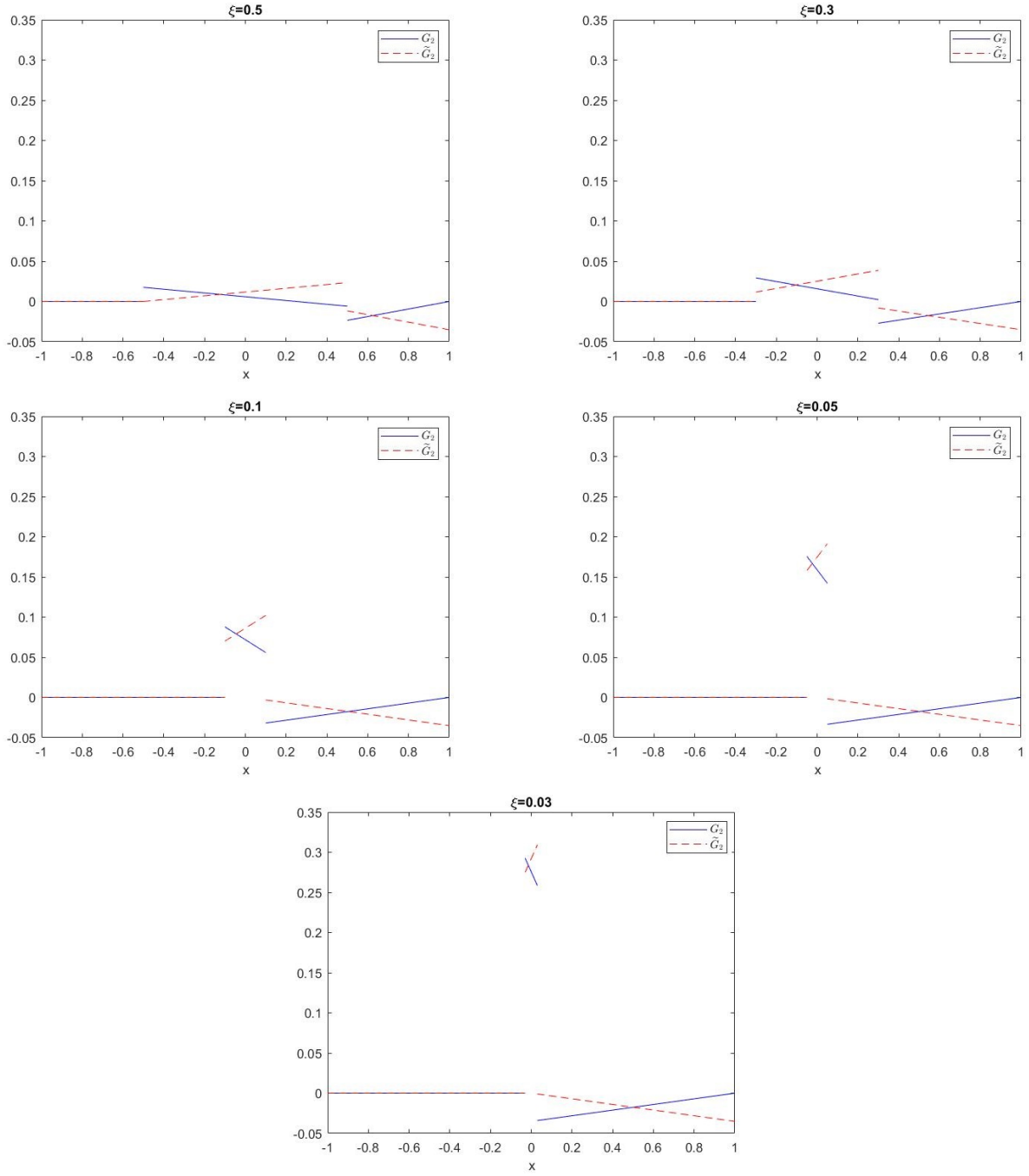
FIG. 4: Discontinuities of the twist-3 GPDs, G_2 and \tilde{G}_2 in SDM for \Lambda_\perp = 2 and g = 1 .
