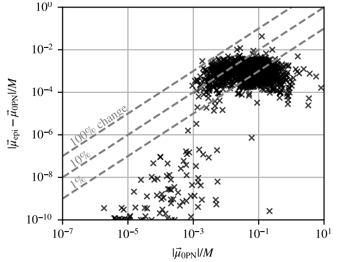
FIG. 13. Change in the size of the COM correction, \vec{\mu} as defined in Eq. (8), when removing epicycles before fitting for the COM correction, as described in Eq. (27). These changes are comparable to, but almost always smaller than, the changes due to variations in the endpoints of integration as seen in Fig. 3; they are also smaller than most of the post-Newtonian corrections seen in Fig. 7, except for systems changing here by more than about 10%.
