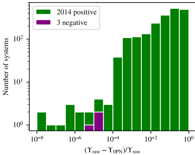
FIG. 5. Relative difference between \Upsilon_{\text{raw}} evaluated on the raw waveform data and \Upsilon_{0\text{PN}} evaluated using the values \vec{\alpha} and \vec{\beta} given by the simplest Newtonian (OPN) approximation of Eqs. (7)—the same COM correction used in the current SXS catalog. In the vast majority of cases, the value of \Upsilon decreases substantially (though it actually increases very slightly in three cases with significant eccentricity). This suggests that even though \Upsilon and the coordinate-based COM are such entirely different measures and based on completely different data, they agree that the changes introduced by naive COM corrections are generally improvements.
