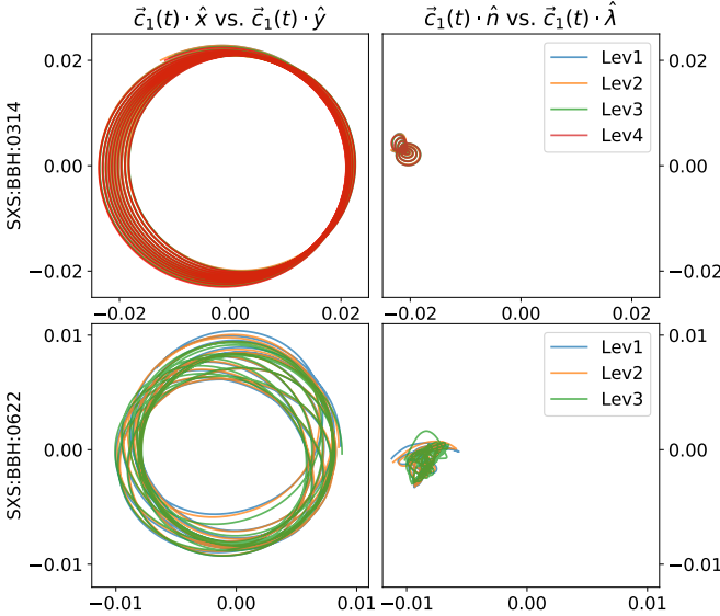
FIG. 12. Contribution to \vec{x}_{\text{COM}} which cannot be fitted by a linear drift. Left panel: Deviation of Newtonian center of mass from a linear motion, i.e. the quantity \vec{c}_1 , plotted in inertial coordinates. Right panel: Projection of \vec{c}_1(t) onto the co-rotating basis vectors \hat{n} and \hat{\lambda} . The rotation of \vec{c}_1 around the origin visible in the left panels is transformed into a nearly constant offset from the origin in co-rotating coordinates of the right panels. Shown are multiple numerical resolutions (Lev1, Lev2, ...) which fall on top of each other, indicating that the epicyclic dynamics is numerically resolved and independent of the direction of the linear drift. Data is plotted only for the time-interval [t_i, t_f] , which is used for the linear center of motion fits.
