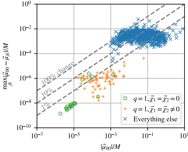
FIG. 3. Comparing the size of COM corrections in the SXS catalog, |\bar{\mu}_{00}| , to how much those corrections change under small variations in the endpoints of integration used to compute the COM correction. The vertical axis shows the largest change in the COM correction if we shift t_i and/or t_f later by half an orbit. The systems with the largest COM corrections—where these corrections are presumably the most important—change by small fractional amounts. On the other hand, there are several systems in which the COM correction changes by more than the original correction; those systems also have some of the smaller COM corrections in the catalog. The median percentage change is 4% of the original correction, and even the largest individual change is smaller than the median value of |\bar{\mu}_{00}| .
