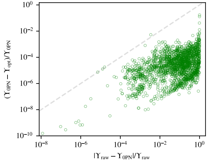
FIG. 6. Comparison between the value \Upsilon_{\text{opt}} for which \vec{\alpha} and \vec{\beta} are optimized, and \Upsilon_{0\text{PN}} evaluated using the values \vec{\alpha} and \vec{\beta} given by the simplest Newtonian (OPN) approximation—the same COM correction used in the current SXS catalog. The vertical axis shows the relative improvement in going from the Newtonian correction to the optimized correction. The dashed diagonal line represents where the comparisons are equal—the “ x = y ” line. Optimization improves the results for the great majority of systems by less than 1%. The three exceptions to this rule are particularly long systems.
