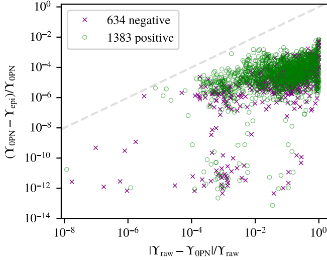
FIG. 14. This plot shows the difference between the value of Y [Eq. (17)] resulting from the naive OPN method based on the coordinate trajectories of the apparent horizons and the value resulting from the epicycle removal method described in Sec. V D. The horizontal axis shows the relative magnitude of the change when going from the raw data to the corrected waveform, while the vertical axis shows the change when incorporating the epicycle corrections. In most cases, the values of Y actually become significantly larger when going from the OPN value to the epicycle corrected value. Those systems are shown as crosses, while systems with smaller values are shown as circles.
