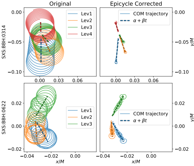
FIG. 11. Illustration of epicycle correction for the two simulations already shown in Fig. 1. The left panels show the Newtonian center of mass \vec{x}_{\text{COM}} , whereas the right panels show the epicycle corrected \vec{c}_2 . The thick dashed lines indicate linear fits to the respective center of mass trajectories: \vec{\alpha} + \vec{\beta}t (left panels) and \vec{\alpha}_{\text{epi}} + \vec{\beta}_{\text{epi}}t (right panels). Several numerical resolutions are shown (labeled Lev1 to Lev4), and data is plotted only for the time-interval [t_i, t_f] , which is used for the linear center of motion fits.
