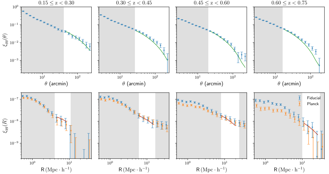
FIG. 6. Measurements of the galaxy auto-correlation ( top row ) and Compton-y galaxy cross-correlation ( bottom row ) at different redshift bins corresponding to four redshift bins used in the analysis. Solid line is the best-fit to the fiducial model of Compton-y which is generated after removing 545GHz and 857GHz frequency channels from the analysis. Only data in the unshaded regions are used for fitting. These scale cut choices are validated in §IV E
