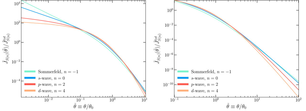
FIG. 2. The scale-free angular distribution of the gamma-ray flux from dark matter annihilation in an NFW subhalo, as function of \tilde{\theta} \equiv \theta/\theta_0 , under the approximation \theta_0 \equiv r_s/D \ll 1 . We show separately the distribution at small (left panel) and large (right panel) values of \tilde{\theta} . As in Fig. 1, the curves represent Sommerfeld-enhanced (teal), s -wave (blue), p -wave (red), and d -wave (orange) annihilation.
