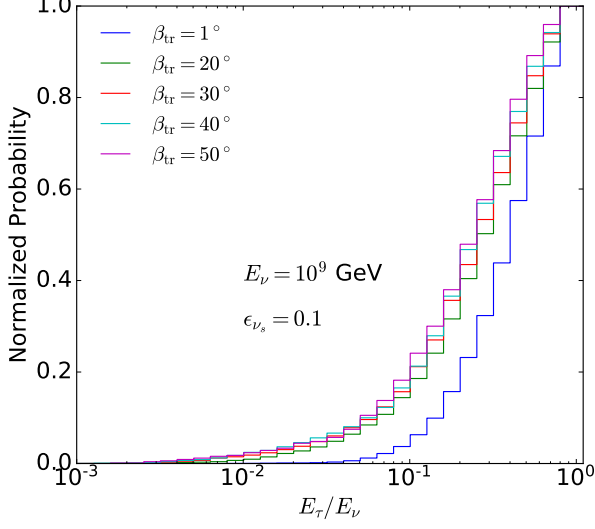
FIG. 7. The cumulative distribution functions for several values of \beta_{\text{tr}} given E_{\nu_s} = 10^9 GeV and \epsilon_\nu = 0.1 .
