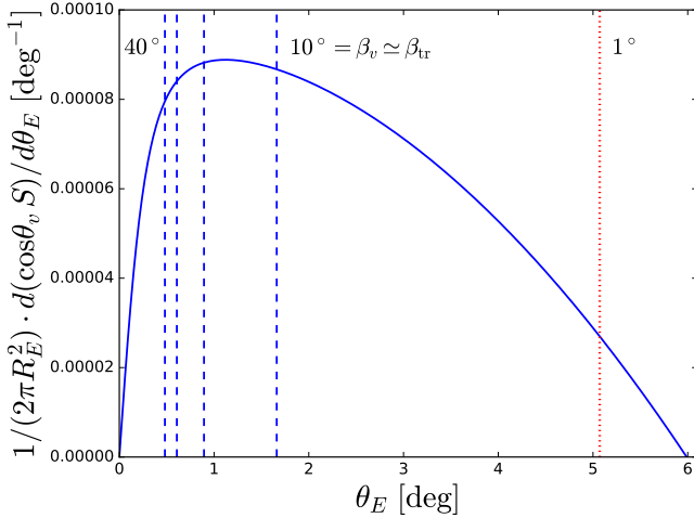
FIG. 11. The differential effective area S as a function of the co-latitude \theta_E of a point on the surface in view, for h = 35 km. The blue vertical dashed lines, from left to right, show the corresponding \beta_v for \beta_v = 40^\circ , 30^\circ , 20^\circ and 10^\circ . The red dashed line corresponds to \beta_v = 1^\circ .
