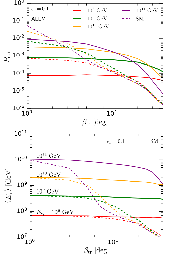
FIG. 6. Upper: Probabilities for fixed sterile neutrinos energies as a function of elevation angle, for an \epsilon_\nu = 0.1 sterile factor (solid lines) and for the standard model (dashed lines), using the ALLM model for photonuclear energy loss of the tau. Lower: The average energy of the emerging tau for sterile neutrinos with \epsilon_\nu = 0.1 and the standard model.
