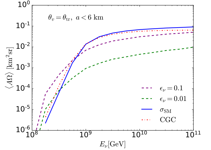
FIG. 8. The effective aperture for standard model tau neutrinos and sterile neutrinos with \sigma = \epsilon_\nu \sigma_{\text{SM}} , with \epsilon_\nu = 0.1 and the ALLM energy loss model. Also shown is the acceptance with a modified neutrino cross sections according to the color glass condensate model (CGC).
