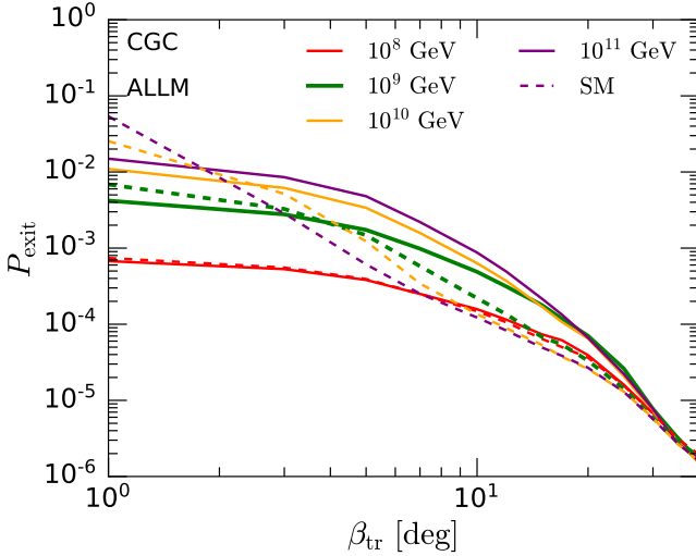
FIG. 5. The probability for a tau to exit for fixed E_{\nu_\tau} = 10^8, 10^9, 10^{10} and 10^{11} GeV for the color glass condensate ultrahigh energy neutrino cross section extrapolation (solid lines) and for a parton distribution function evaluation of the cross section ( \sigma_{\text{SM}} , dashed lines), as in Fig. 4.
