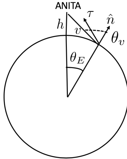
FIG. 1. Geometry of ANITA an altitude h above the surface of the Earth. The line of sight from the tau exit point at a co-latitude \theta_E has length v and makes an angle \theta_v relative to the local normal \hat{n} .
