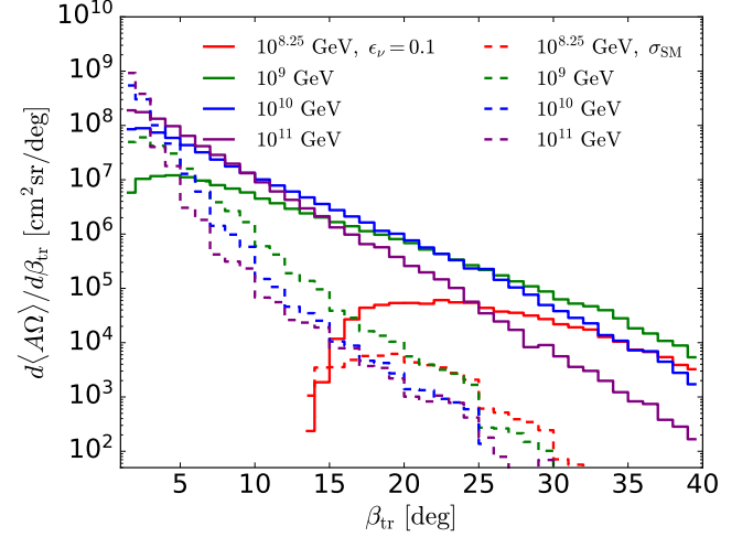
FIG. 9. The differential effective aperture as a function of \beta_{\text{tr}} for standard model tau neutrinos (dashed) and sterile neutrinos (solid) with \sigma = \epsilon_\nu \sigma_{\text{SM}} , \epsilon_\nu = 0.1 and the ALLM energy loss model.
