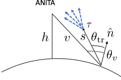
FIG. 2. The tau trajectory make an angle \theta_{\text{tr}} relative to the local normal \hat{n} . The tau decays a distance s along its trajectory. The figure is exaggerated to distinguish \theta_v and \theta_{\text{tr}} , however the effective Cherenkov angle of the signal from the tau decay shower is such that \theta_v \simeq \theta_{\text{tr}} .
