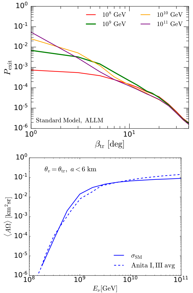
FIG. 4. Upper : The probability of a tau to exit for fixed E_{\nu_\tau} = 10^8, 10^9, 10^{10} and 10^{11} GeV in the standard model, as a function of elevation angle \beta_{tr} . The ALLM photonuclear energy loss is used. Lower : The standard model effective aperture compared with the mean effective aperture of Anita I,III [26] for upward-going tau air showers from incident \nu_\tau 's.
