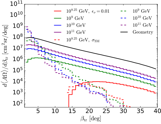
FIG. 10. The differential effective aperture as a function of \beta_{\text{tr}} for standard model tau neutrinos (dashed) and sterile neutrinos (solid) with \sigma = \epsilon_\nu \sigma_{\text{SM}} , \epsilon_\nu = 0.01 and the ALLM energy loss model. The curve labeled “Geometry” shows the rescaled differential aperture when P_{\text{exit}} = P_{\text{obs}} = 1 .
