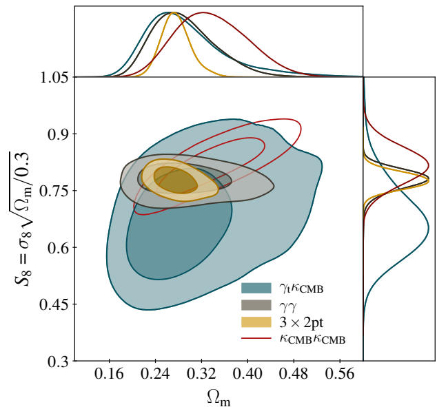
FIG. 6. Constraints on \Omega_m and S_8 from \gamma_t^{\kappa_{CMB}} , DES cosmic shear measurement [11], DES 3 \times 2pt measurement [12] and Planck \kappa_{CMB}^{\kappa_{CMB}} measurement [9].
