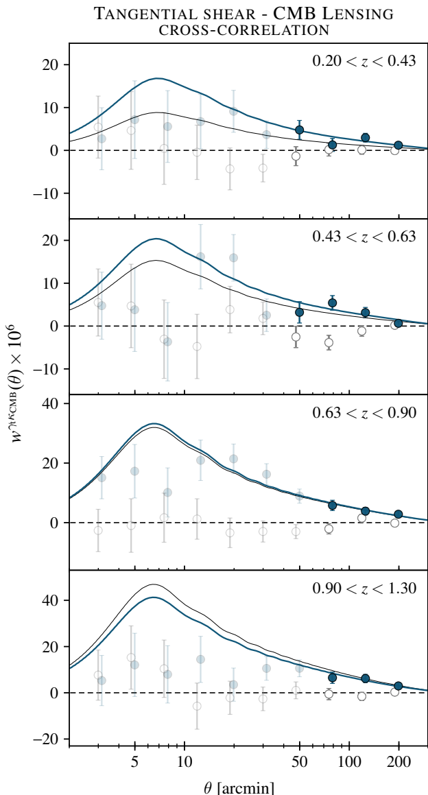
FIG. 2. Measurements of w^{\gamma t K_{CMB}}(\theta) (filled circles) and w^{\gamma \times K_{CMB}}(\theta) (open circles) using METACALIBRATION shear estimates and the SPT+ Planck CMB lensing map. The four panels show results for the four source galaxy redshift bin. Faded points are removed from the final analysis due to systematics or uncertainties in the modeling. Also shown are the theoretical predictions using fiducial cosmology with A = 1 (black), and with best-fit A (blue), where A is defined in Sec. VI A.
