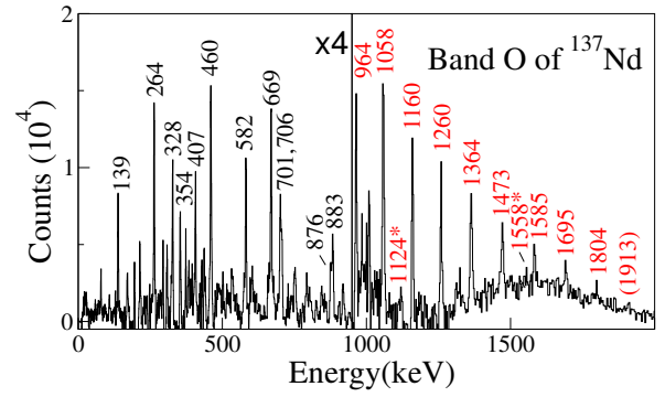
FIG. 2. Spectrum constructed by double-gating on the observed transitions of band O of ^{137}\text{Nd} . The in-band transitions are marked with red labels, while the low-lying transition are marked in black. Possible decay-out transitions are marked by an asterisk. The levels de-excited by the 328-, 407- and 876-keV transitions are fed by pathways which can be found in Ref. [22].
