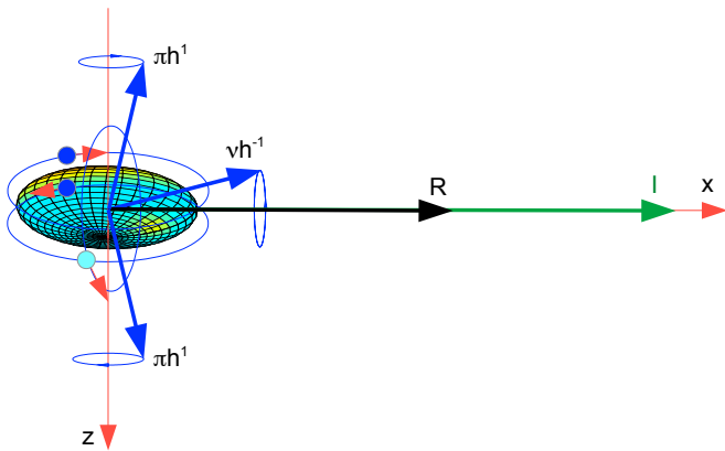
FIG. 7. Angular momentum composition of band O. The h_{11/2} orbitals are represented by their individual j -vectors. The sum of the contributions of the normal-parity orbitals, which are not shown in the figure, is denoted by R . The total angular momentum, I , is the sum of the projections on the rotational ( x -) axis.
