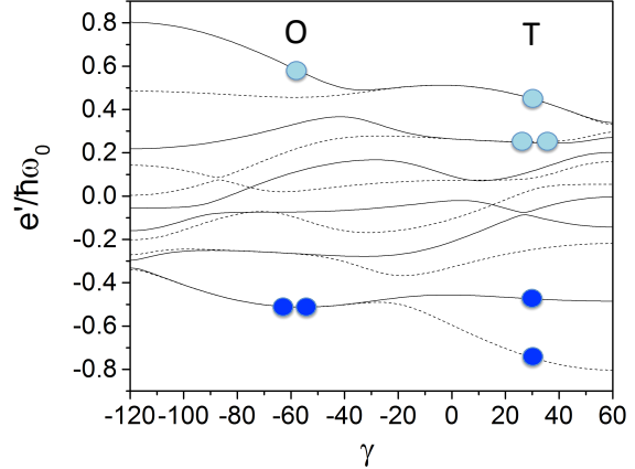
FIG. 6. Single-particle Routhians of the h_{11/2} shell as function of the triaxiality parameter \gamma for the j -shell model of Ref. [25]. The shown case corresponds to the bottom of band O and the middle of band T. The rotational frequency is \hbar\omega = 0.45 MeV and the energy scale is \hbar\omega_0 = 8 MeV. Full line: favored signature, dashed line: unfavored signature (respectively, -1/2 and 1/2 for h_{11/2} ), blue circles: protons, cyan circles: neutron holes.
