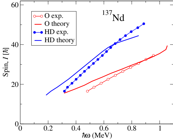
FIG. 4. Angular momentum as function of the rotational frequency \hbar\omega = (E(I) - E(I - 2))/2 of bands O and HD.
