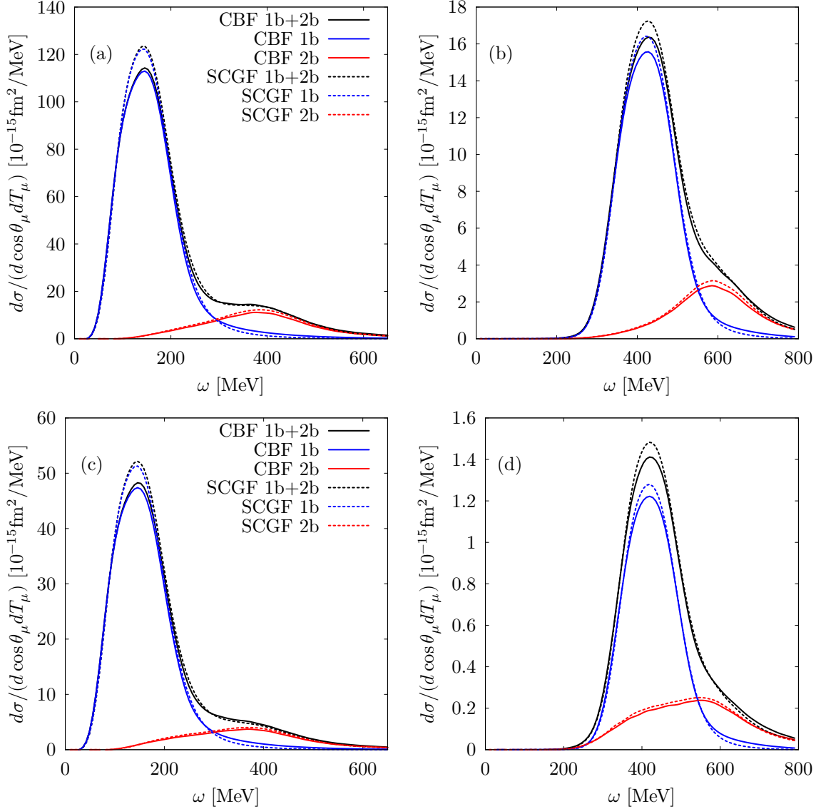
FIG. 4. Panels (a) and (b) correspond to the CC inclusive differential cross section of \nu_\mu scattering on ^{16}\text{O} for E_\nu=1 GeV and \theta_\mu = 30^\circ and 70^\circ , respectively. The blue (red) lines correspond to including only one-body (two-body) contributions in the CC reaction, while the black lines displays the total result. Dotted lines show results from the SF computed with the SCGF method and solid lines are from CBF. Panels (c) and (d) are the same as the upper but for \bar{\nu}_\mu scattering on ^{16}\text{O} .
