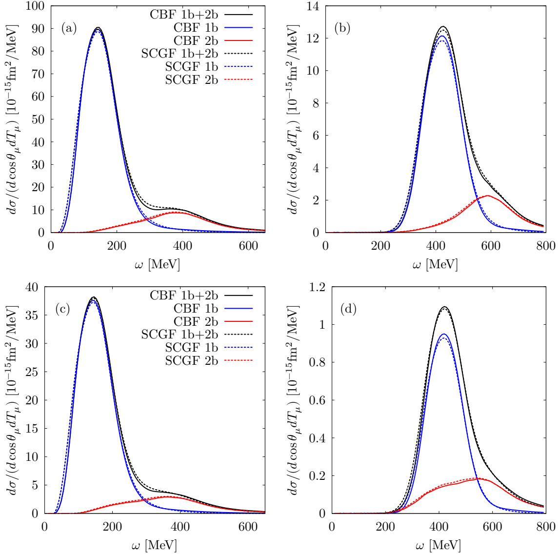
FIG. 3. Panels (a) and (b) correspond to the CC inclusive differential cross section of \nu_\mu scattering on ^{12}\text{C} for E_\nu=1 GeV and \theta_\mu = 30^\circ and 70^\circ , respectively. The blue (red) lines correspond to including only one-body (two-body) contributions in the CC reaction, while the black lines displays the total result. Dotted lines show results from the SF computed with the SCGF method and solid lines are from CBF. Panels (c) and (d) are the same as (a) and (b) but for \bar{\nu}_\mu scattering on ^{12}\text{C} .
