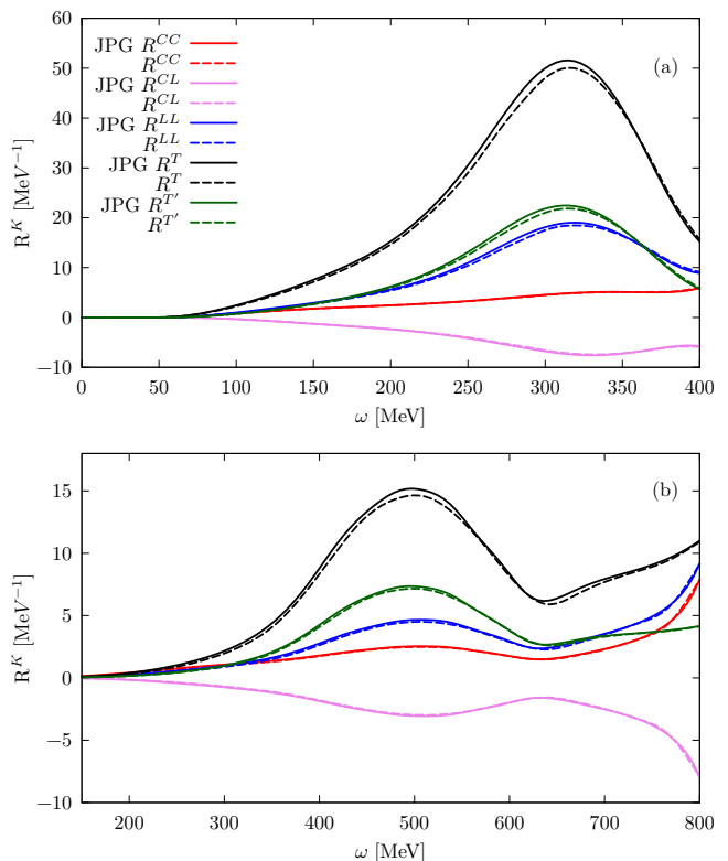
FIG. 2. Panel (a) and (b) display the two-body CC response functions of ^{12}\text{C} for |\mathbf{q}|=400 , and 800 MeV, respectively, obtained within the Relativistic Fermi gas model. We benchmark our results displayed by the dashed curves with those of Ref. [36] corresponding to the solid curves.
