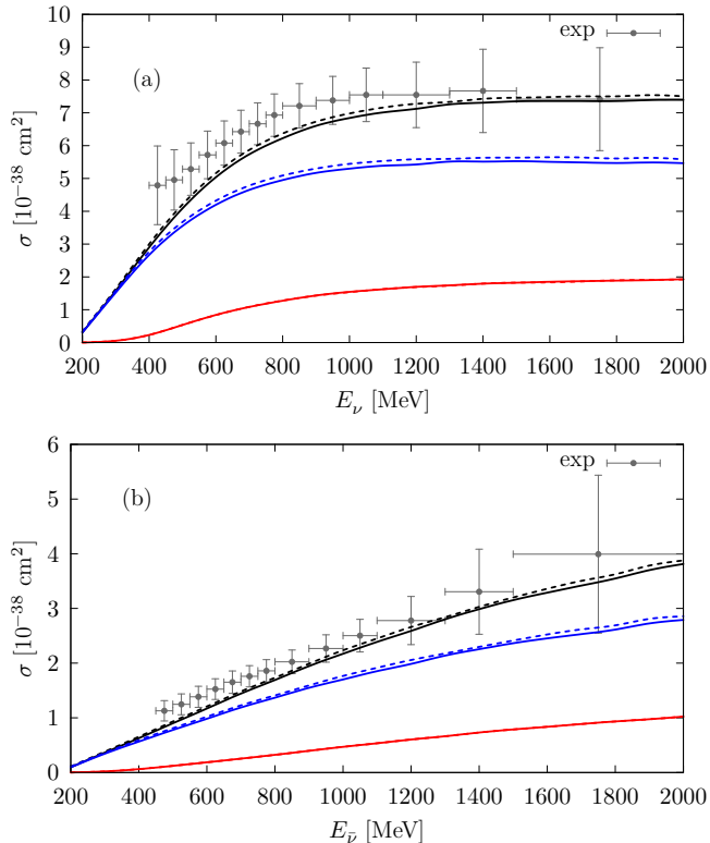
FIG. 7. Panels (a) and (b) display the CCQE \nu_{\mu} - and \bar{\nu}_{\mu} - ^{12}\text{C} total cross section per nucleon as a function of the neutrino energy, respectively. The blue (red) lines correspond to including only one-body (two-body) contributions in the CC reaction, while the black lines displays the total result. Dotted lines show results from the SF computed with the SCGF method and solid lines are from CBF. The MiniBooNE data points [42] are plotted as a function of the reconstructed neutrino energy.
