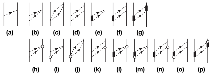
FIG. 1. OPE and TPE contributions at LO [(a)], NLO [(b)-(g)], and N2LO [(h)-(p)]. Nucleons, \Delta isobars, and pions are denoted, respectively, by the solid, thick-solid, and dashed lines; note that both direct and crossed box contributions are retained in diagrams (d), (f)-(g), (k), (n)-(p). The open circles denote \pi N and \pi N\Delta couplings from the sub-leading chiral Lagrangians \mathcal{L}_{\pi N}^{(2)} [36] and \mathcal{L}_{\pi N\Delta}^{(2)} [37].
