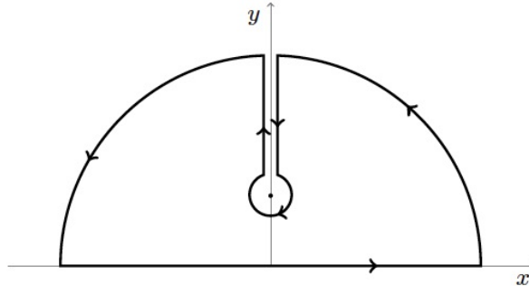
FIG. 4. Integration contour.
