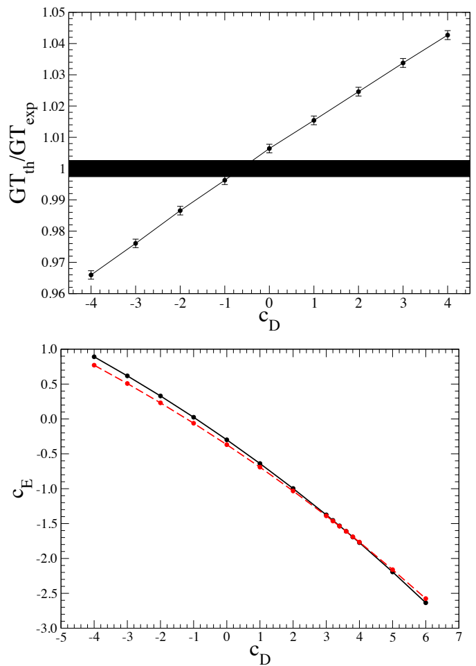
FIG. 3. Upper panel: The calculated ratio \text{GT}_{\text{th}}/\text{GT}_{\text{exp}} as function of c_D (solid line; each point on this line reproduces the trinucleon binding energies). Lower panel: The c_D - c_E trajectories obtained by fitting the experimental trinucleon binding energies (solid line) and nd doublet scattering length (dashed line) (the intercept of these two lines gives the c_D and c_E values that reproduce these two observables simultaneously). The NV2+3-Ia chiral interactions are used here for illustration. The values of 8.475 MeV and 7.725 MeV, and 0.645 \pm 0.010 fm [44] are used for the {}^3\text{H} and {}^3\text{He} binding energies, and nd scattering length, respectively. Note that these energies have been corrected for the small contributions (+7 keV in {}^3\text{H} and -7 keV in {}^3\text{He} ) due to the n - p mass difference [45]. The band (left panel) results from experimental uncertainty \text{GT}_{\text{EXP}} , which has conservatively been doubled.
