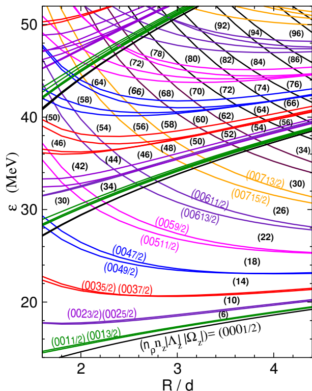
FIG. 2. (Color online) Single-particle energies for a toroidal nucleus as a function of the aspect ratio R/d . The states are labeled by quantum numbers (n_\rho, n_z, |\Lambda_z|, |\Omega_z|) which are displayed only for the lowest states. The locations of the toroidal shell are shown as bracketed numbers, (N) , at their corresponding toroidal deformations, R/d .
