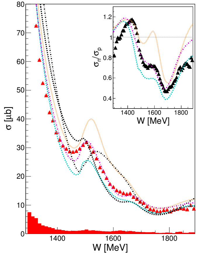
FIG. 28. Full red triangles: Total cross section as a function of the final state invariant mass for the free neutron (quasi-free neutron data corrected for FSI effects). Dashed cyan line: SAID, dotted orange line: MAID, dash-dotted magenta line: BnGa. The black dashed and dash-dotted lines show the results of the SAID and BnGa analysis previous to the results from the present work and [38]. The insert shows the ratio of the free neutron to the SAID proton (full black triangles).
