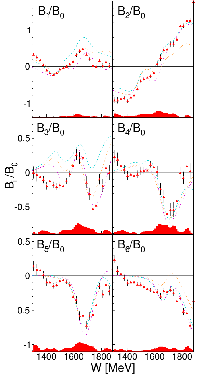
FIG. 30. Full red triangles: normalized Legendre coefficients as a function of the final state invariant mass for exclusive single \pi^0 photoproduction off the free neutron (quasi-free data corrected for FSI effects). Solid histograms: systematic uncertainties, dashed cyan curve: SAID, dotted orange curve: MAID, dash-dotted magenta curve: BnGa.
