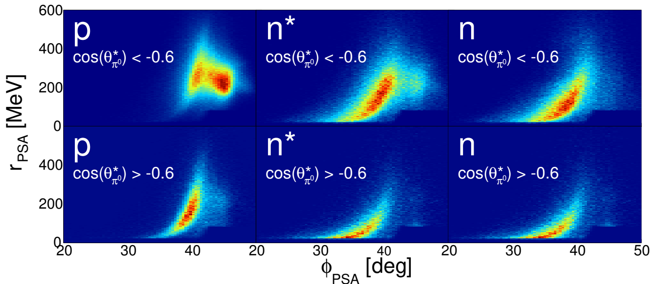
FIG. 9. PSA analysis of hits in the TAPS detector for nucleon candidates for events with forward and backward pion angles. Plotted is the PSA radius ( r_{\text{PSA}} versus the PSA angle ( \phi_{\text{PSA}} ). Left column: proton, center column: neutron without ToF-versus-energy cut, right column: neutron with ToF-versus-energy cut. Top row: \cos(\theta_{\pi^0}^*) < -0.6 , bottom row: \cos(\theta_{\pi^0}^*) > -0.6 .
