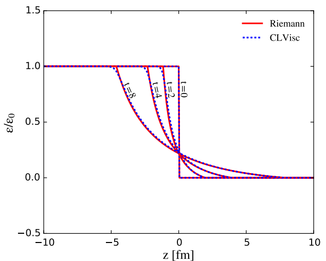
Figure 5. (color online) The comparison between CLVisc and Riemann solution for energy density evolution as a function of time.
