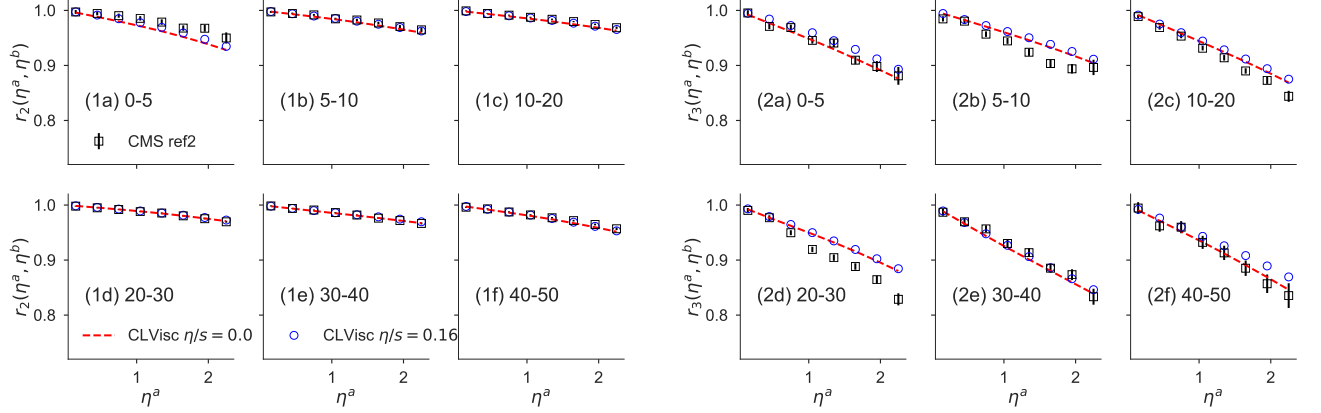
Figure 22. (color online) The decorrelation of elliptic flow (1a)-(1f) and triangular flow (2a)-(2f) along the pseudo-rapidity direction, for Pb+Pb \sqrt{s_{NN}} = 2.76 TeV collisions with centrality range 0-5, 5-10, 10-20, 20-30, 30-40 and 40-50, from (3+1)D viscous hydrodynamic simulations starting from AMPT initial conditions without the initial fluid velocity ( \eta_v/s = 0 for red lines and \eta_v/s = 0.16 for blue circles and stars) as compared with LHC measurements at CMS (black squares). The “ref2” denotes 4.4 < \eta^b < 5.0 , used in both CMS data and CLVisc calculation.
