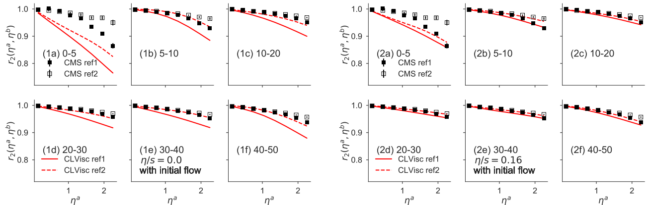
Figure 23. (color online) The decorrelation of elliptic flow along the pseudo-rapidity direction, for Pb+Pb \sqrt{s_{NN}} = 2.76 TeV collisions with centrality range 0-5, 5-10, 10-20, 20-30, 30-40 and 40-50, from (3+1)D viscous hydrodynamic simulations starting from AMPT initial conditions with the initial fluid velocity ( \eta_v/s = 0 for (1a)-(1f) and \eta_v/s = 0.16 for (2a)-(2f)) as compared with LHC measurements at CMS (black squares). The “ref1” denotes 3.0 < \eta^b < 4.0 while “ref2” denotes 4.4 < \eta^b < 5.0 .
