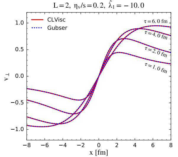
Figure 9. (color online) The time evolution of transverse fluid velocity from CLVisc numerical results (solid) and Gubser analytical solution (dashed) for 2nd order viscous hydrodynamics.
