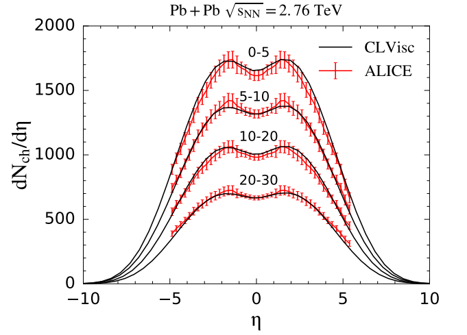
Figure 17. (color online) Pseudo-rapidity distribution for charged hadrons in Pb+Pb collisions at \sqrt{s_{NN}} = 2.76 TeV with centrality range 0–5%, 5–10%, 10–20% and 20–30%, from CLVisc (solid-lines) and LHC experimental data by ALICE collaboration [115].
