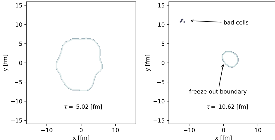
Figure 1. (color online) The space-time coordinates of bad cells where \max(|\pi^{\mu\nu}|) > T_0^{\tau\tau} , from one testing event in \sqrt{s_{NN}} = 200 GeV Au+Au collisions at 0-10% centrality. The bad cells in this event appear at \tau \sim 10.62 fm with spatial coordinates far away from the freeze out boundary.
