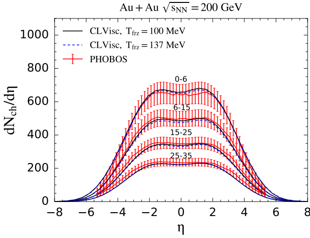
Figure 15. (color online) Pseudo-rapidity distribution for charged hadrons in Au+Au collisions at \sqrt{s_{NN}} = 200 GeV with centrality range 0–6%, 6–15%, 15–25% and 25–35%, from CLVisc with freeze-out temperature 100 MeV (solid-lines) and 137 MeV (dashed lines) as compared with RHIC experimental data by PHOBOS collaboration [115].
