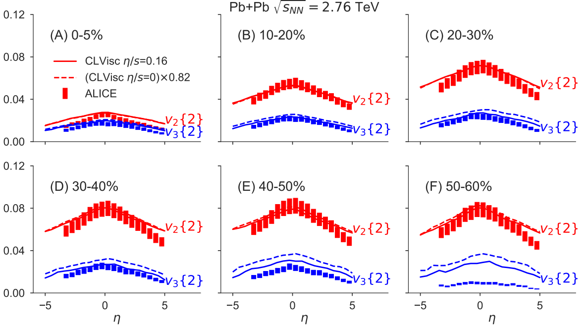
Figure 20. The pseudo-rapidity dependence of elliptic flow and triangular flow, for Pb+Pb \sqrt{s_{NN}} = 2.76 TeV collisions with centrality range 0-5, 10-20, 20-30, 30-40, 40-50 and 50-60, from (3+1)D viscous hydrodynamic simulations starting from AMPT initial conditions without initial fluid velocity and evolve with \eta_v/s = 0.16 as compared with LHC measurements from ALICE collaboration [119].
