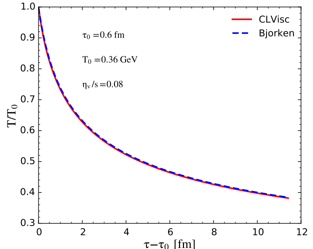
Figure 7. (color online) The comparison between CLVisc and Bjorken solution for viscous hydrodynamics
