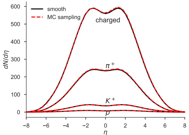
Figure 3. (color online) Pseudo-rapidity distributions for charged hadrons and identified particles \pi^+ , K^+ and proton from smooth particle spectra (black solid line) with integral resonance decay and Monte Carlo sampling (red dashed line) with forced resonance decay. The hydrodynamic evolution is given by CLVisc with optical Glauber initial condition at impact-parameter b = 2.4 fm, with initial time \tau_0 = 0.4 fm, the maximum energy density in most central collisions \epsilon_{\text{max}} = 55 GeV/fm 3 and lattice QCD EoS from Wuppertal-Budapest 2014 computation.
