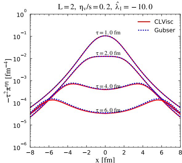
Figure 11. (color online) The time evolution of -\tau^2 \pi^{\eta_s \eta_s} from CLVisc numerical results and Gubser analytical solution for 2nd order viscous hydrodynamics.
