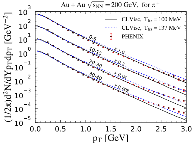
Figure 16. (color online) Invariant yield of \pi^+ in Au+Au collisions at \sqrt{s_{NN}} = 200 GeV with centrality range 0–5%, 10–15%, 20–30% and 30–40%, from CLVisc with freeze-out temperature 100 MeV (solid-lines) and 137 MeV (dashed lines) as compared with RHIC experimental data by PHENIX collaboration.
