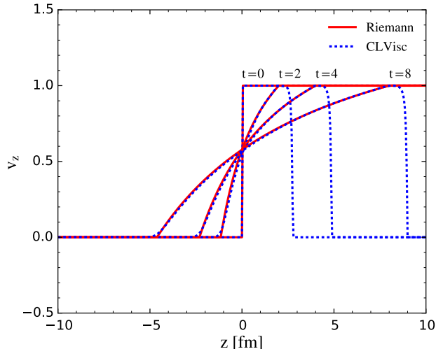
Figure 6. (color online) The comparison between CLVisc and Riemann solution for fluid velocity evolution as a function of time.
