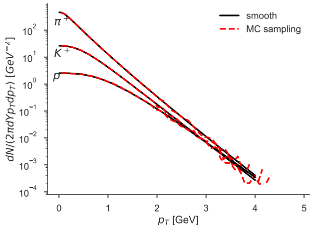
Figure 4. (color online) The transverse momentum distribution for identified particles \pi^+ , K^+ and proton from smooth particle spectra (black solid line) with integral resonance decay and Monte Carlo sampling (red dashed line) with forced resonance decay. The hydrodynamic evolution is the same as in Fig. 3.
