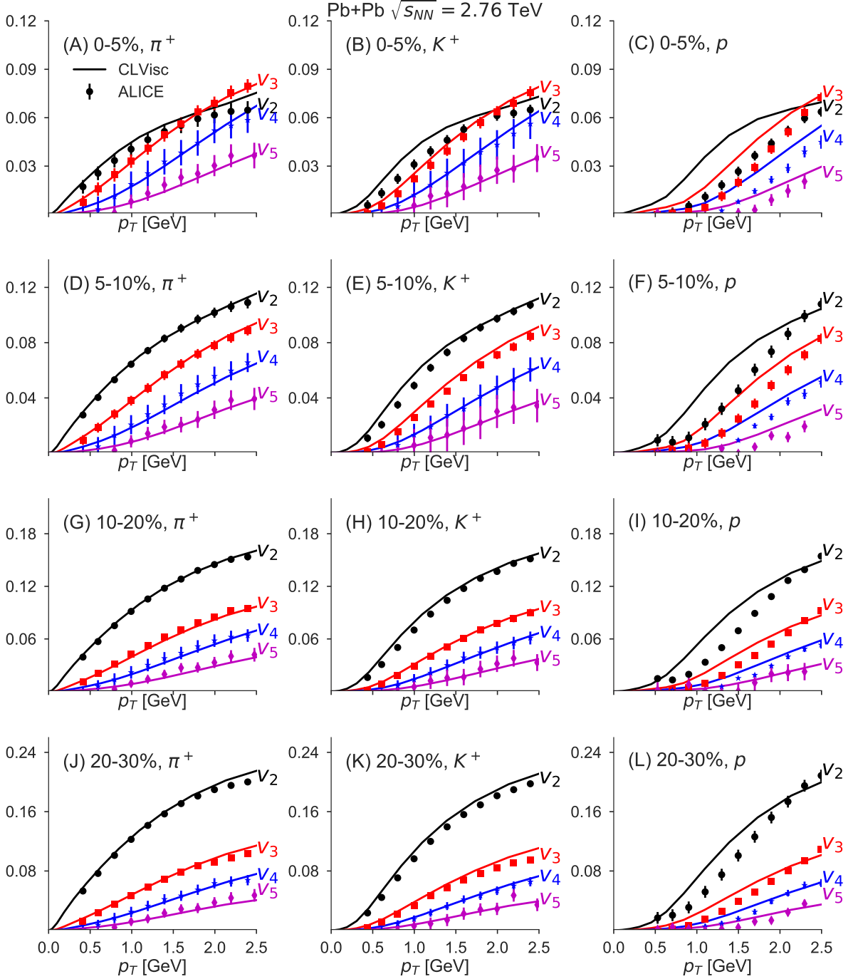
Figure 19. (color online) The centrality dependence of the anisotropic flows v_2 , v_3 , v_4 and v_5 from scalar-product method in Pb+Pb collisions at \sqrt{s_{NN}} = 2.76 TeV with centrality ranges 0–5%, 5–10%, 10–20% and 20–30%, from CLVisc (solid-lines) and LHC experimental data (markers) by ALICE collaboration [118].
