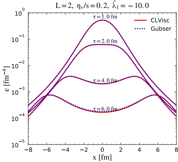
Figure 8. (color online) The time evolution of energy density distribution from CLVisc numerical results (solid) and Gubser analytical solution (dashed) for 2nd order viscous hydrodynamics.
