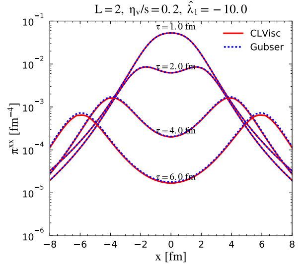
Figure 10. (color online) The time evolution of \pi^{xx} from CLVisc numerical results and Gubser analytical solution for 2nd order viscous hydrodynamics.
