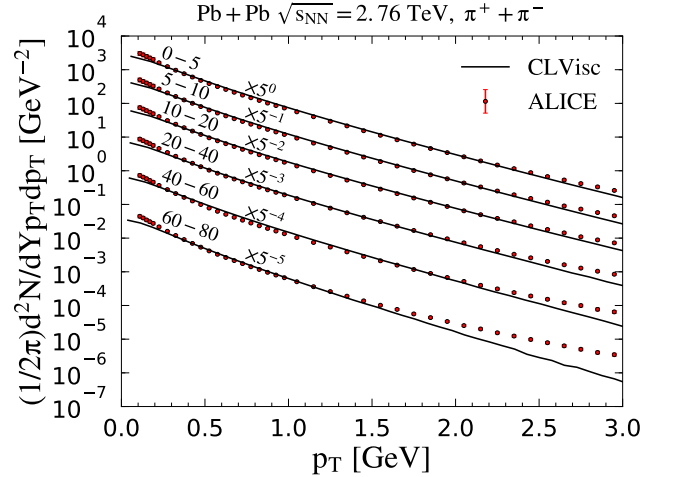
Figure 18. (color online) p_T spectra of charged pions for Pb+Pb \sqrt{s_{NN}} = 2.76 TeV collisions at centrality range 0–5%, 5–10%, 10–20%, 20–40%, 40–60%, 60–80%, from CLVisc (solid-lines) and LHC experimental data by ALICE collaboration [116].
