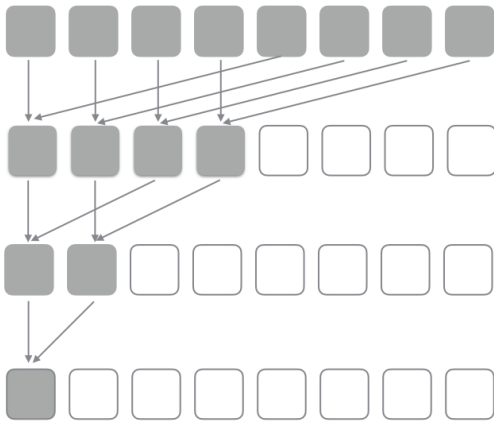
Figure 27. Parallel reduction used on GPU to compute the summation of particle spectra from millions of freeze-out hyper-surface elements.
