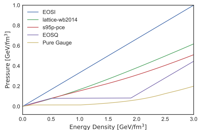
Figure 2. (color online) Pressure as a function of energy density for 5 different equations of state. They are denoted as EOSI, lattice-wb2014, s95p-pce, EOSQ and pure gauge from top to down.
