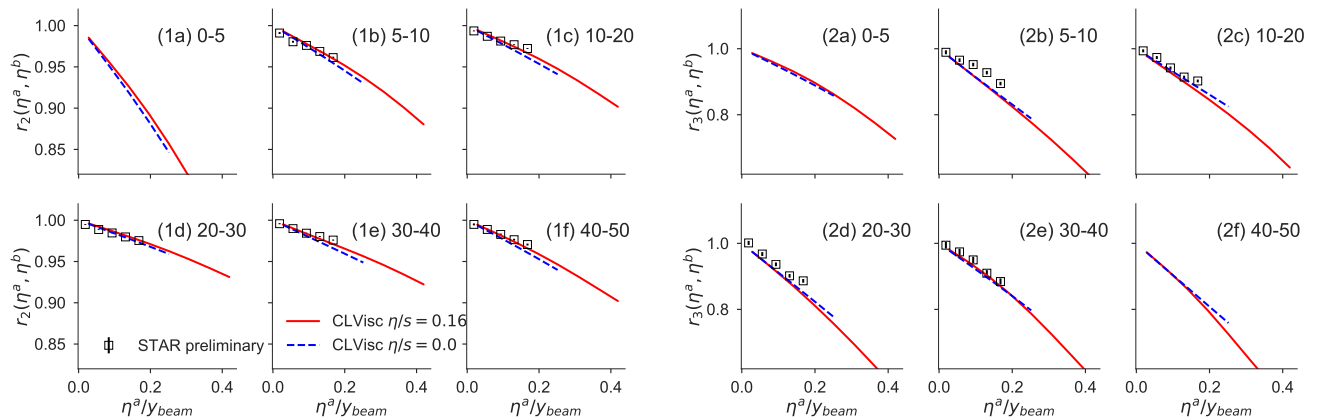
Figure 24. (color online) The decorrelation of elliptic flow (1a)-(1f) and triangular flow (2a)-(2f) along the pseudo-rapidity direction, for Au+Au \sqrt{s_{NN}} = 200 GeV collisions with centrality range 0-5, 5-10, 10-20, 20-30, 30-40 and 40-50, from (3+1)D viscous hydrodynamic simulations starting from AMPT initial conditions ( \eta_v/s = 0.16 for red solid lines and \eta_v/s = 0 for blue dashed lines) as compared with preliminary STAR measurements at RHIC (black squares). The reference rapidity window is 2.5 < \eta^b < 4.0 and y_{beam} = 5.36 for Au+Au \sqrt{s_{NN}} = 200 GeV collisions.
