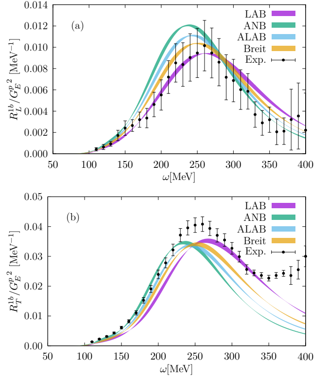
FIG. 3. Frame dependence of the GFMC longitudinal (a) and transverse (b) electromagnetic response functions of {}^4\text{He} at |\mathbf{q}|=700 MeV.
