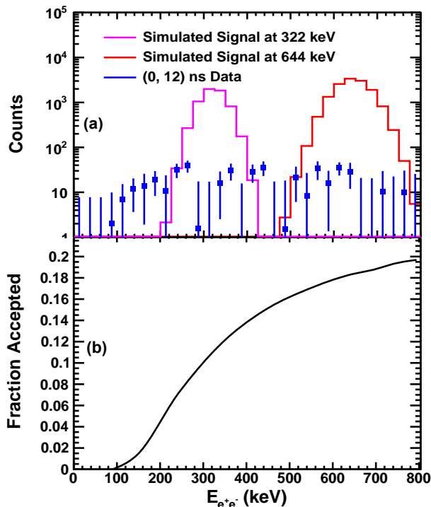
Figure 4. (a) Background-subtracted e^+e^- pair kinetic energy spectra for events in the analysis time-window. For comparison, simulated positive dark matter decay signals at 322 keV, 644 keV are overlaid. (b) Total e^+e^- pair acceptance (see text) as a function of summed kinetic energy.
