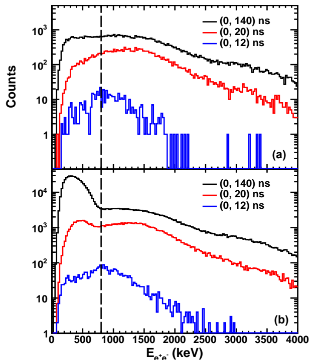
Figure 3. Energy spectrum of (a) background and (b) foreground runs, for three separate time-windows. Clear structure of a neutron \beta -decay backscattering peak at 300 keV is visible for time-windows > 12 ns in the foreground runs. Dashed lines at 0 keV, 800 keV indicate the energy region of interest used for the present analysis.
