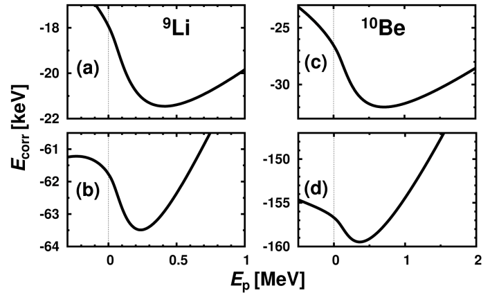
FIG. 3. The continuum-coupling correlation energy as a function of proton energy E_p for: (a) J^\pi = 1/2^+ ; T = 3/2 SM states with an excitation energy E^* < 15 MeV coupled in s -wave to the (lowest) one-proton decay channel and (b) with the additional coupling to all one-neutron decay channels, (c) {}^{10}\text{Be}^* for the J_n^\pi = 2_{12}^- ; T = 1 state considering all J^\pi = 2^- ; T = 1 SM states with an excitation energy E^* < 22 MeV s -wave coupled to the (lowest) one-proton decay channel and (d) with the addition of coupling to 9 neutron-decay channels.
