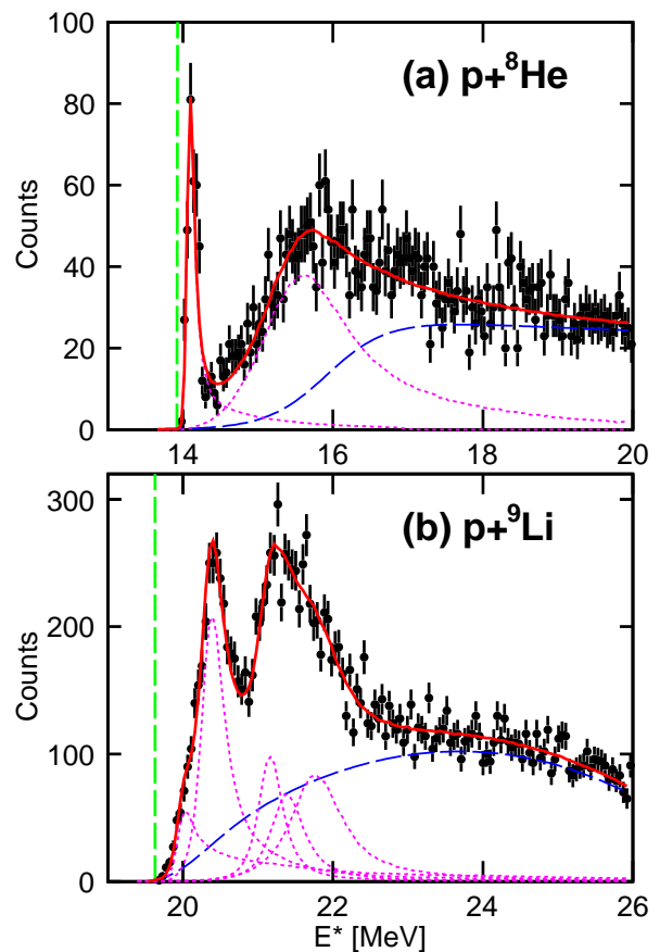
FIG. 1. (Color online) Invariant-mass reconstructions of (a) {}^9\text{Li}^* and (b) {}^{10}\text{Be}^* from the indicated decay channels. The vertical lines are the proton-decay thresholds (13.944 and 19.636 MeV) and the dotted (dashed) curves indicate the fitted states (backgrounds).
