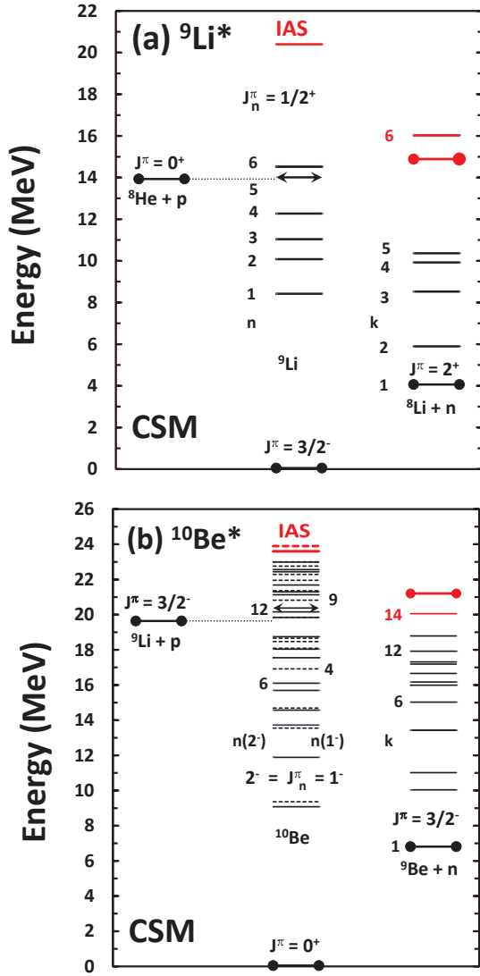
FIG. 2. (color online) Continuum-shell-model level diagrams for relevant (a) {}^9\text{Li}^* and (b) {}^{10}\text{Be}^* resonances. All shown levels are coherently coupled in the SMEC calculations. The black (red) lines indicate T_{<} ( T_{>} ) levels, lines with end points are experimental levels and those with arrows indicate the lowest-lying levels with a significant proton-decay branch. The {}^9\text{Li} levels of J^\pi = 1/2^+ , {}^{10}\text{Be} levels with J^\pi = 2^- (solid lines) and 1^- (dashed lines), the ground-state proton decay channel and the relevant n-decay channels are all indicated. The wave-function compositions are provided in the supplementary tables that are organized by the indices n and k [36].
