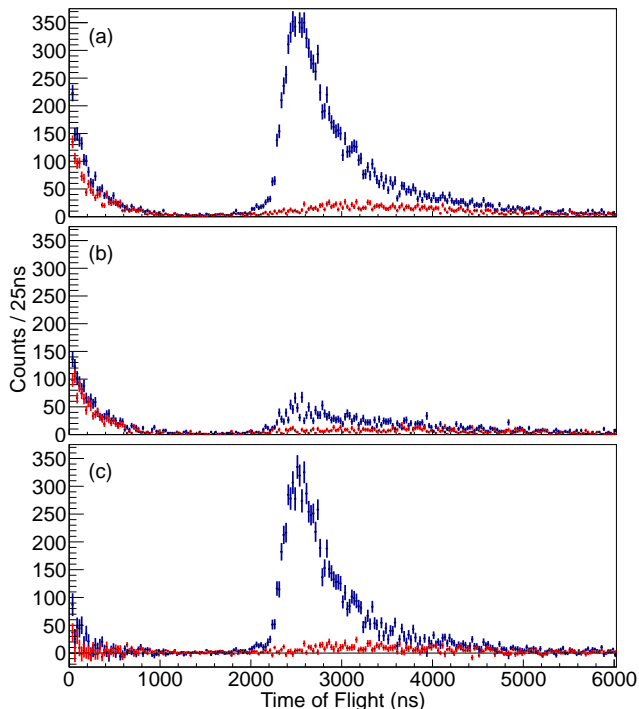
FIG. 3: (Color Online) Time-of-flight spectrum for \beta -ion coincidences for (a) the ^{134}\text{Sb} -optimized measurement cycle, (b) the ^{134m}\text{Sb} -optimized measurement cycle scaled to have the same ^{134m}\text{Sb} decay contribution as in the ^{134}\text{Sb} -optimized measurements (as described in the text), and (c) the ^{134}\text{Sb} spectrum obtained by subtracting the ^{134m}\text{Sb} contribution. The data collected with the \Delta E -MCP detector pairs separated by 180^\circ (left \Delta E with right MCP and bottom \Delta E with top MCP) are shown in blue while the data for detector pairs separated by 90^\circ (left \Delta E with top MCP and bottom \Delta E with right MCP) are shown in red.
