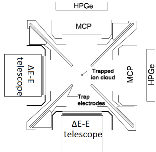
FIG. 2: A cross-sectional view of the BPT and the detector array used in this work, not to scale. The beam axis points out of the page, and the detectors are identified according to their positioning relative to this axis. In the left and bottom positions are the two \Delta E -E plastic-scintillator detectors used for \beta -particle detection, and in the right and top positions are two MCP detectors and two HPGe detectors used for recoil-ion and \gamma -ray detection, respectively.
