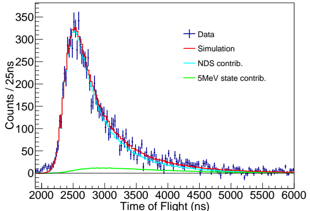
FIG. 7: (Color Online) The TOF spectrum for \beta -ion coincidences compared to simulations (red) which include the decay scheme from the Nuclear Data Sheets [16] with a_{\beta\nu} = 1 (cyan) and a single fictitious allowed Gamow-Teller transition with a_{\beta\nu} = -1/3 to a 5-MeV excited state (green) which decays directly to the ground state by a single \gamma ray.
