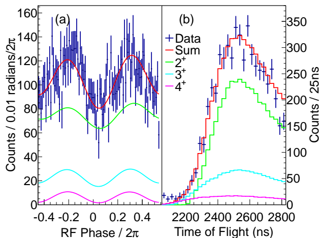
FIG. 4: (Color Online) (a) The RF-phase dependence of \beta -ion coincidences from the decay of ^{134}\text{Sb} . The best fit (red) from simulations consists of the sum of 2^+ (green), 3^+ (cyan), and 4^+ (magenta) contributions. (b) The resulting TOF spectra from the charge-state distribution determined from the RF phase, confined to 2000 to 2800 ns to illustrate the low TOF behavior of the charge states.
