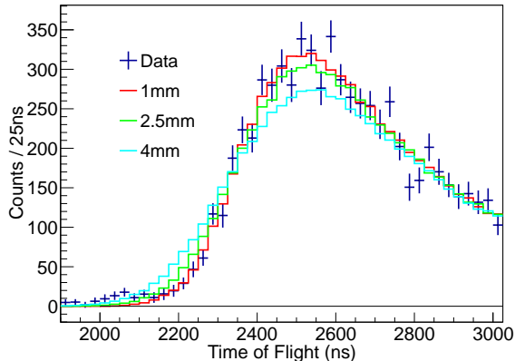
FIG. 5: (Color Online) The rising edge of the ^{134}\text{Sb} decay TOF compared with three simulated cloud sizes, labeled by the FWHM of the Gaussian distribution used. The 1 mm (red) simulation is scaled to match counts between 2400–2600 ns, and the 2.5 mm (green) and 4 mm (cyan) are shown with the same number of \beta -ion coincidences as the 1 mm simulation.
