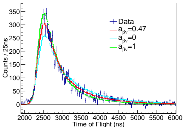
FIG. 6: (Color Online) The measured ^{134}\text{Sb} TOF spectrum compared to simulations using the decay scheme in Ref. [16] with different a_{\beta\nu} values. The value which matches R_{180/90}=9.33 from the data is a_{\beta\nu}=0.47 and the resulting TOF distribution is shown in red. The TOF spectra for a_{\beta\nu}=0 (cyan) and a_{\beta\nu}=1 (green) are also shown and result in R_{180/90} values that are inconsistent with the data.
