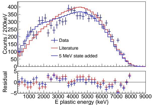
FIG. 8: (Color Online) The \beta -energy spectrum for \beta -ion coincidences compared to simulations which include the decay scheme from the Nuclear Data Sheets [16] with a_{\beta\nu} = 1 (red) combined with a single fictitious allowed Gamow-Teller transition with a_{\beta\nu} = -1/3 to a 5-MeV (blue) excited state which decays directly to the ground state by a single \gamma ray, scaled to match counts above 200 keV.
