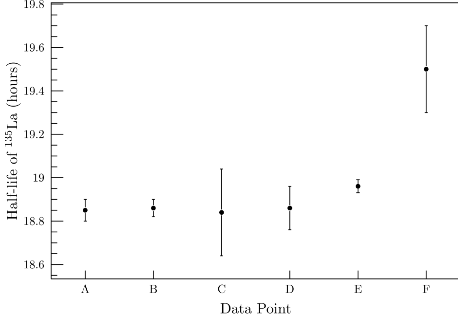
FIG. 3. Plot showing the 5 measurements for the half-life of ^{135}\text{La} in this work and the Nuclear Data Sheet value. Data points A-E are the half-lives measured using the 480.5 keV peak in Data Set 2, the 480.5 keV peak in Data Set 1, the 874.5 keV peak in Data Set 2, the 874.5 keV peak in Data Set 1, and the ionization chamber measurement, respectively. Data point F is the previously accepted value in NDS.
