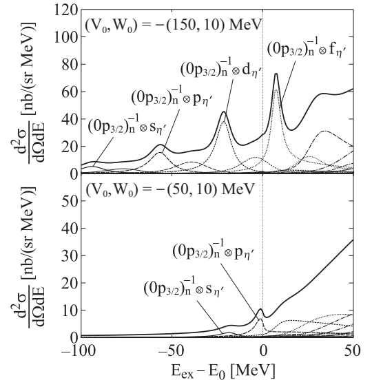
FIG. 10. Theoretically-calculated spectra of the ^{12}\text{C}(p, d)^{11}\text{C} \otimes \eta' reaction at 2.5 GeV [29]. The \eta' -nucleus potential parameters are taken as (V_0, W_0) = (-150, -10) MeV (top) and (-50, -10) MeV (bottom). Total formation cross sections are shown by the thick lines, and major configurations of the \eta' -mesic states \ell_{\eta'} coupling with the neutron hole states (nl_j)_n^{-1} are shown by the thin lines.
