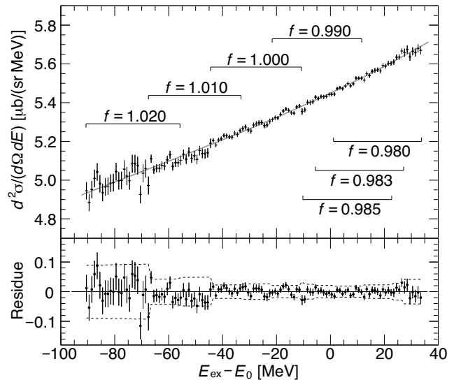
FIG. 8. (Top panel) Combined spectrum of the ^{11}\text{C} excitation energy E_{\text{ex}} near the \eta' production threshold E_0 = 957.78 MeV. A third-order polynomial fit is given by the solid gray curve. The horizontal bars indicate excitation-energy regions covered by each FRS momentum setting. (Bottom panel) Residues of the polynomial fit. The dashed lines display envelopes of 2 standard deviations.
