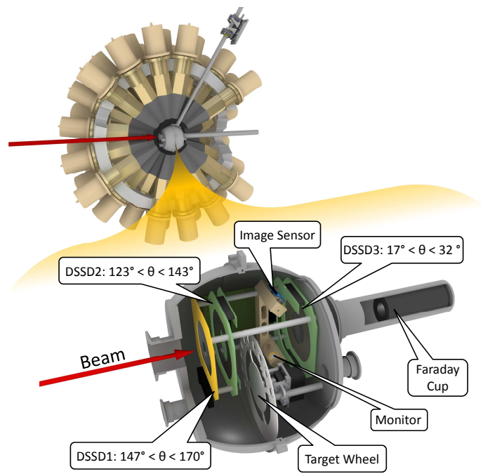
FIG. 2: (Color online) A schematic drawing of the experimental setup showing the spherical target chamber mounted in the middle of the Gammasphere array.
