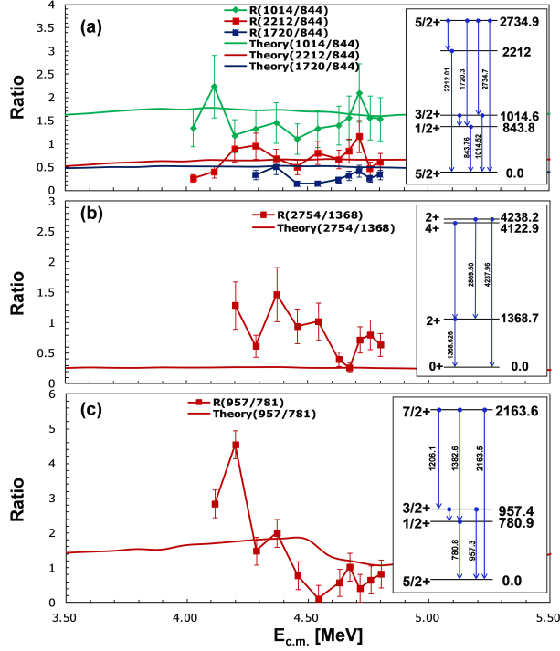
FIG. 10: The relative \gamma strengths of the observed transitions with respect to the strength of the ground state transition of the first excited state associated with the proton (a), alpha (b), and neutron (c) channels are shown (symbols). Also shown for comparison are the ratios obtained from the SAPHIRE calculations (solid lines).
