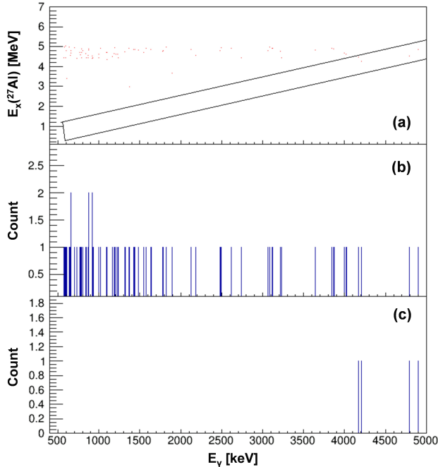
FIG. 7: Beam-induced coincident background taken with the same target at a much lower beam energy E_{beam}=7.0 MeV is shown. The top panel (a) displays coincidence events for protons and \gamma rays, equivalent E_x(^{27}\text{Al}) versus E_\gamma . Panel (b) shows the projection of E_\gamma for all coincident events. Panel (c) shows the projection of E_\gamma for the coincident events inside the black-box cut indicated in (a). This corresponds to the \gamma transitions under the same gate as in Fig. 5, i.e., equivalently for direct decays from the excited states (with excitation energy up to about 5 MeV) in ^{27}\text{Al} to the ground state.
