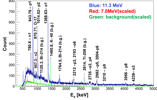
FIG. 5: The HPGe \gamma -ray spectra taken at E_{beam}=11.3 MeV (blue) compared with a beam-induced background spectrum at 7.0 MeV (red), and a room background measurement (green). The \gamma energies and the related particle (n, p, and \alpha ) emission channels are labeled for primary \gamma transitions in ^{12}\text{C}+^{16}\text{O} . Some of the pronounced background lines are labeled as well.
