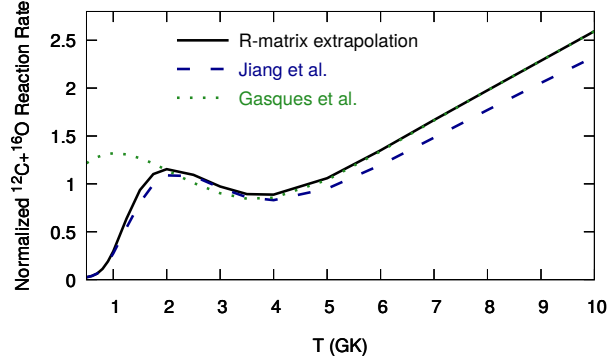
FIG. 14: The reaction rate for the ^{12}\text{C}+^{16}\text{O} fusion is shown for both the calculations using the Sao Paulo potential [2, 41] (dotted line) and a hindrance model fit [7] (dashed line) of the data, normalized to the standard rate of Caughlan and Fowler [45]. An R-matrix-extrapolation rate (solid line) using the R-matrix fit of the data with high energy extrapolation from the Sao Paulo calculations [2, 41] and low energy extrapolation from the hindrance model fit [7] is also shown.
