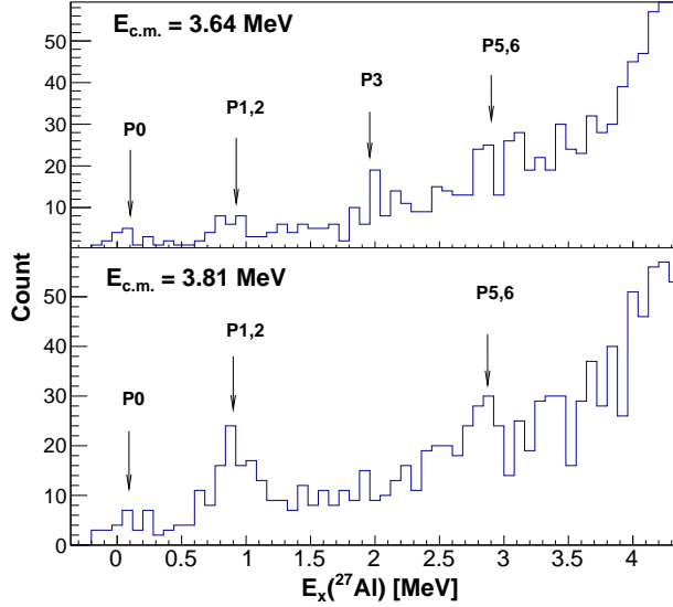
FIG. 4: Proton spectra of ^{12}\text{C}(^{16}\text{O}, p)^{27}\text{Al} reaction are shown for lower energies at E_{c.m.} = 3.64 MeV (top panel) and E_{c.m.} = 3.81 MeV (bottom panel), respectively. Observed proton groups are labeled as p_i , representing the protons populating ^{27}\text{Al} at the i th excited state. The rising trend at the high excitation energy end shows the low energy tail of detected signals contributed from background and noises.
