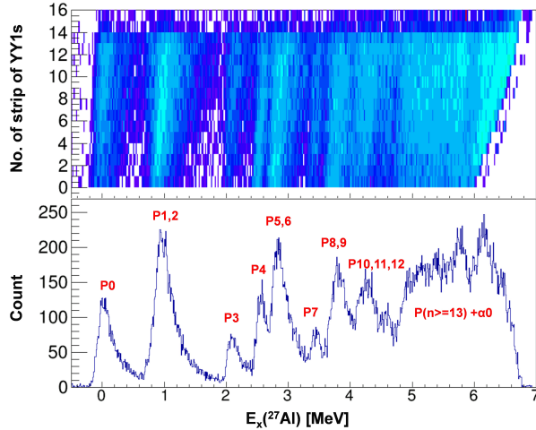
FIG. 3: Proton spectrum of ^{12}\text{C}(^{16}\text{O}, p)^{27}\text{Al} reaction taken by YY1s at E_{beam}=11.3 MeV. The top panel shows the raw spectrum of YY1s for the different strips versus excitation energies in ^{27}\text{Al} . The bottom panel shows the projection of E_x(^{27}\text{Al}) . Different proton groups are identified and labeled as p_i , representing the protons populating ^{27}\text{Al} at the i th excited state. Some of the very energetic alpha particles from the \alpha_0 channel can leak into the proton group of p_{13} and above where the signals are just above the detection threshold of the silicon detectors.
