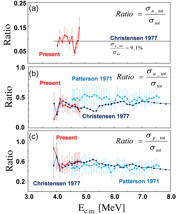
FIG. 12: The ratios of the cross sections of three particle emission channels (n, \alpha and p) to the total ^{16}\text{O}+^{12}\text{C} fusion cross section are shown in panels (a), (b), and (c), respectively. Previous data [16, 17] on the p and \alpha channels are shown for comparison. For the n channel, a flat ratio of 9% was used in the data of Christensen et al. [16].
