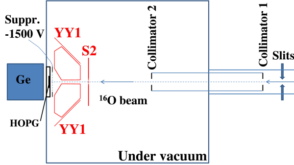
FIG. 2: The experimental setup showing the location of the charged particle as well as the \gamma detectors. The ^{16}\text{O} beam direction is from right to left with scattering being suppressed by a set of collimators and slits. Six YY1-type and one S2-type silicon detectors were used for the detection of charged particles. One HPGe / NaI was placed immediately after the HOPG target for measuring gamma rays.
