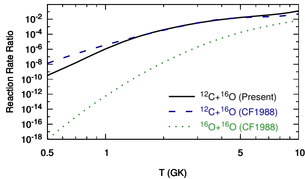
FIG. 15: The past [45] (dashed line) and present (solid line) reaction rates of ^{12}\text{C}+^{16}\text{O} , as well as the rate of ^{16}\text{O}+^{16}\text{O} [45] (dotted line), are shown as normalized to that of ^{12}\text{C}+^{12}\text{C} fusion [45].
