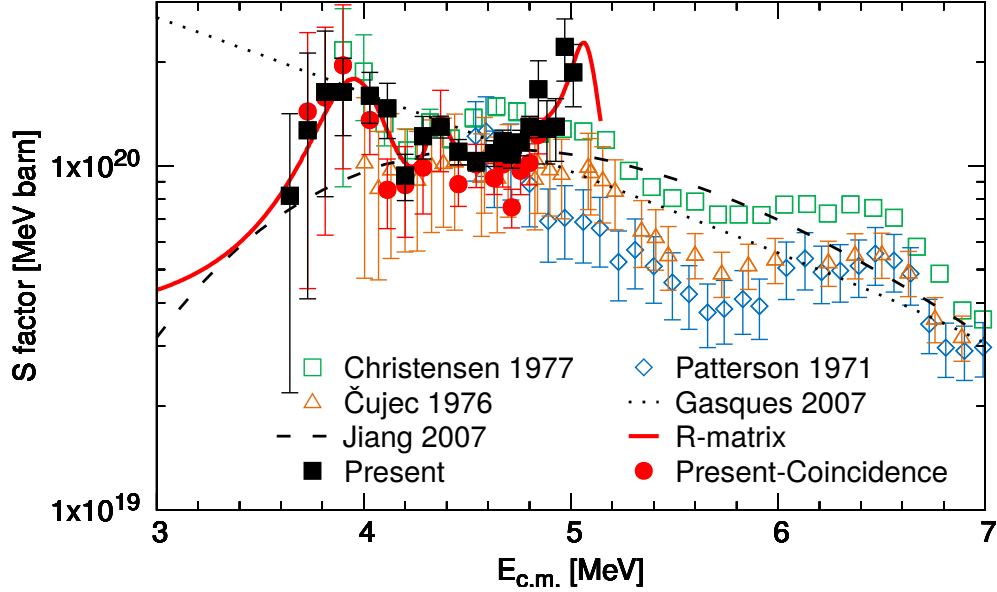
FIG. 13: The S(E) factor of ^{12}\text{C}+^{16}\text{O} fusion. In addition to the data of the present work (solid symbols) also previous data (open symbols) from the literature [15–17] are shown. Patterson’s data [17] does not include the n channel. The dotted line denotes the calculations using the Sao Paulo potential [2, 41]. The hindrance model fit [7] with all the data points is presented as the dashed line. An R-matrix calculation (solid line) based on the analysis of the proton channel is shown as well.
