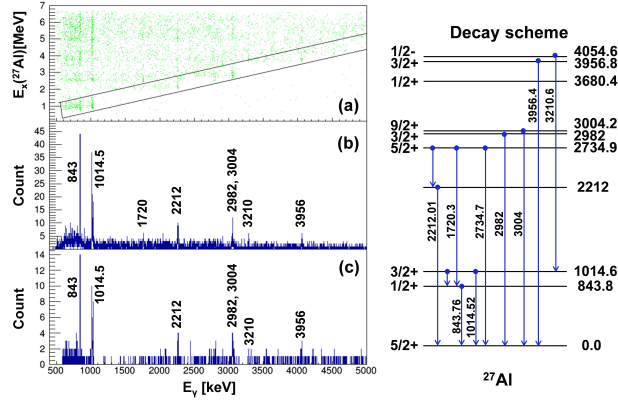
FIG. 6: p- \gamma coincidences demonstrated for E_{beam}=11.3 MeV. The top panel (a) displays coincidence events for protons and \gamma rays, E_x(^{27}\text{Al}) versus E_\gamma . Panel (b) shows the projection of E_\gamma for all coincident events. Panel (c) shows the projection of E_\gamma for the coincident events inside the black-box cut indicated in (a). This corresponds to the \gamma transitions that decay directly from the excited states (with excitation energy up to about 5 MeV) in ^{27}\text{Al} to the ground state.
