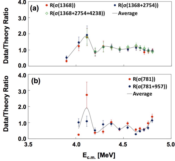
FIG. 9: The ratios of the measured partial cross sections of the ^{24}\text{Mg}+\alpha (upper panel) and ^{27}\text{Si}+n (lower panel) channels to those calculated with the statistical model (SAPPHIRE).
