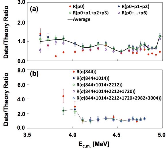
FIG. 8: The ratios of the measured partial cross sections of the ^{27}\text{Al}+p channel to those calculated with the statistical model (SAPPHIRE).
