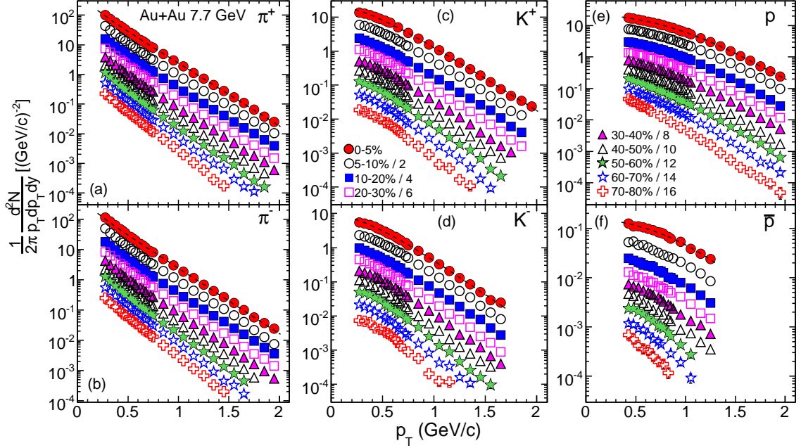
FIG. 12: (Color online) Mid-rapidity ( |y| < 0.1 ) transverse momentum spectra for (a) \pi^+ , (b) \pi^- , (c) K^+ , (d) K^- , (e) p , and (f) \bar{p} in Au+Au collisions at \sqrt{s_{NN}} = 7.7 GeV for different centralities. The spectra for centralities other than 0–5% are scaled for clarity as shown in figure. The curves represent the Bose-Einstein, m_T -exponential, and double-exponential function fits to 0–5% central data for pions, kaons, and (anti-) protons, respectively. The uncertainties are statistical and systematic added in quadrature.
