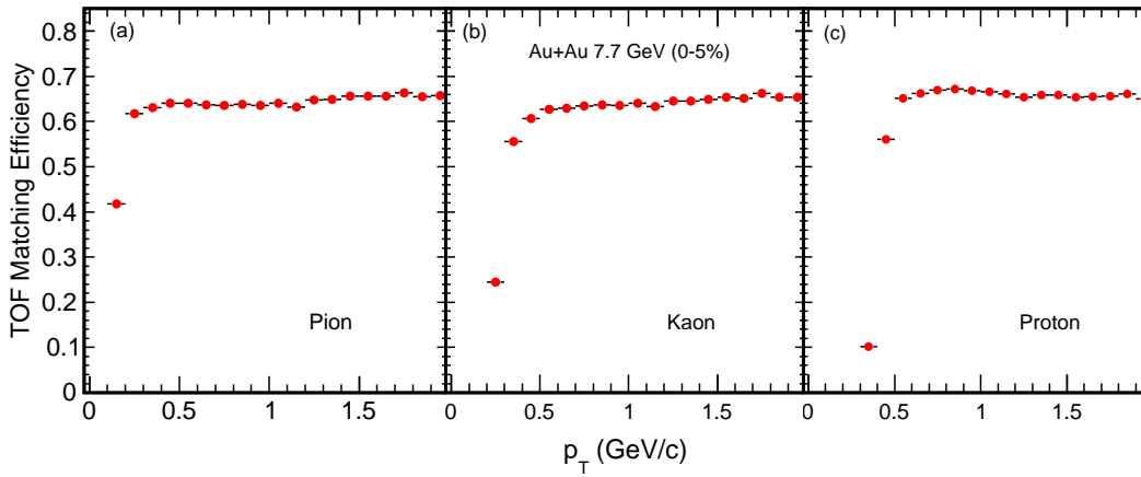
FIG. 8: (Color online) TOF matching efficiency for (a) pions, (b) kaons, and (c) protons as a function of p_T at midrapidity ( |y| < 0.1 ) for 0-5% Au+Au collisions at \sqrt{s_{NN}} = 7.7 GeV.
