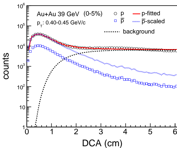
FIG. 11: (Color online) The DCA distributions of protons and antiprotons for 0.40 < p_T < 0.45 GeV/c at midrapidity ( |y| < 0.1 ) in 0–5% Au+Au collisions at \sqrt{s_{NN}} = 39 GeV. The dashed curve is the fitted proton background; the dotted histogram is the \bar{p} distribution scaled by the p/\bar{p} ratio; and the solid histogram is the fit given by Eq. (6).
