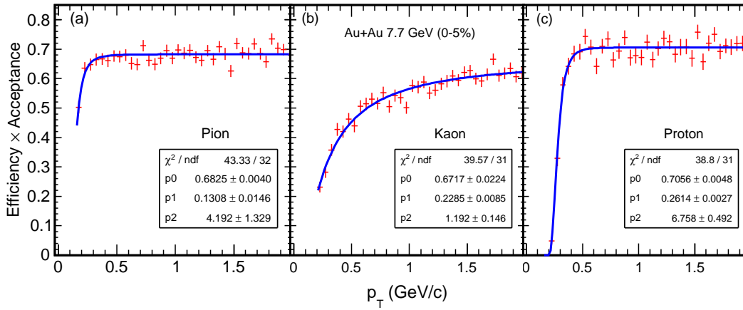
FIG. 7: (Color online) Efficiency \times acceptance obtained from Monte Carlo embedding for reconstructed (a) pions, (b) kaons, and (c) protons in the TPC as a function of p_T at midrapidity ( |y| < 0.1 ) for 0-5% Au+Au collisions at \sqrt{s_{NN}} = 7.7 GeV. The curves represent the functional fit of the form p_0 \exp[-(p_1/p_T)^{p_2}] .
