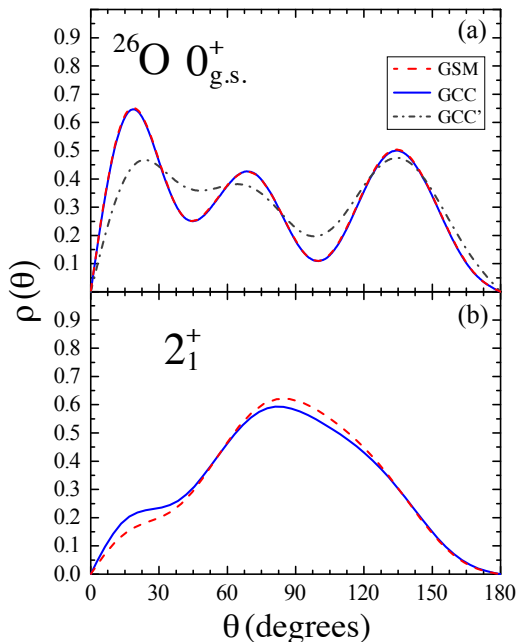
FIG. 8. Two-neutron angular correlation for the 0^+ g.s. (a) and 2_1^+ state (b) configuration of ^{26}\text{O} computed with GCC (solid line) and GSM (dashed line) with \ell_{\text{max}} = 10 . The dash-dotted curve labeled GCC' in panel (a) shows GCC results obtained with the strength of the neutron-neutron interaction reduced by 50%.
