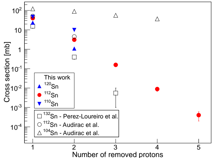
FIG. 5. (Color online) Cross sections of the proton removal channels produced in the fragmentation of different tin isotopes measured by Perez-Loureiro et al. (open squares) [37], Audirac et al. (open circles and triangles) [22], and this work (solid symbols). The data uncertainties are shown if they exceed the size of the symbols.
