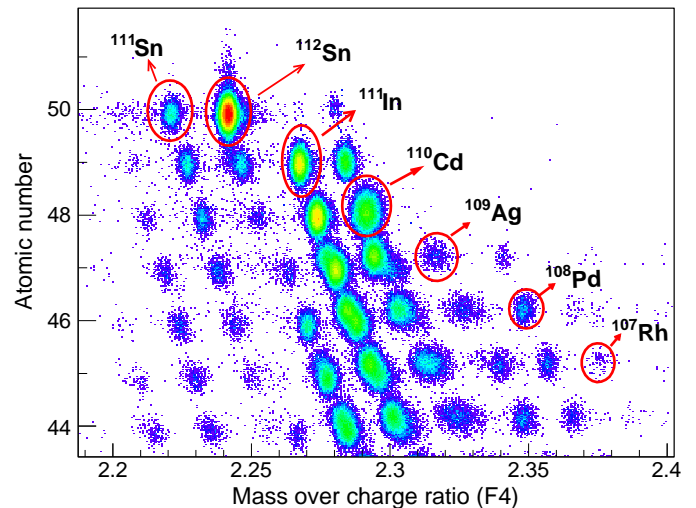
FIG. 2. (Color online) Identification matrix at the final focal plane (F4) of the FRS obtained in reactions induced by ^{112}\text{Sn} impinging on the carbon target. The figure was obtained by overlapping several magnetic settings of the FRS.
