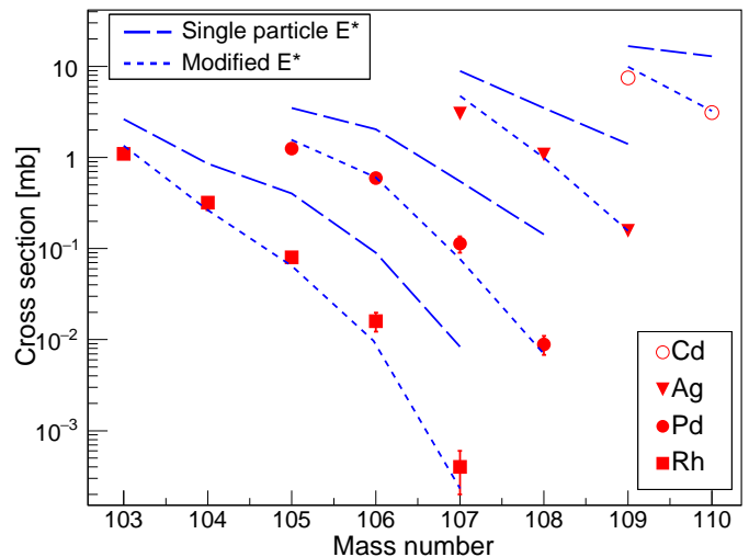
FIG. 6. (Color online) Measured isotopic production cross sections of fragment residues produced in the reaction ^{112}\text{Sn}(1A \text{ GeV}) + ^{12}\text{C} (points) compared with different calculations (lines). The data uncertainties are shown if they exceed the size of the symbols.
