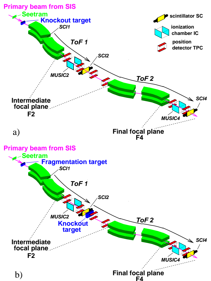
FIG. 1. (Color online) Schematic view of the FRS experimental setups used in the present work. (a) Setup with the reaction target at the entrance of the spectrometer to investigate knockout reactions of stable tin isotopes ( ^{112}\text{Sn} and ^{124}\text{Sn} ). (b) Setup with a fragmentation target at the entrance of the FRS to produce secondary beams of ^{110}\text{Sn} and ^{120}\text{Sn} that then impinged on a second carbon target located at the intermediate focal plane F2 in order to induce knockout reactions.
