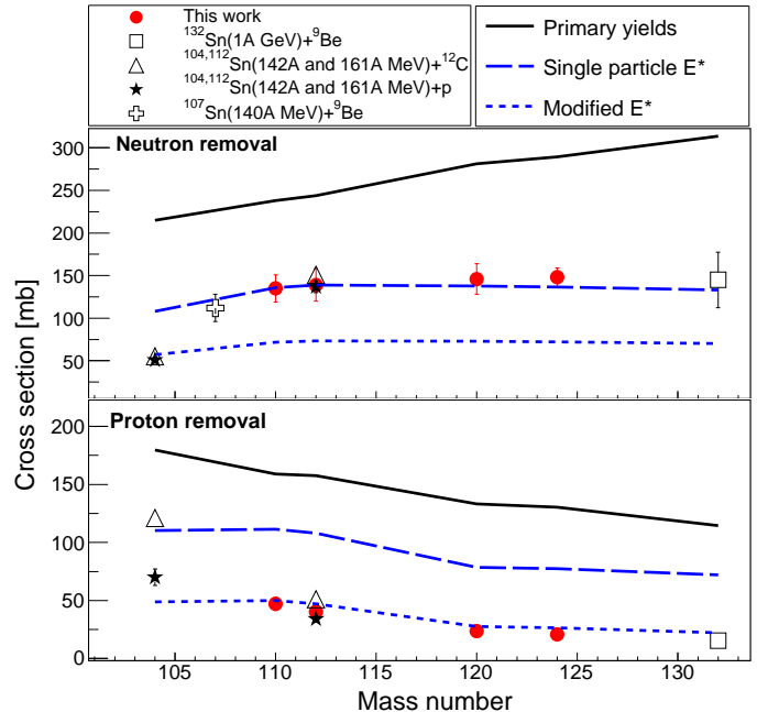
FIG. 3. (Color online) Neutron (upper panel)- and proton (lower panel)-removal cross sections measured for different tin isotopes covering a large range in neutron excess: Perez-Loureiro et al. (open squares) [37], Audirac et al. (open triangles and solid stars) [22], Cerizza et al. (open cross) [44], and this work (solid dots). The data uncertainties are shown if they exceed the size of the symbols. This set of data is compared with Glauber model calculations (lines).
