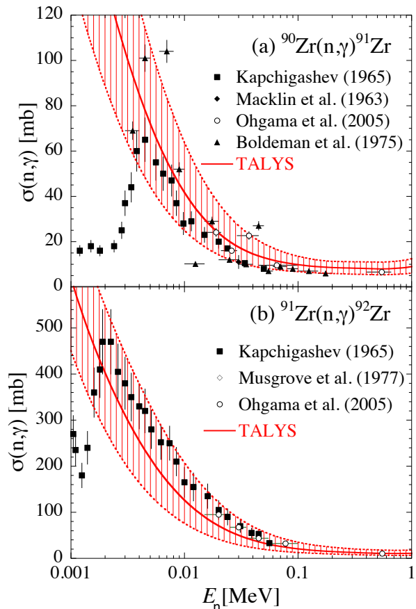
FIG. 9: (Color online) (a) Comparison between the experimental ^{90}\text{Zr}(n, \gamma)^{91}\text{Zr} cross section [51–53] and the one obtained with the TALYS code on the basis of the NLD and \gamma\text{SF} derived experimentally in the present work. The hashed area depicts all the experimental and model-dependent uncertainties taken into account in the present analysis. (b) Same for ^{91}\text{Zr}(n, \gamma)^{92}\text{Zr} cross section with experimental data taken from Refs. [51, 53, 54].
