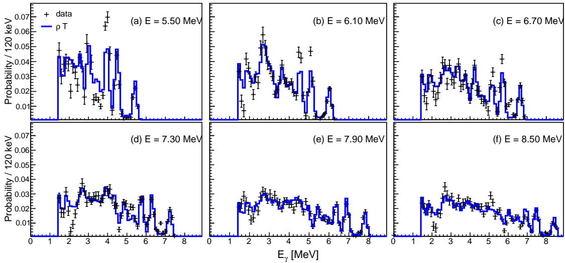
FIG. 5: (Color online) Same as Fig. 4 for ^{92}\text{Zr} . Both the \gamma and excitation energy dispersions are 120 keV/ch.
