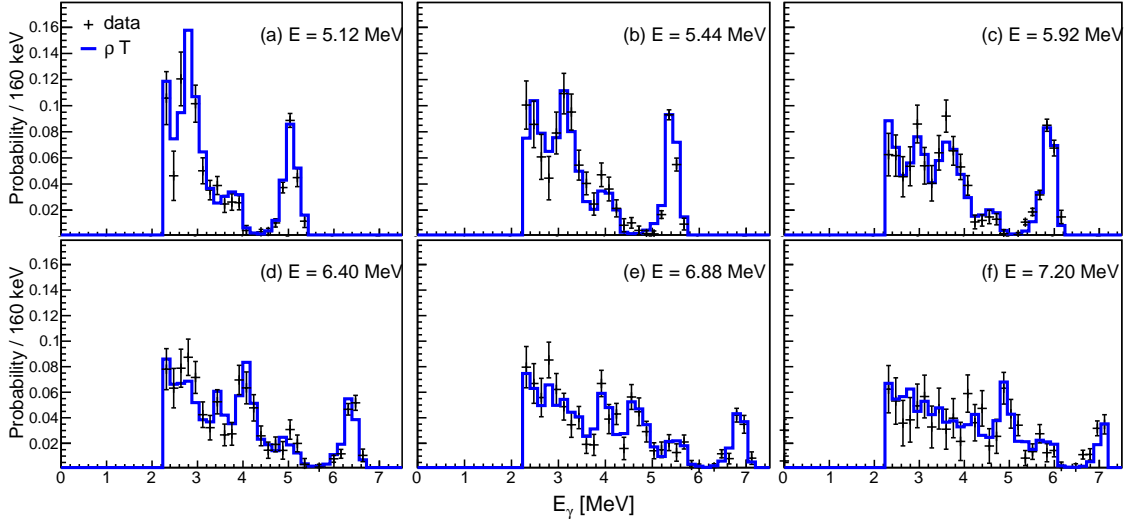
FIG. 4: (Color online) Primary \gamma -ray spectra from various initial excitation energies E (crosses) in ^{91}\text{Zr} . The spectra are compared to the product \rho(E - E_\gamma)\mathcal{T}(E_\gamma) (blue histogram). Both the \gamma and excitation energy dispersions are 160 keV/ch.
