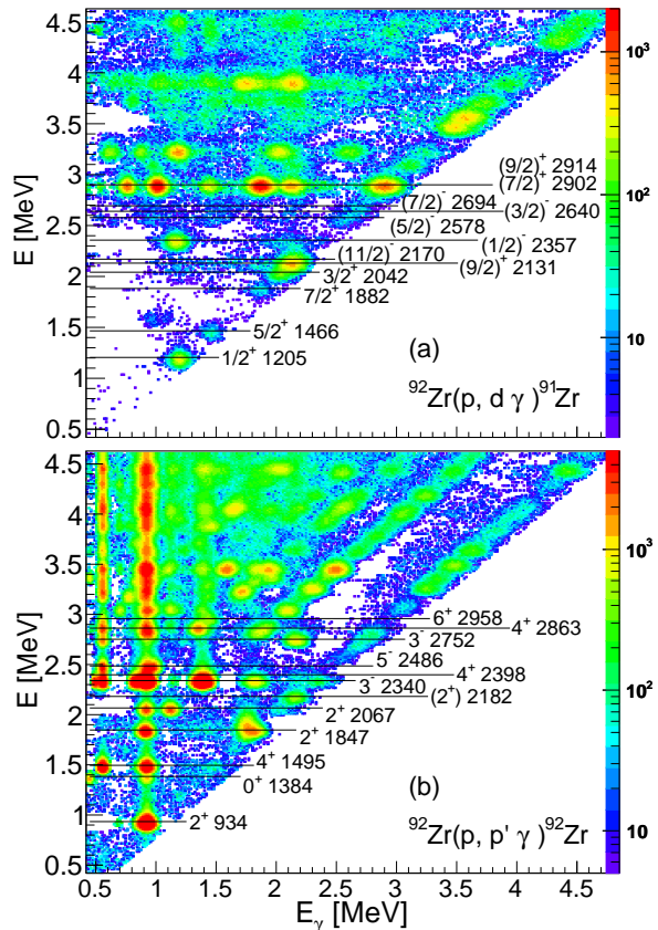
FIG. 1: (Color online) The discrete part of the particle- \gamma coincidence matrices for the (a) ^{92}\text{Zr}(p, d)^{91}\text{Zr} and (b) ^{92}\text{Zr}(p, p')^{92}\text{Zr} reactions. Only excitation energies between 0.5 and 4.5 MeV are shown in order to highlight the decay pattern recognized in the present experiment. The pixel width is 16 keV \times 16 keV.
