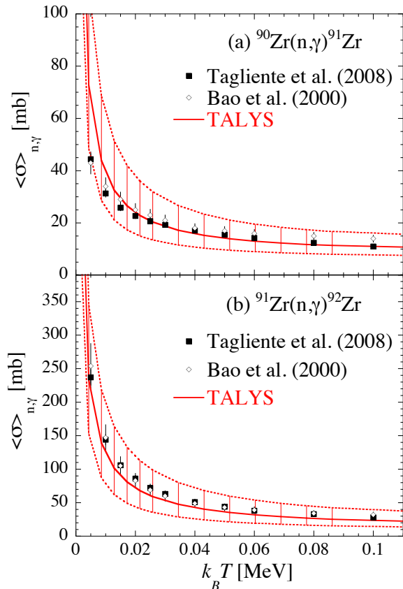
FIG. 10: (Color online) Comparison between the experimental ^{90}\text{Zr}(n, \gamma)^{91}\text{Zr} Maxwellian-averaged cross section [26, 55] and the one obtained with the TALYS code on the basis of the NLD and \gamma SF derived experimentally in the present work. (b) Same for ^{91}\text{Zr}(n, \gamma)^{92}\text{Zr} Maxwellian-averaged cross section with experimental data taken from Refs. [27, 55].
