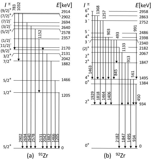
FIG. 3: Partial level schemes for (a) ^{91}\text{Zr} and (b) ^{92}\text{Zr} . Only the levels, which are most strongly populated in the (p,p') and (p,d) reactions, respectively, are shown. The most prominent \gamma -rays from these states are displayed with \gamma energies in keV. More complete level schemes are found in Ref. [17].
