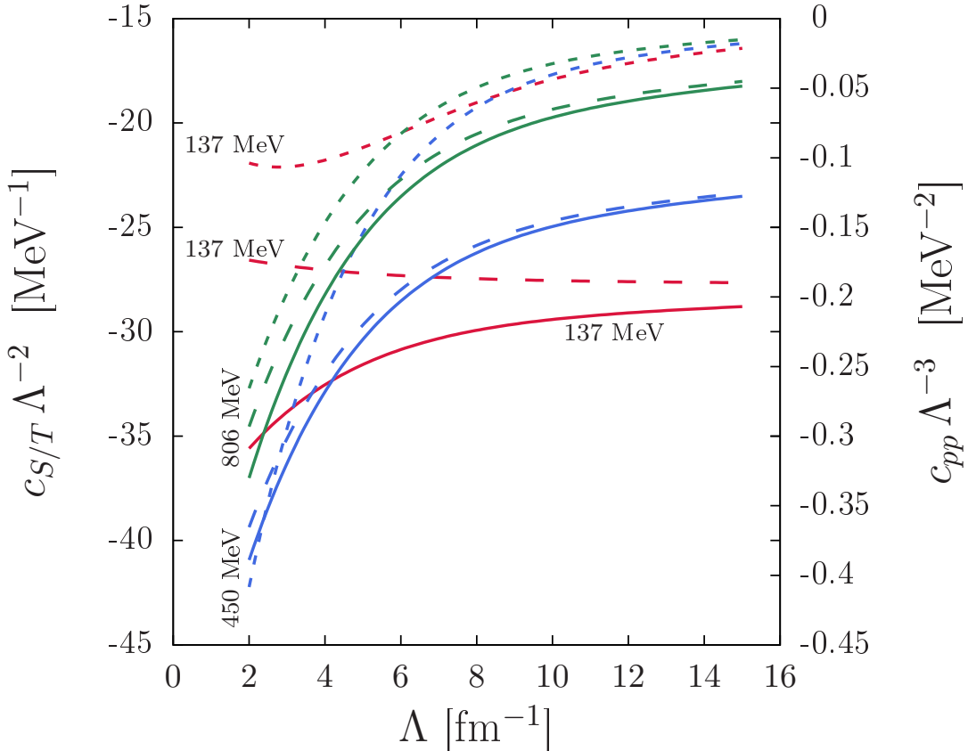
FIG. 1. (Color online) Cutoff dependence of the LECs c_S (solid line, left y-axis), c_T (dashed line, left y-axis), and c_{pp} (short dashed, right y-axis) for three pion masses, m_\pi = 137 \text{ MeV} (red), m_\pi = 450 \text{ MeV} (blue), and m_\pi = 806 \text{ MeV} (green).
