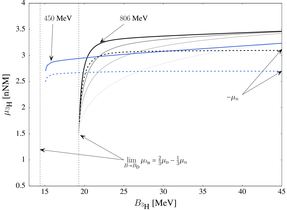
FIG. 4. (Color online) The magnetic moment of the triton as a function of its binding energy for m_\pi = 806 MeV (gray( \Lambda = 4 fm ^{-1} ) \rightarrow black ( \Lambda = 15 fm ^{-1} )) and m_\pi = 450 MeV (blue, \Lambda = 8 fm ^{-1} ). Vertical dashed lines mark the deuteron-neutron thresholds at B_D = 19.5 MeV and B_D = 14.4 MeV, respectively. LO results with one-body-current coupling (dotted lines) are compared with NLO values (solid lines) which consider also the two-body-current coupling l_1, l_2 . Asymptotic limits are indicated with arrows, for B_{3H} \rightarrow B_D : \mu_{3H} \rightarrow 1.196 nNM (450 MeV), \mu_{3H} \rightarrow 1.472 nNM (806 MeV); and B_{3H} \rightarrow \infty : \mu_{3H} \rightarrow 2.70 nNM (450 MeV), \mu_{3H} \rightarrow 3.119 nNM (806 MeV).
