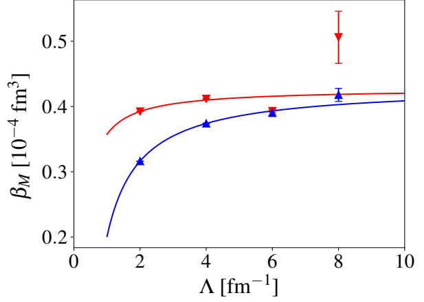
FIG. 7. (Color online) Regulator dependence of the magnetic polarizability EFT calculations for {}^3\text{He} and triton m_\pi = 806 MeV.
