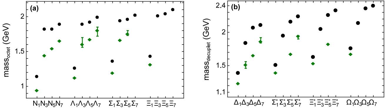
FIG. 2. Left panel (a) : Pictorial representation of octet masses in Table III. Circles (black) – computed masses; and diamonds (green) – empirical masses. On the horizontal axis we list a particle name with a subscript that indicates its row in the table, e.g. N_1 means nucleon column, row 1. In this way the labels step through ground-state, radial excitation, parity partner, parity partner’s radial excitation. Right panel (b) : Analogous plot for the decuplet masses in Table III. Where noticeable, the estimated uncertainty in the location of a resonance’s pole position is indicated by an error bar.
