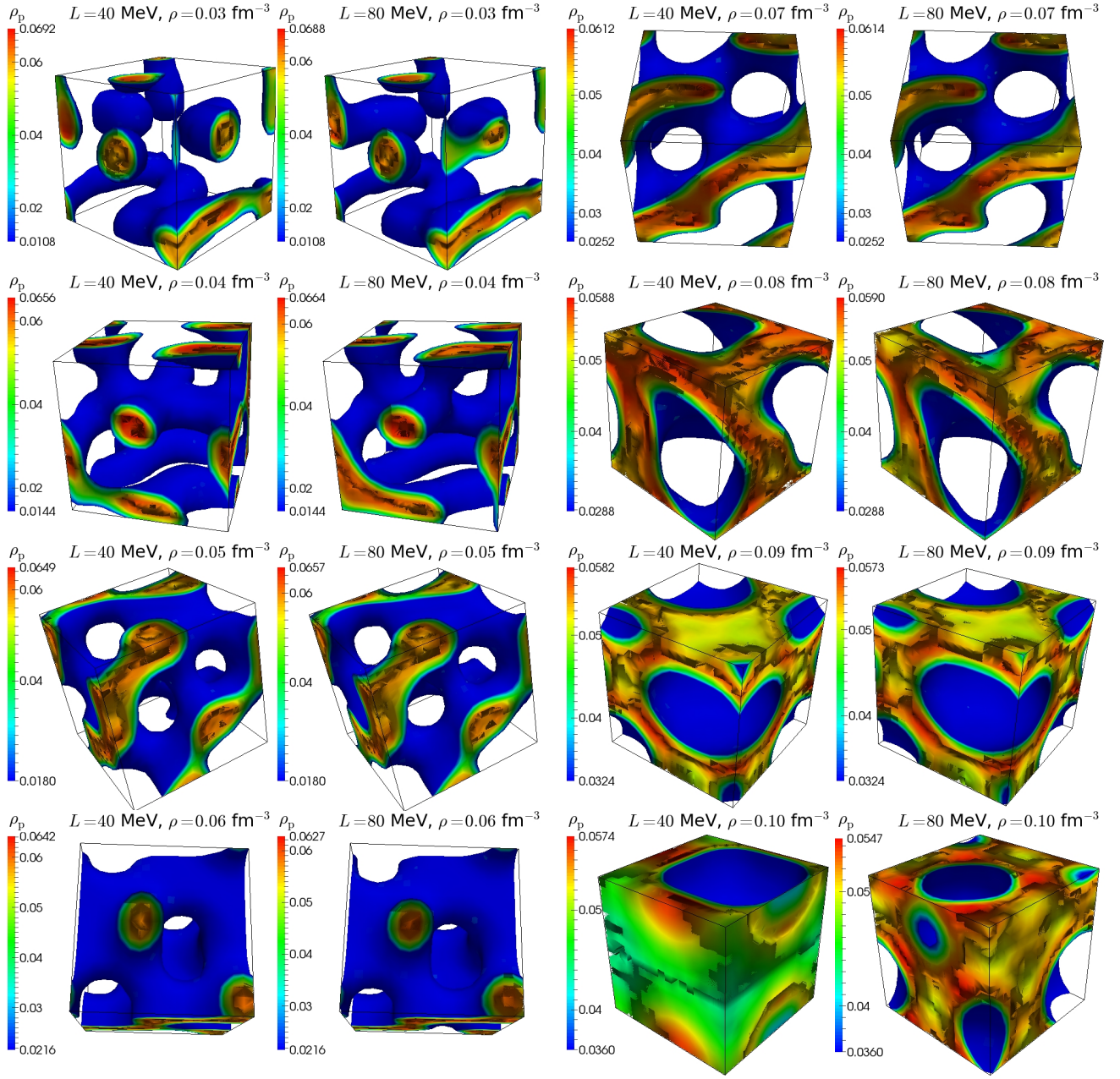
FIG. 12. (Color online) Isosurface of proton densities are plotted using the same prescription as in Fig. 5 except now the proton fraction of the system is Y_p = 0.40 .
