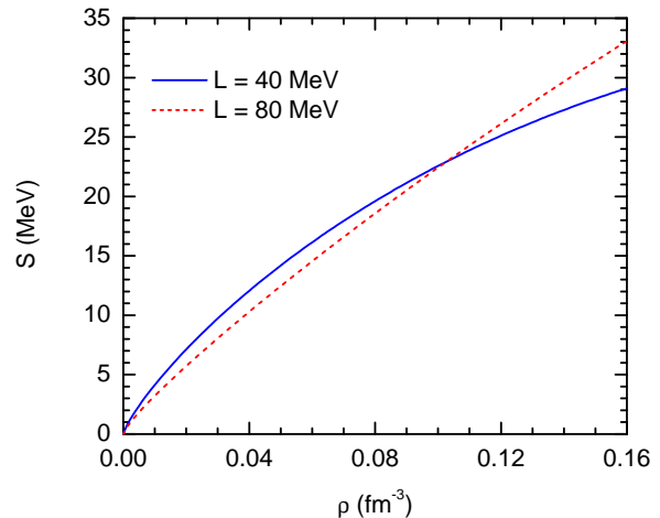
FIG. 1. (Color online) Density dependence of the nuclear symmetry energy for the two models discussed in the text.
