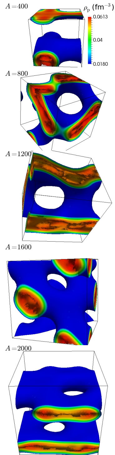
FIG. 3. (Color online) The appearance of the nuclear waffle phase at Y_p = 0.40 , \rho = 0.05 \text{ fm}^{-3} for different volume sizes containing A = 400, 800, 1200, 1600 and 2000 nucleons from top to the bottom, respectively. The sides of the cubic volumes correspondingly are equal to 20 fm, 25.2 fm, 28.8 fm, 31.7 fm, 34.2 fm. The blue color represents isosurface proton densities of \rho_p = 0.9(Y_p\rho) and the red color represents the region with the highest proton density \rho_p^{\text{max}} within the pasta structure, where \rho is the average nucleon density. This figure and all other similar figures throughout the paper are generated using the ParaView software [71].
