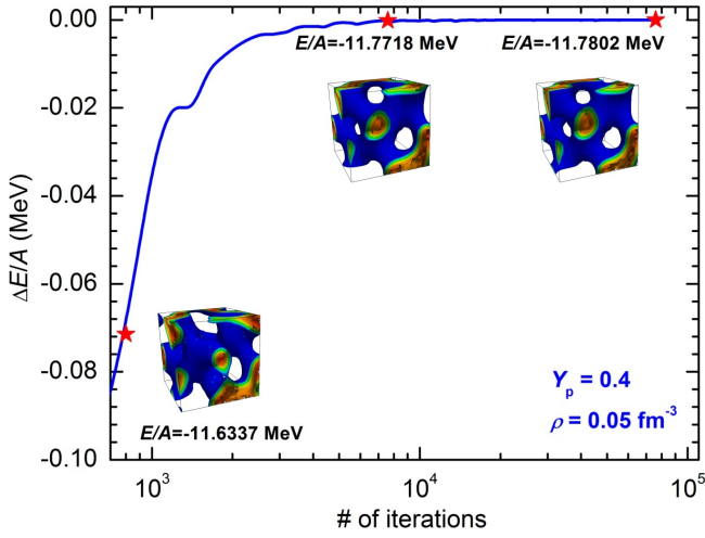
FIG. 14. (Color online) Energy difference per 200 iterations versus the number of iterations is plotted for a total of 76,000 iterations. The inset pasta phases correspond the simulation phases at 800, 7600, and 76000 iterations, respectively.
