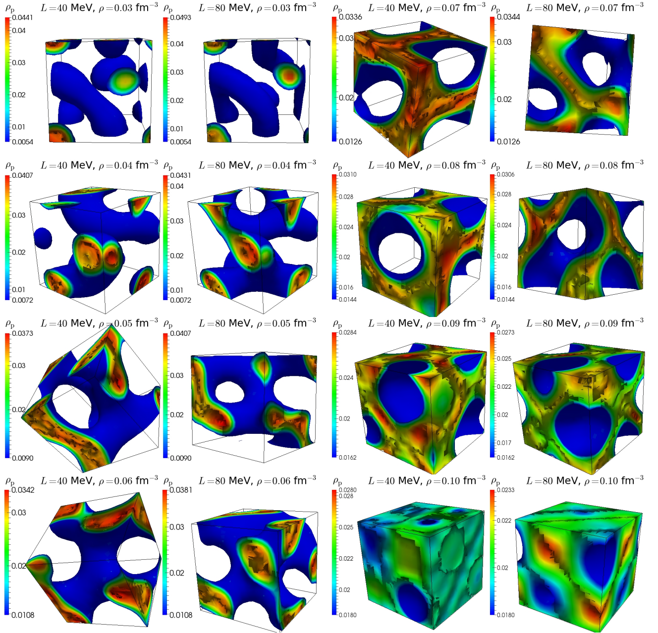
FIG. 10. (Color online) Isosurface of proton densities are plotted using the same prescription as in Fig. 5 except now the proton fraction of the system is Y_p = 0.20 .
