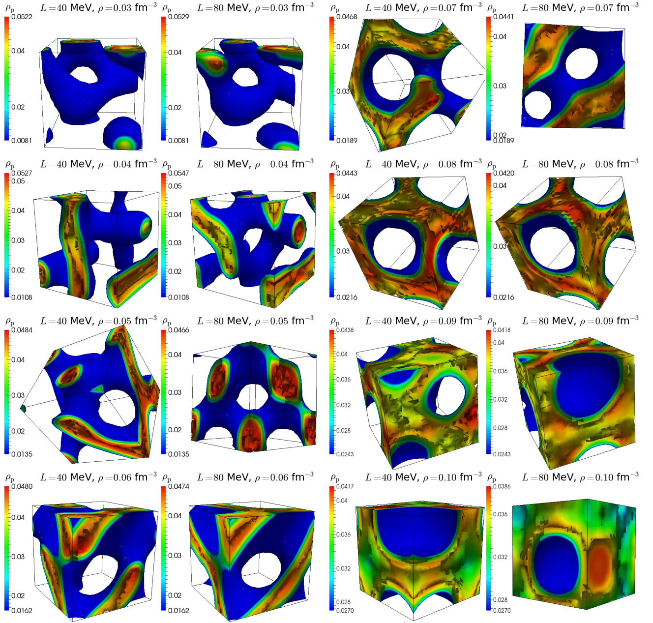
FIG. 11. (Color online) Isosurface of proton densities are plotted using the same prescription as in Fig. 5 except now the proton fraction of the system is Y_p = 0.30 .
