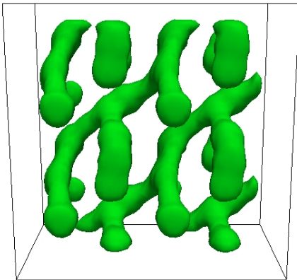
FIG. 9. (Color online) Four periodic copies of pasta structure with Y_p = 0.10 , \rho = 0.05 \text{ fm}^{-3} for model with L = 80 \text{ MeV} are put together for a simulation box posed at a different angle for better visualization. The box dimensions are 68.4 \times 68.4 \times 34.2 \text{ fm} , and the isosurface of proton density at \rho_p = 0.02 \text{ fm}^{-3} is plotted.
