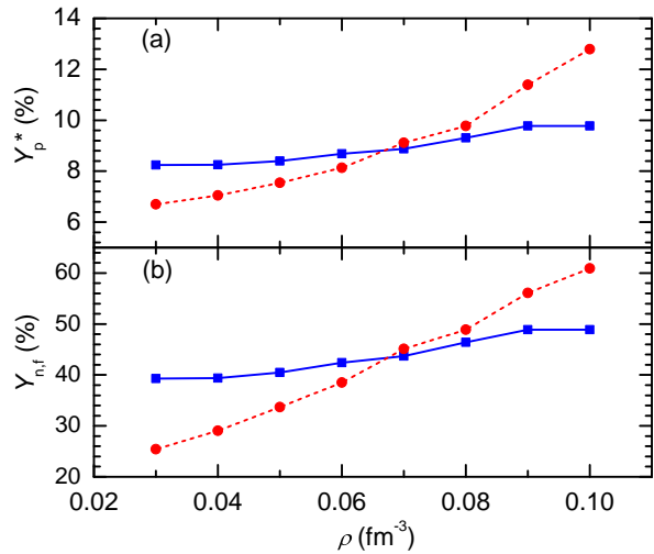
FIG. 6. (Color online) Effective proton fractions Y_p^* (top panel) and free neutron fractions Y_{n,f} (bottom panel) are plotted as a function of total average baryon density for the two models discussed in the text.
