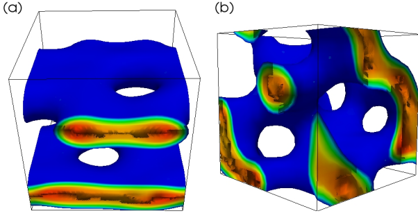
FIG. 13. (Color online) Nuclear pasta phases at \rho = 0.05 \text{ fm}^{-3} and Y_p = 0.40 that started out from two different initial configurations with nucleons randomly distributed in the box and the grid spacing of (a) \Delta x = 1.00 \text{ fm} and (b) \Delta x = 1.42 \text{ fm} .
