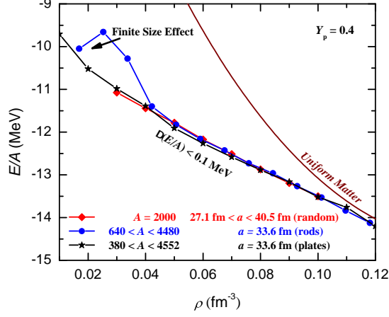
FIG. 17. (Color online) Total energy per nucleon as a function of density for pasta structures that are obtained from three different initial configurations.
