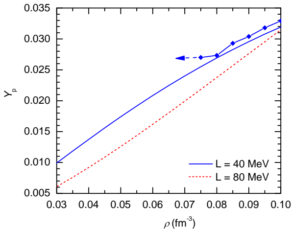
FIG. 4. (Color online) Proton fractions as a function of baryon density for a uniform neutron-star matter in two models discussed in the text. Also shown is the proton fractions at few fixed average baryon densities obtained directly from nuclear pasta simulations (diamonds).
