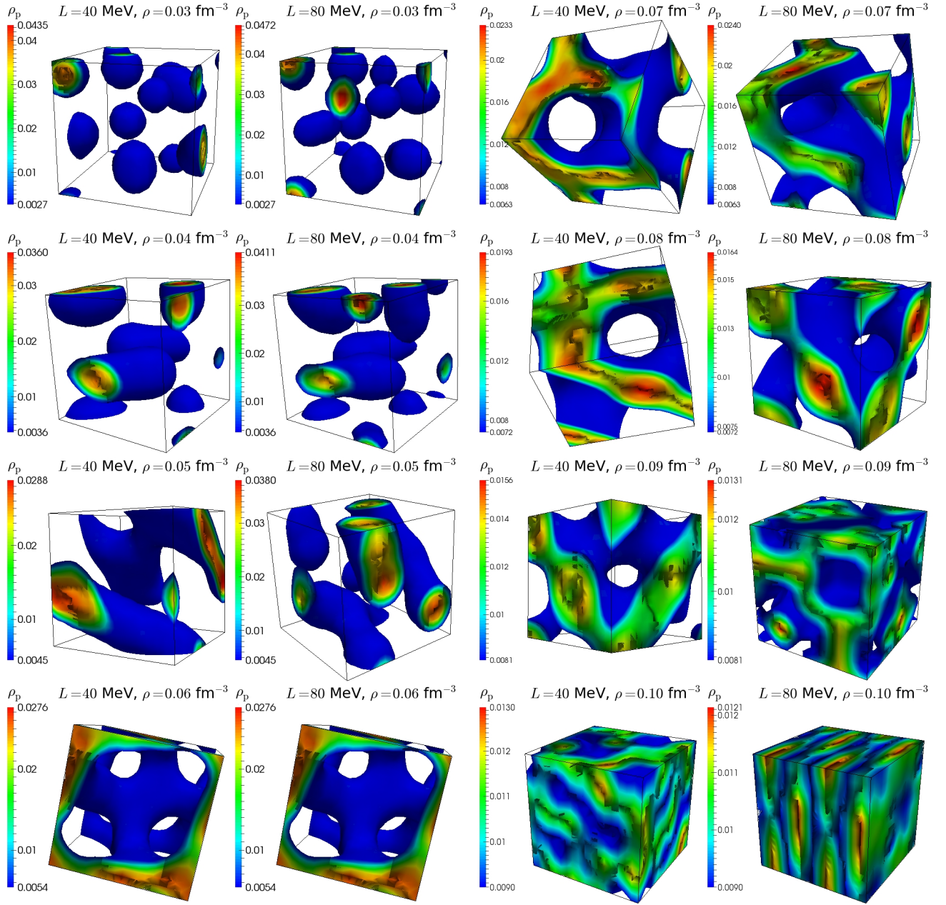
FIG. 8. (Color online) Isosurface of proton densities are plotted using the same prescription as in Fig. 5 except now the proton fraction of the system is Y_p = 0.10 .
