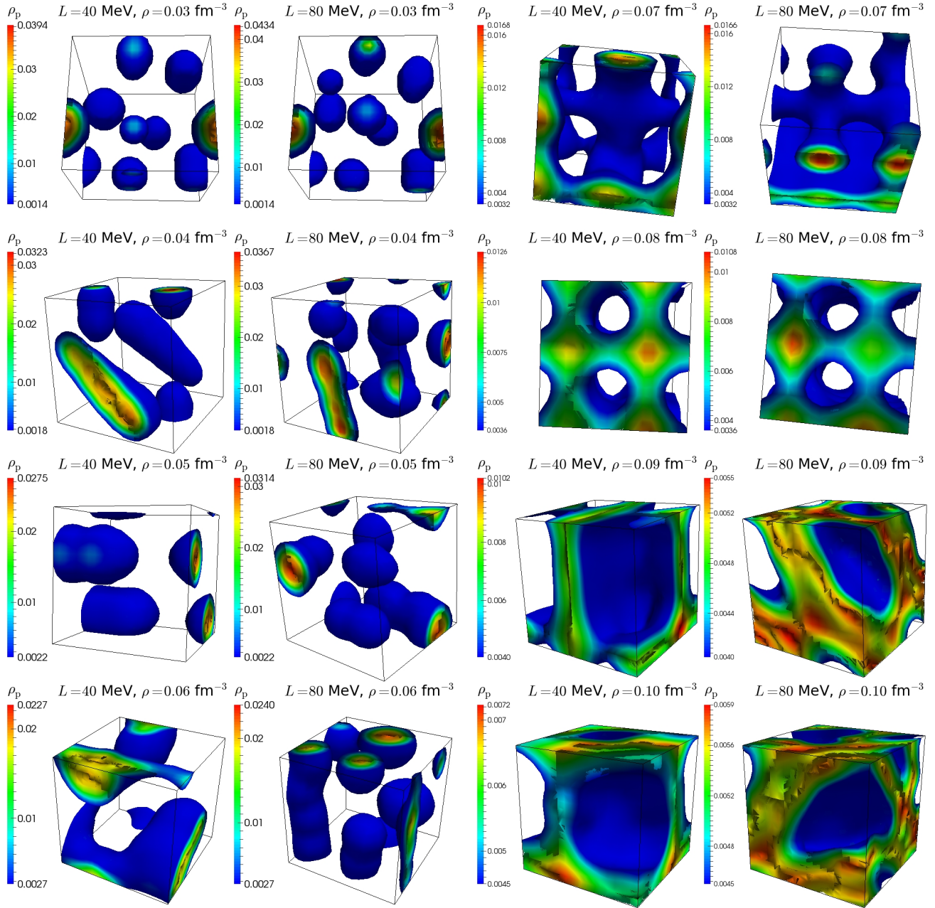
FIG. 5. (Color online) Isosurface of proton densities are plotted for the two model discussed in the text over the range of baryon densities at a fixed proton fraction of Y_p = 0.05 . The total number of nucleons are fixed at A = 2000 and the side of the cubic box varies from 40.55 fm down to 27.14 fm, corresponding to average baryon densities of 0.03 \leq \rho \leq 0.10 \text{ fm}^{-3} , respectively.
