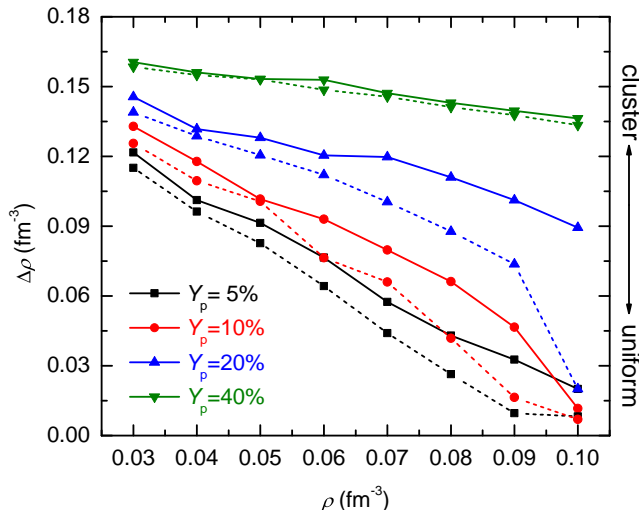
FIG. 7. (Color online) Density contrast \Delta\rho within the pasta simulation box as a function of the average baryon density \rho for various proton fractions Y_p for models with L = 40 MeV (solid) and L = 80 MeV (dashed). System is considered as uniform when \Delta\rho = 0 , otherwise it is pasta-rich.
