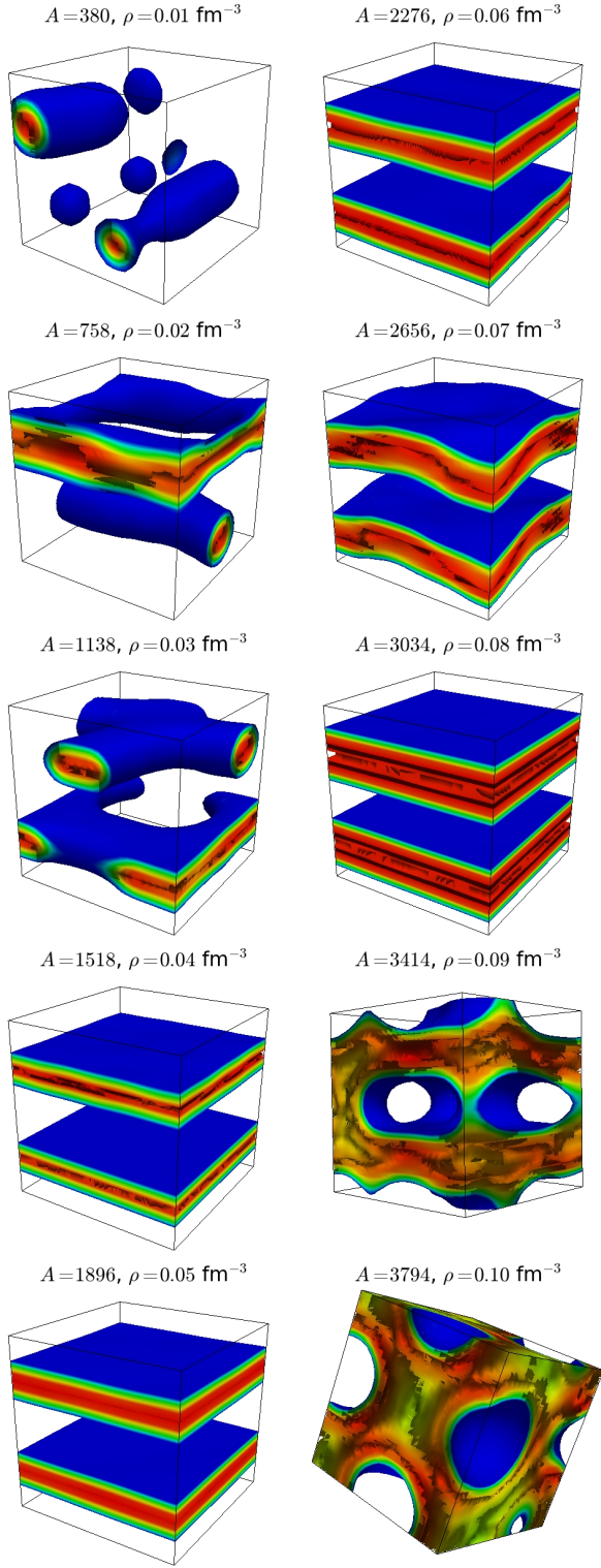
FIG. 16. (Color online) Nuclear pasta simulations with proton fractions of Y_p = 0.40 at average baryon densities of 0.01 < \rho < 0.10 \text{ fm}^{-3} corresponding to a cubic volume with a \approx 33.6 \text{ fm} . All systems are initialized with nucleons distributed randomly to form two identical parallel plates.
