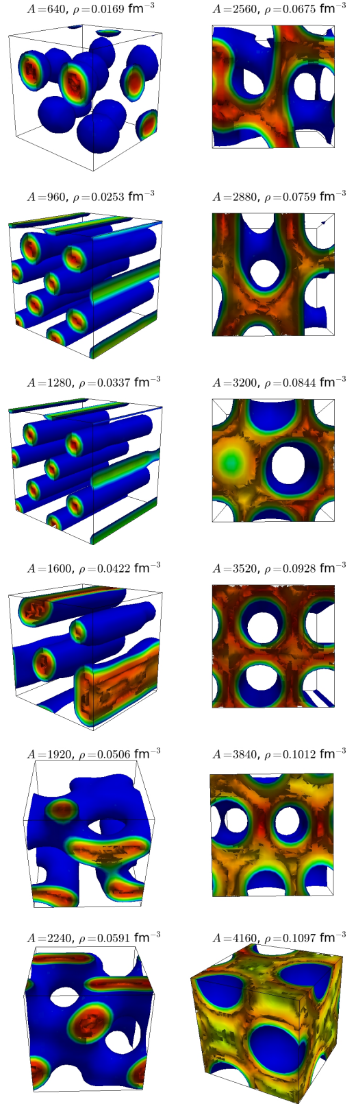
FIG. 15. (Color online) Nuclear pasta simulations with proton fractions of Y_p = 0.40 for a cubic volume of fixed side a = 33.6 \text{ fm} containing 640 < A < 4180 nucleons. All systems are initialized with nucleons distributed randomly to form eight identical rods aligned on a face-centered site.
