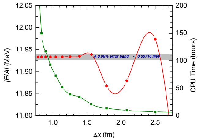
FIG. 2. (Color online) The absolute value of the binding energy per nucleon and the simulation runtime as a function of the grid spacing \Delta x for a system of A = 800 nucleons at the average baryon density of \rho = 0.0512 \text{ fm}^{-3} and proton fraction of Y_p = 0.4 .
