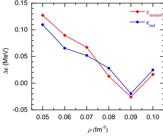
FIG. 18. (Color online) The energy differences of final configurations (shown in Fig. 17). Here \Delta \epsilon_{\text{random}} \equiv (E/A)_{\text{random}} - (E/A)_{\text{plate}} and \Delta \epsilon_{\text{rod}} \equiv (E/A)_{\text{rod}} - (E/A)_{\text{plate}} .
