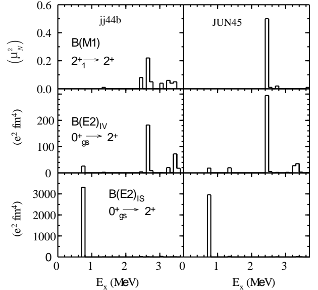
FIG. 8. B(M1) , B(E2)_{IV} and B(E2)_{IS} strength from shell-model calculations. See the text for more details.
