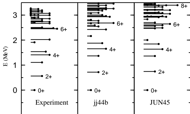
FIG. 5. Comparison of experimental and theoretical (shell model) level energies for the positive-parity states of ^{76}\text{Ge} . Levels with the same spin are indicated with lines of the same length.
