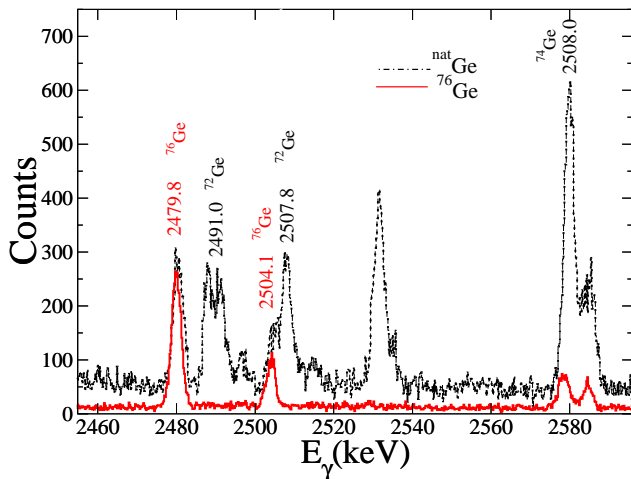
FIG. 1. (Color online) Portion of the \gamma -ray spectrum from 3.5-MeV neutrons incident on the enriched ^{76}\text{GeO}_2 scattering sample (solid) and a comparison with ^{nat}\text{Ge} (dashed) as the sample. The ^{nat}\text{Ge} has been normalized to the ^{76}\text{Ge} spectrum with respect to time and amount of ^{76}\text{Ge} present. The peaks belonging to the ^{76}\text{Ge} have similar count in both spectra.
