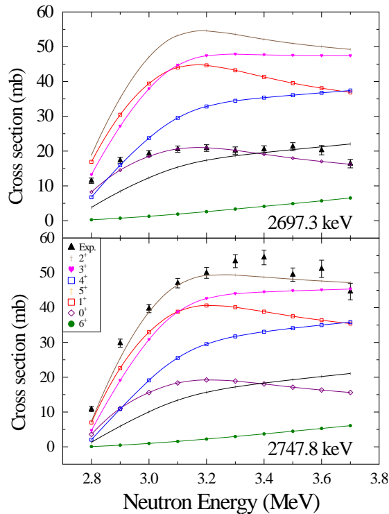
FIG. 2. (Color online) Comparison of the excitation functions for the 2697.3 keV 0^+ and 2747.8 keV 2^+ levels with the theoretical cross sections calculated with the code CINDY [20].
