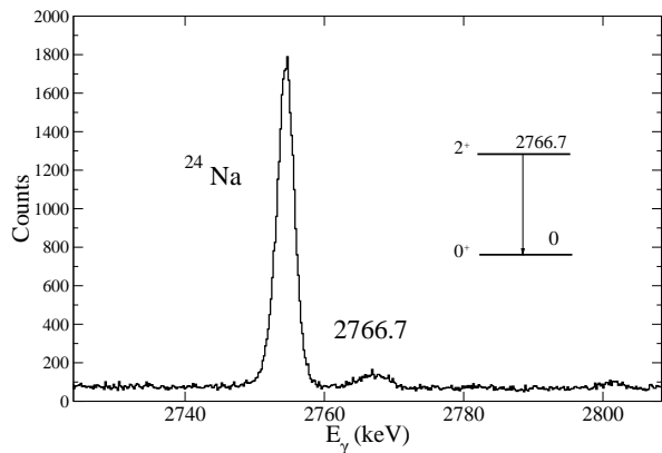
FIG. 9. Portion of the summed \gamma -ray spectrum. See the text for more details.
