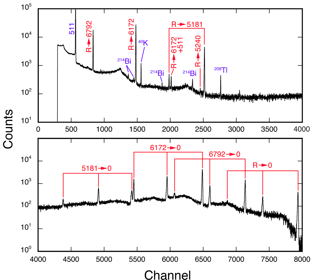
FIG. 6. (Color online) Spectrum of the ^{14}\text{N}(p, \gamma)^{15}\text{O} reaction taken at E_p^{\text{lab}} = 284 keV with the HPGe detector. Gamma rays associated with the decay of the 259-keV resonance are labeled in red, background lines are denoted in purple.
