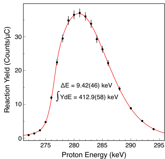
FIG. 11. (Color online) An example of a yield curve for the 259-keV resonance. The Markov Chain Monte Carlo fit is denoted by the red line.
