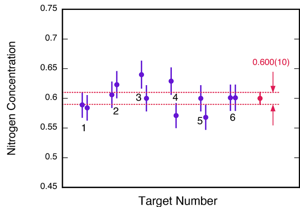
FIG. 2. (Color online) Relative concentration of ^{14}\text{N} in the region of saturation density. Each pair of closely-spaced points corresponds to a different target, with two measurements at different locations on the same target. Note that only statistical uncertainties are shown. The average is denoted by the red point and the uncertainty calculated via bootstrapping is indicated by the dashed lines.
