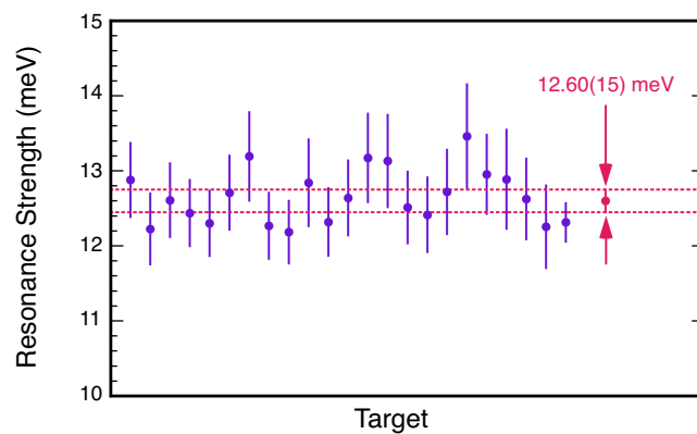
FIG. 12. (Color online) Resonance strengths extracted from independent yield-curve measurements on 23 separate targets (blue points). The red point and dashed lines represent the weighted average of the individual points. Note that only statistical uncertainties are shown.
