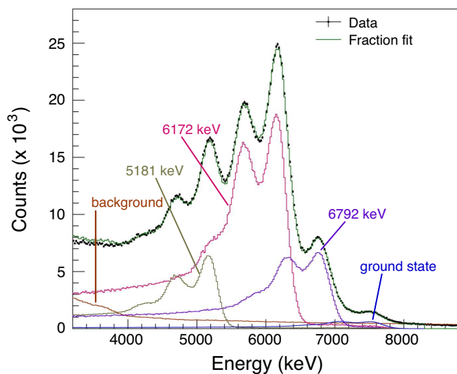
FIG. 10. (Color online) Maximum-likelihood fit of the multiplicity-1 data collected with the APEX detector. The data are denoted by the black points, the fit by the green line and the individual templates are displayed as the colored histograms.
