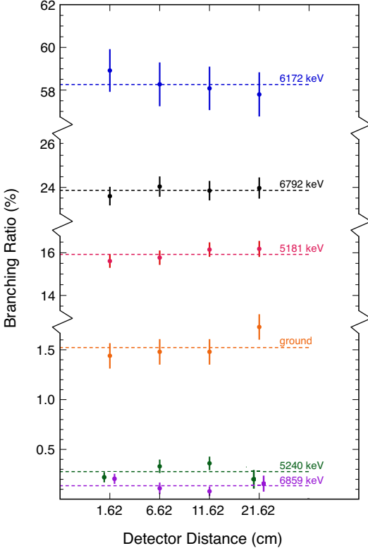
FIG. 8. (color online) Branching ratios measured using the HPGe detector at distances of 1.62, 6.62, 11.62, and 21.62 cm from the target to the detector crystal. The dashed lines are the weighted averages of the individual measurements for each transition, which are listed in Table III.
