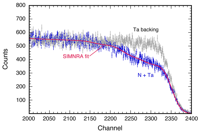
FIG. 1. (Color online) RBS spectra from an implanted target (blue) and a tantalum backing (grey). The SIMNRA [27] fit is shown in red.
