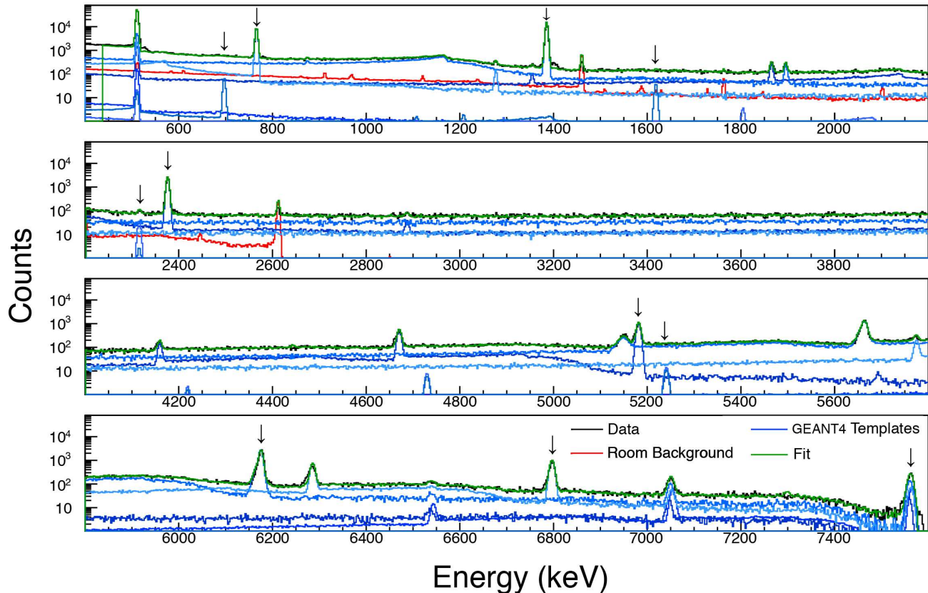
FIG. 7. (color online) The result of the best fit, shown in green, to HPGe data for the 259-keV resonance in the ^{14}\text{N}(p, \gamma)^{15}\text{O} reaction, shown in black, as derived using the TFractionFitter [46] class of ROOT [47] as described in the text and in Refs. [48, 49]. Note that the data are not easily distinguished from the fit. Full-energy peaks for primary and secondary transitions are indicated by arrows and the corresponding templates are also shown in light and dark blue. The room-background spectrum is shown in red.
