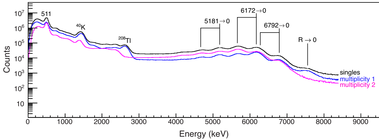
FIG. 9. (Color online) Reconstructed APEX energy spectra of \gamma rays from the decay of the 259-keV resonance with imposed multiplicity-1 and -2 cuts. The ground-state and secondary \gamma rays for transitions to the 5181-, 6172-, and 6792-keV states are indicated as well as their corresponding single-escape peaks.
