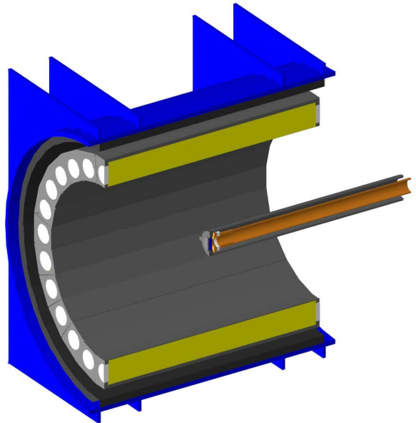
FIG. 3. (Color online) Cutaway view of the GEANT4 geometry used in the Monte Carlo simulation of the APEX detector. The beam enters the target chamber from the right.
