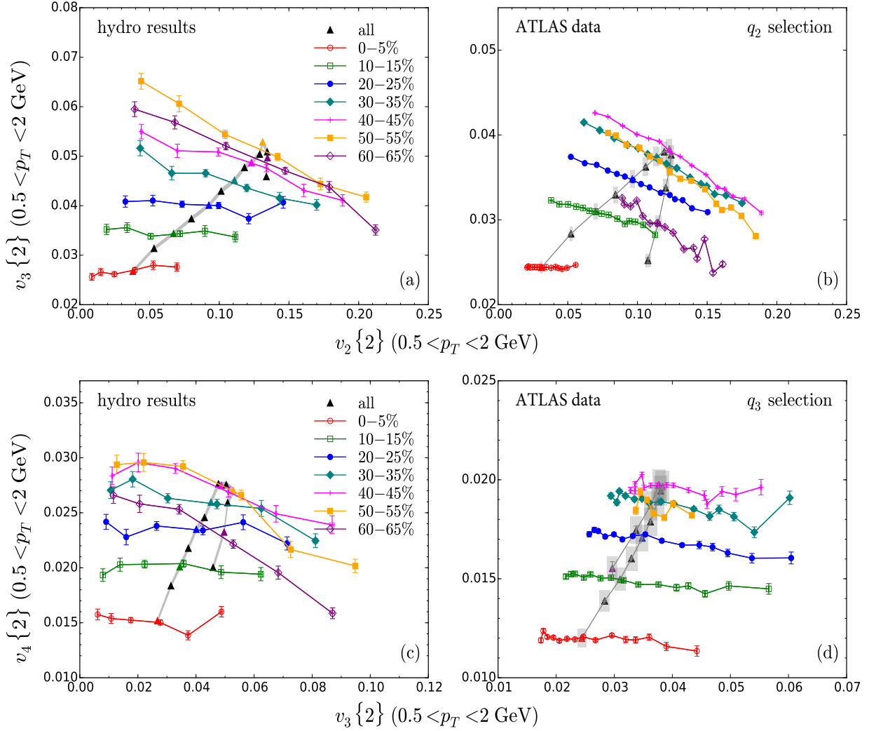
FIG. 1. (Color online) The correlations between v_3 and v_2 (a,b) and between v_4 and v_3 (c,d), as a function of event centrality for the 14 centrality bins described in the text, from viscous hydrodynamic simulations (a,c) and from experimental data [19] (b,d) for Pb-Pb collisions at the LHC. Solid triangles represent v_m - v_n correlations in a given centrality bin; black triangles represent the values for centrality bins for which event-shape selected results are suppressed to avoid excessive clutter, while colored solid triangles represent the bin-averaged values for the centrality bins listed in the legend for which we show, with symbols of the same color, the v_m - v_n correlations for event-shape selected events within the given centrality bin. In panels (a,b) event shapes are selected using q_2 , for panels (c,d) we use q_3 for the event-shape selection. For the ATLAS data [19] (b,d) statistical and systematic uncertainties are shown as error bars and grey shaded boxes, respectively. Note that what is plotted is the rms value of v_n , i.e. v_n\{2\} , for charged hadrons (after resonance decays) integrated over the indicated p_T range; this agrees with Ref. [19] where, however, the qualifier \{2\} was dropped for clarity. The reader should also note the different vertical and horizontal ranges covered by the theoretical (a,c) and experimental (b,d) results.
