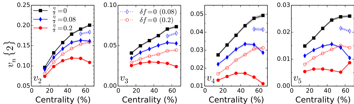
FIG. 5. (Color online) v_2, v_3, v_4, and v_5 as function of collision centrality from ideal and viscous hydrodynamics with KLN initial conditions. Each centrality bin contains 1000 events. Solid black squares correspond to ideal hydrodynamics, while solid blue diamonds and solid red circles correspond to viscous hydrodynamics with \eta/s = 0.08 and 0.2 , respectively. The open blue diamonds and red circles are also from viscous hydrodynamics with \eta/s = 0.08 and 0.2 , respectively, but without including the viscous correction \delta f at freeze-out.
