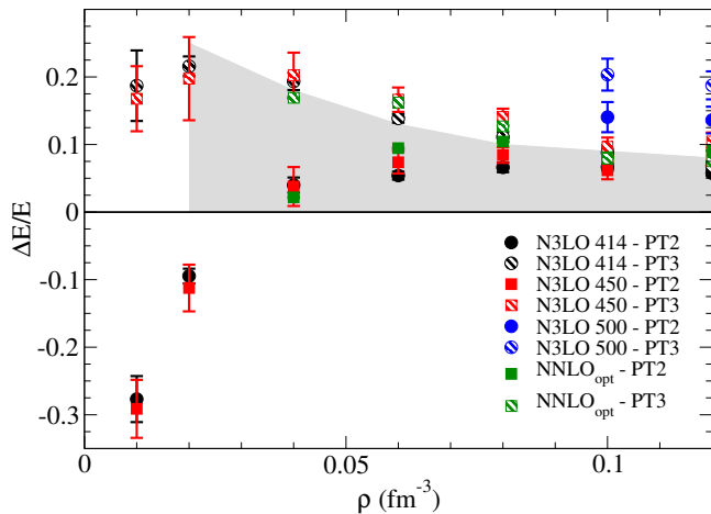
FIG. 5. (color online) Relative deviations of energies obtained at different orders in perturbation theory with respect to the corresponding CIMC result for symmetric nuclear matter. The gray band is a qualitative estimate of the uncertainties in the fixed-node approximation (see text for the details).
