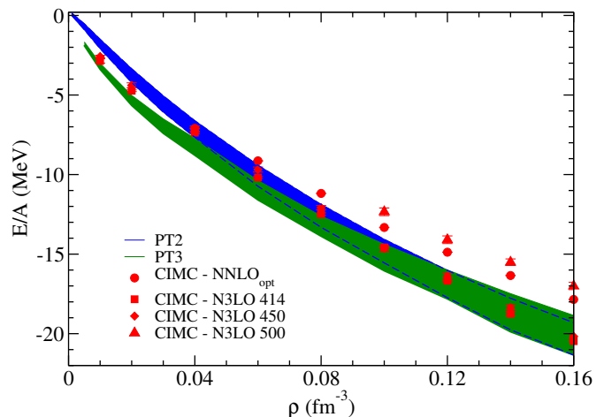
FIG. 3. (color online) Same as in Fig. 1, except for symmetric nuclear matter. The \text{NNLO}_{opt} results now are contained in the N^3\text{LO} bands.
