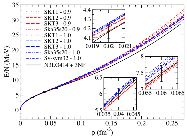
FIG. 7. (color online) Equation of state for pure neutron matter. The insets show the uncertainty bands from neglected correlations in the perturbative treatment from Section II.
