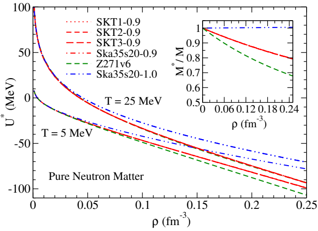
FIG. 11. (color online) Neutron mean field shift and effective mass in pure neutron matter. Note that all “Sk...0.9” Skyrme interactions have nearly identical effective masses.
