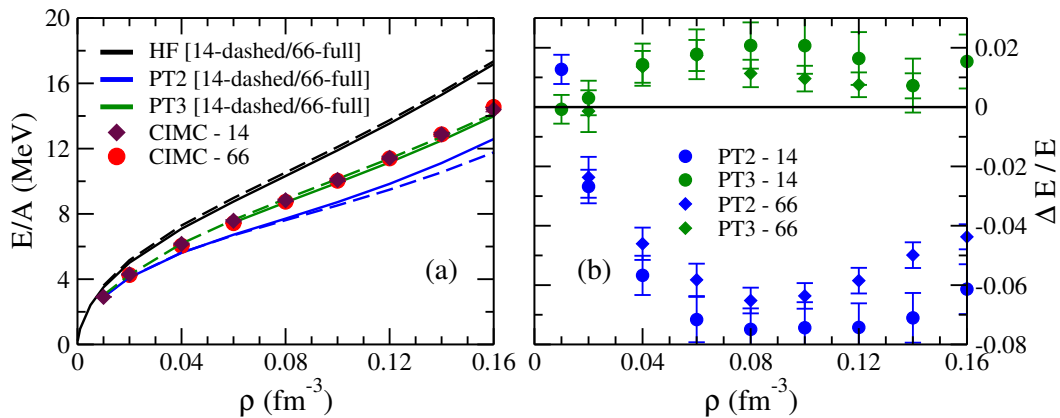
FIG. 17. (color online) (panel (a)): energy per particle in PNM computed with N = 14 and 66 neutrons from CIMC and MBPT using the \text{NNLO}_{opt} chiral two-nucleon potential. (panel (b)): relative differences between the results from CIMC and MBPT at second and third order using N = 14 and 66.
