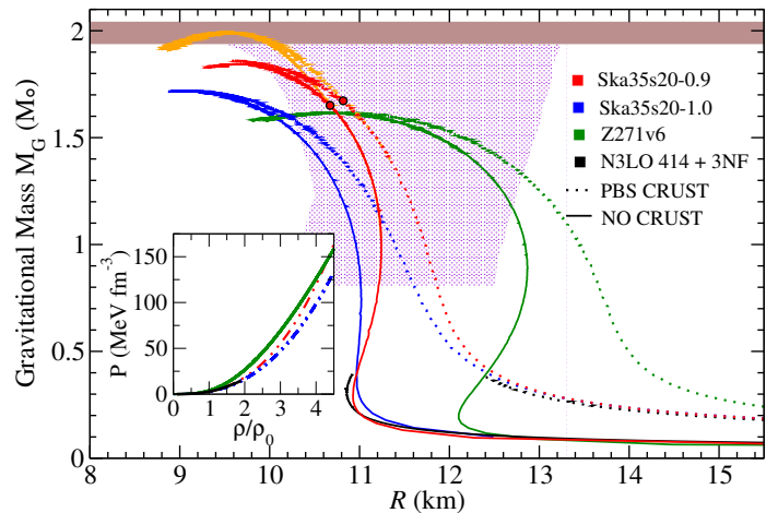
FIG. 15. (color online) Neutron star mass as a function of radius. The mass-radius observational constraint comes from Ref. [98] and the maximum neutron star mass comes from Refs. [4, 5]. We use the BPS crust EoS [99] at low densities. The solid dots indicate the transition region to the constant speed of sound equation of state.
