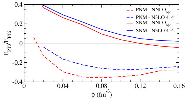
FIG. 4. (color online) Ratio of the third-order correction to the second-order one in PNM (dashed lines) and SNM (full lines) for \text{NNLO}_{opt} (red) and N^3\text{LO} 414 (blue).
