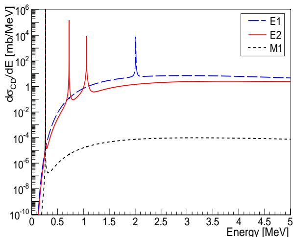
FIG. 3: (Color online) Multipole contributions to the differential cross section of the breakup reaction ^{208}\text{Pb}(^{27}\text{P}, ^{26}\text{Si} p \gamma)^{208}\text{Pb} at 491.3 A MeV incident beam energy.
