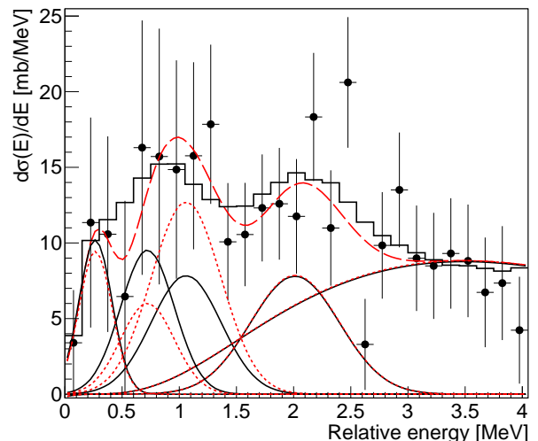
FIG. 13: (Color online) Comparison between the experimental invariant-mass spectrum (solid circles with error bars) and a simulated one using the theoretical predictions (histogram). The solid curves represent Gaussian peaks fitted to the histogram. The red dashed curves and their sum curve (long-dashed) result from fits to the experimental data. Note that in the simulation the strength of the fourth resonance at E_r = 2.01 MeV was scaled down to match the experimental cross section.
