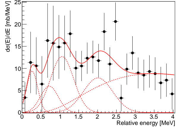
FIG. 12: (Color online) Invariant-mass spectrum for the CD of ^{27}\text{P} feeding directly the ground-state of ^{26}\text{Si} . Nuclear and empty-target contributions have been subtracted (see text).
