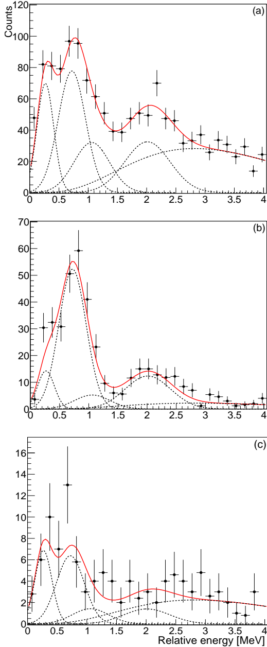
FIG. 11: (Color online) Invariant-mass spectra for ^{27}\text{P} impinging on (a) a ^{nat}\text{Pb} target, (b) a ^{12}\text{C} target, and (c) an empty target frame.
