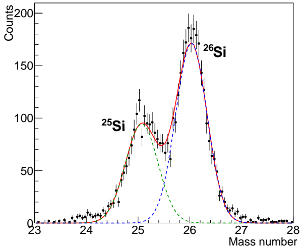
FIG. 7: (Color online) Mass distribution of Si fragments detected behind the Pb breakup target. Events have been selected with gates on ^{27}\text{P} in front of and on Z = 14 (Si) behind the target, in coincidence with a proton in the proton arm.
