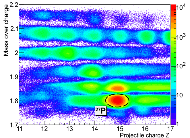
FIG. 5: (Color online) Particle-identification plot of the secondary beam from the FRS as derived from magnetic-rigidity, time-of-flight and energy-loss measurements. The two-dimensional gate used to select ^{27}\text{P} is indicated by the dashed contour line. The color scale is logarithmic.
