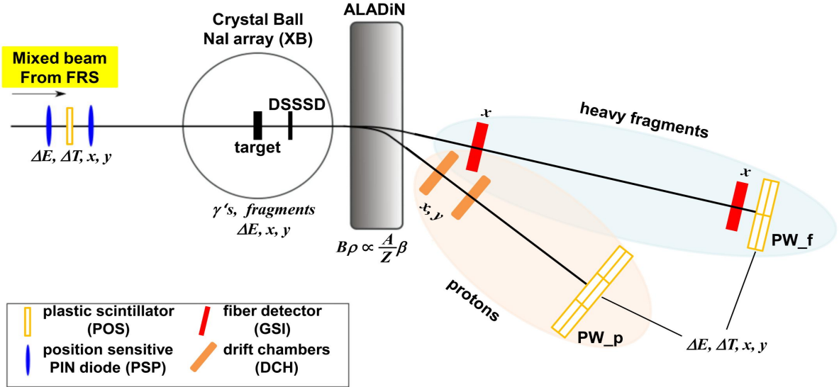
FIG. 4: (Color online) Schematic view of the experimental setup used to detect CD of ^{27}\text{P} in complete kinematics. The physical quantities measured with the various detectors are indicated. Some technical details for the detectors are given in the text. Figure is adapted from Ref. [24].
