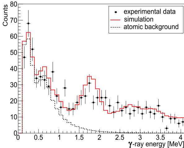
FIG. 10: (Color online) Reconstructed \gamma -ray spectrum from the Crystal Ball for the reaction ^{27}\text{P} \rightarrow ^{26}\text{Si} + \text{proton} in a ^{nat}\text{Pb} target (black circles). The red histogram represents a simulation of the XB response, made with the R3BROOT package. The dashed histogram marks the atomic background (see text for details).
