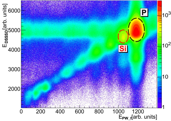
FIG. 6: (Color online) Energy loss measured in the two-layer double-sided Si micro-strip detector (DSSSD) behind the Pb target plotted versus the energy loss in the plastic-scintillator wall (PW.f). The color scale is logarithmic.
