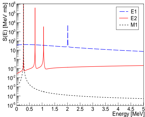
FIG. 2: (Color online) Multipole contributions to the astrophysical S -factor of the radiative-capture reaction ^{26}\text{Si}(p,\gamma)^{27}\text{P} .
