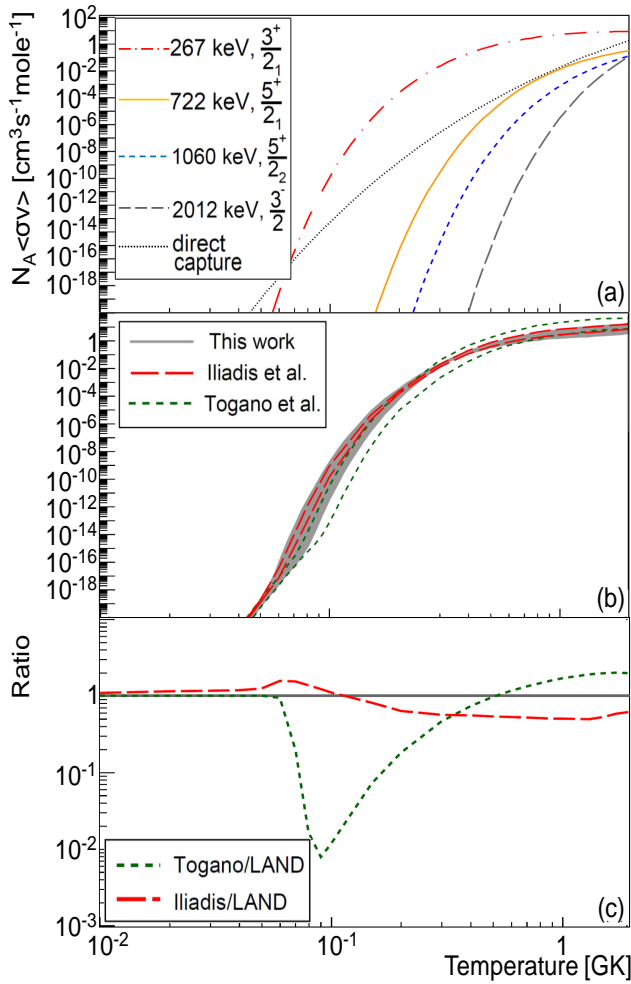
FIG. 14: (Color online) Calculated thermonuclear reaction rates: (a) - the single-resonance and direct-capture contributions from this work; (b) - the \pm 1\sigma -uncertainty bands of the total reaction rates from this work (shaded band) in comparison with those from Togano et al. ([8], short-dashed) and Iliadis et al. ([5], long-dashed); (c) - ratios of the Togano et al. [8] and the Iliadis et al. [5] reaction rates divided by those of the present work.
