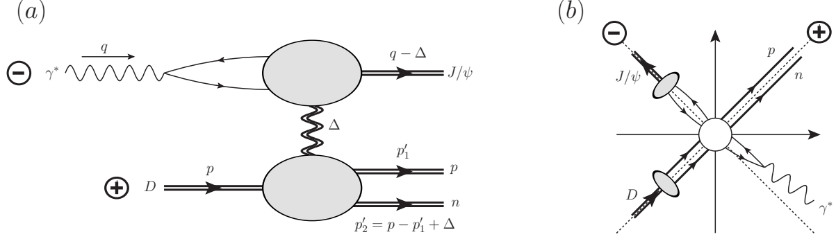
FIG. 1. Schematic illustration of the amplitude for diffractive J/\psi electroproduction on the deuteron: \gamma(q) + D(p) \rightarrow J/\psi(q-\Delta) + p(p'_1) + n(p'_2) . (a) In Regge kinematics, the photon preferentially fluctuates into a quark dipole and scatters from the deuteron by pomeron exchange (double wavy line in the t -channel). (b) Spacetime picture of the collision. The symbols \oplus and \ominus represent the trajectories of the deuteron and photon along the respective light front axes.
