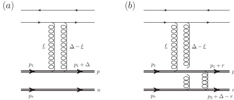
FIG. 3. Examples of the dipole- NN T -matrix which can contribute to (a) the |t| \sim |T| and (b) |t_1| \gg |T| regimes. In the first case, |t| \approx |T| \approx \Delta_T^2 , and in the second case |t| \approx p_{1T}^2 \gg \Delta_T^2 \approx |T| .
