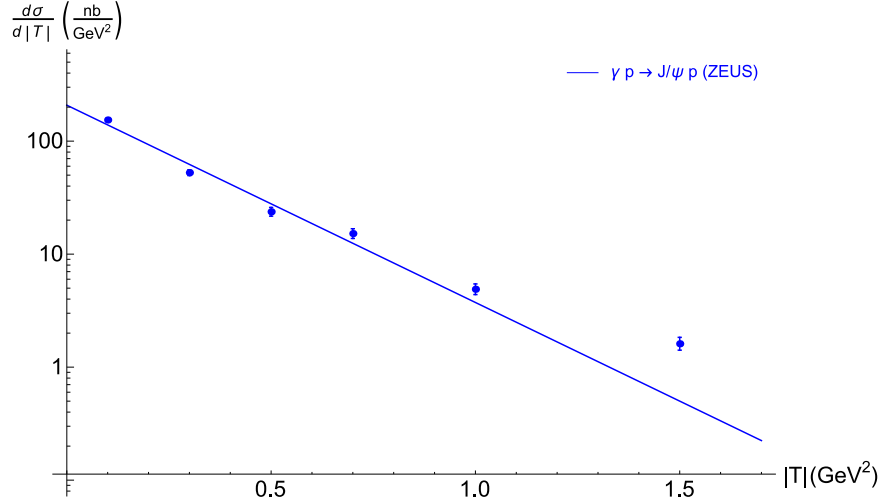
FIG. 14. Selected data for J/\psi photoproduction at HERA. The data and the fit (77) are taken from Ref. [32], corresponding to a photon-proton center-of-mass energy \sqrt{s} = W between 50 GeV and 70 GeV.
