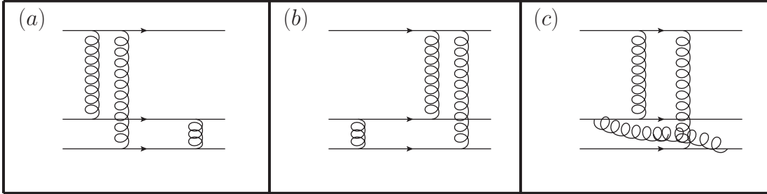
FIG. 4. Representative diagrams from the three classes of nucleon-nucleon interactions. The NN interaction can occur as (a) a final state interaction, (b) an initial state interaction, or (c) a long lived fluctuation. For each class of diagrams there are also minor variations on the topology, such as altering the order in which the projectile scatters on the two nucleons.
