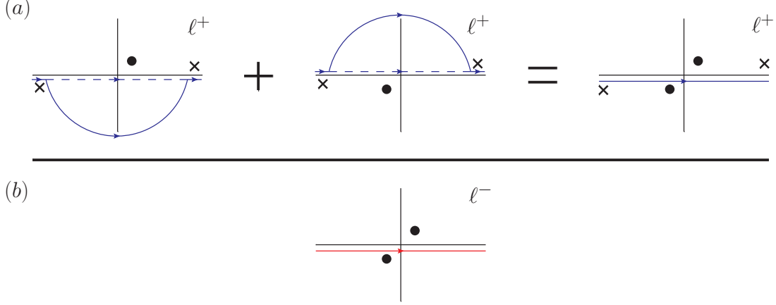
FIG. 7. Pole structure in the complex \ell^\pm plane. (a) The \ell^+ pole corresponds to the intermediate quark propagator from the projectile dipole, with a contour that can be deformed far away from the origin. The magnitude of the deformation is limited by the presence of auxiliary poles (denoted by crosses) from the t -channel gluons. (b) The \ell^- poles correspond to the intermediate proton/neutron propagators.
