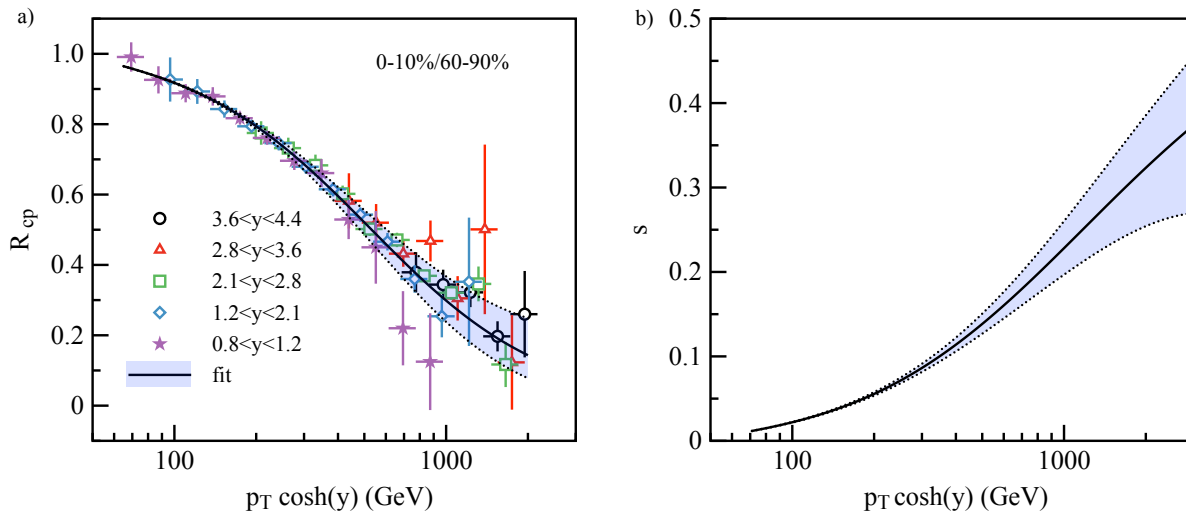
FIG. 3. a) The experimental data [2] for R_{cp} (the ratio of 0 – 10% central to 60 – 90% peripheral) as a function of E_{\text{jet}} = p_{\perp} \cosh(y) at different values of rapidity. The black line and the shaded area shows our fit with uncertainties. b) The corresponding suppression factor, s , dependence on E_{\text{jet}} extracted from the experimental data shown in the left plot.
