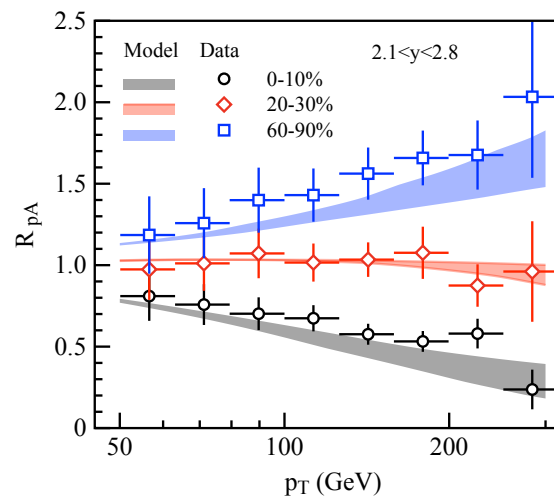
FIG. 4. The comparison of the model results (bands) with the experimental data [2] (points) on R_{pA} as a function of p_{\perp} in the rapidity range 2.1 < y < 2.8 for three centrality classes.
