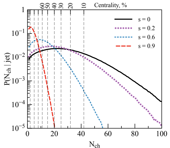
FIG. 1. The probability distribution of the number of charged particles for events with high energy jets P(N_{\text{ch}}|\text{jet}) for the different suppression factors, s . The centrality classes are defined according to the minimum bias probability distribution.
