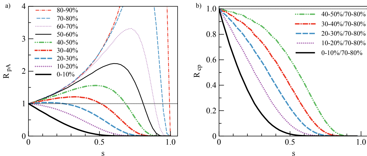
FIG. 2. a) The nuclear modification factor R_{pA} in p +Pb collisions as a function of the soft particle suppression factor s , see Eq. (4), for various centrality classes defined by the number of soft particles in minimum bias events. b) The central-to-peripheral ratio R_{cp} , Eq. (2), where the peripheral class is taken to be 70 – 80% centrality, as a function of the suppression factor s . In our model events with high energy jets are characterized by a suppressed number of soft particles thus shifting these events into more peripheral bins. This naturally results in the suppression (enhancement) of R_{pA} in central (peripheral) collisions, respectively. The suppression factor is expected to grow with jet energy or transverse momentum.
