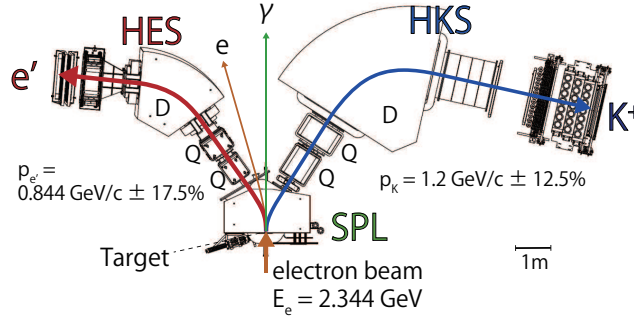
FIG. 1. (Color online) A schematic drawing of the JLab E05-115 experimental geometry. The setup consists of SPL, HKS and HES spectrometers. An electron beam with the energy of 2.344 GeV is incident on the target located at the entrance of SPL. A K^+ and an e' with the momenta of \sim 1 GeV/ c are observed by HKS and HES, respectively.
