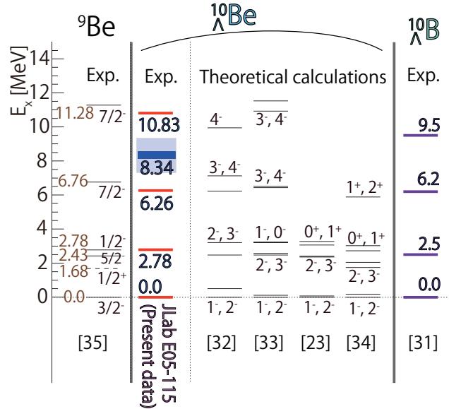
FIG. 5. (Color online) The obtained energy levels of {}^{10}_\Lambda\text{Be} (Fit I) compared to those of the theoretical calculations [23, 32–34]. The energy levels of {}^9\text{Be} [35] and {}^{10}_\Lambda\text{B} [31] are shown for comparisons as well.
