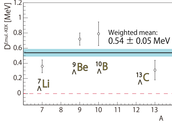
FIG. 6. (Color online) The binding energy differences of {}^7_{\Lambda}\text{Li} , {}^9_{\Lambda}\text{Be} , {}^{10}_{\Lambda}\text{B} and {}^{13}_{\Lambda}\text{C} between the emulsion experiments [16] and the (\pi^+, K^+) experiments [2] with the statistical errors. The values of (\pi^+, K^+) experiments were subtracted from those of the emulsion experiments. The weighted mean was obtained to be +0.54 \pm 0.05 MeV as represented by a solid line. The plots should be on a line of zero (dashed line) if the binding energies measured in the (\pi^+, K^+) and emulsion experiments are consistent.
