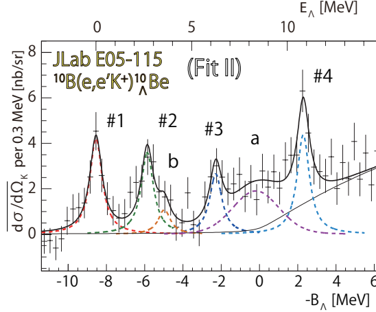
FIG. 4. (Color online) The binding energy ( B_\Lambda ) and excitation energy ( E_\Lambda \equiv B_\Lambda - B_\Lambda(\#1) ) spectra for the ^{10}\text{B}(e, e'K^+)_{\Lambda}^{10}\text{Be} reaction with a fitting result of Fit II. The ordinate axis is \overline{(d\sigma/d\Omega_K)} per 0.3 MeV.
