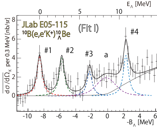
FIG. 3. (Color online) The binding energy ( B_{\Lambda} ) and excitation energy ( E_{\Lambda} \equiv B_{\Lambda} - B_{\Lambda}(\#1) ) spectra for the ^{10}\text{B}(e, e'K^+)^{10}_{\Lambda}\text{Be} reaction with a fitting result of Fit I. The ordinate axis is (\overline{d\sigma/d\Omega_K}) per 0.3 MeV.
