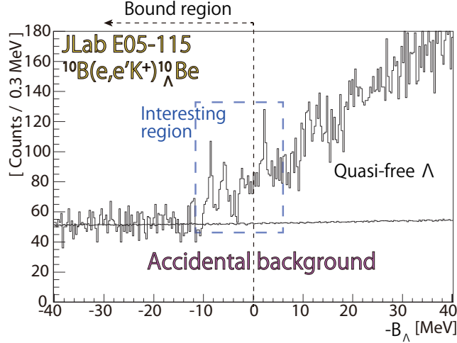
FIG. 2. (Color online) The binding energy spectrum of ^{10}_{\Lambda}\text{Be} . A distribution of an accidental coincidence between an e' and a K^+ was obtained by the mixed event analysis as described in the text.
