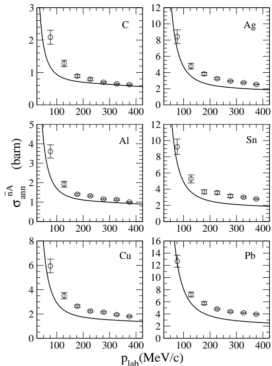
FIG. 6. (Color online) \bar{n}A annihilation cross section as a function of the antineutron momentum in the laboratory frame. Comparing result from Eq.(1) with experimental data from [24].
