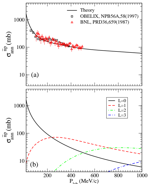
FIG. 2. (Color online)(a) Antineutron-proton annihilation cross sections as a function of the antineutron momentum in the laboratory frame. Solid curve: \bar{n}p annihilation cross section using Eq.(1) without the Gamow factor=1. Solid triangle: experimental data from the OBELIX Collaboration [17] and open circle denotes experimental data from BNL [18]. (b) Contributions from different partial waves to the total annihilation cross sections.
