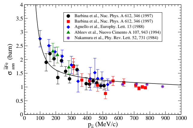
FIG. 5. (Color online) \bar{n}\text{Fe} annihilation cross section as a function of the antineutron momentum in the laboratory frame. Comparing result from Eq.(1) with several sets of experimental data.
