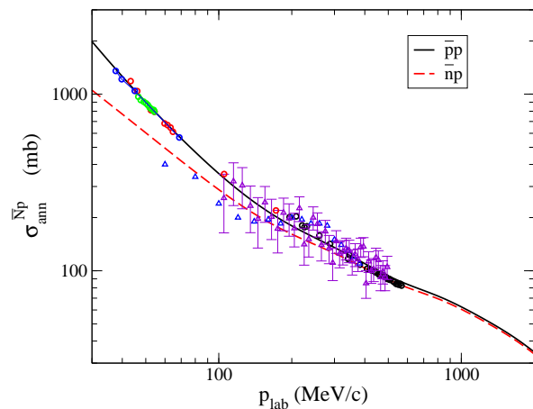
FIG. 3. (Color online) Comparison of \bar{p}p and \bar{n}p annihilation cross sections as a function of the antiproton momentum in the laboratory frame.
