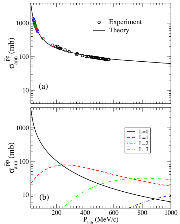
FIG. 1. (Color online) (a) Antiproton-proton annihilation cross sections as a function of the antiproton momentum in the laboratory frame. The solid curve represents the \bar{p}p annihilation cross section of Eq.(1). The experimental data points are from the compilation of [25], where the individual experimental sources can be found. (b) Contributions from different partial waves to the total annihilation cross sections.
