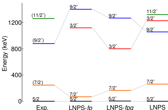
FIG. 7. (Color online) Comparison of the proposed level scheme with shell-model calculations, see text for details. Spin-parity assignments for the upper two levels in the experimental scheme are tentative and based on the systematics of the lighter Mn isotopes and the shell-model calculations.
