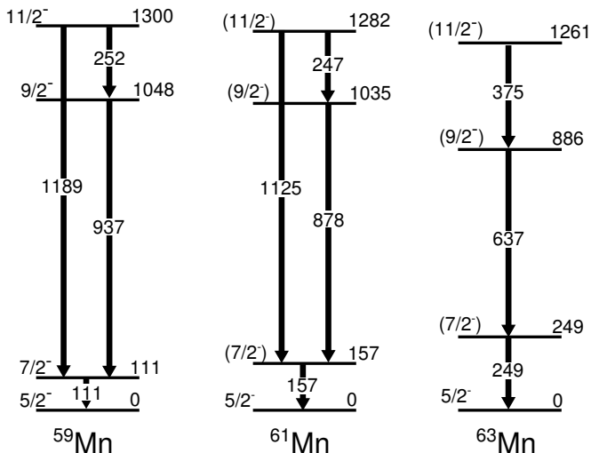
FIG. 6. Comparison of proposed level schemes for ^{59,61,63}\text{Mn} for levels below 1.5 MeV. The level schemes for ^{59,61}\text{Mn} are taken from [15]. The levels are labeled with spin, parity, and excitation energy in keV. Spin-parity assignments for ^{61,63}\text{Mn} are tentative, based on systematics and guided by shell-model calculations. Ground-state spin assignments of J = 5/2 were recently confirmed by laser spectroscopy of the hyperfine structure at ISOLDE [22].
