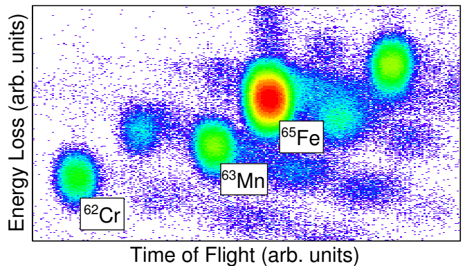
FIG. 1. (Color online) Particle-identification spectrum for the reaction residues produced at the S800 target position by the incoming projectile beam. The magnetic rigidity of the S800 spectrograph was optimized for the transmission of ^{62}\text{Cr} . ^{63}\text{Mn} nuclei can be cleanly separated.
