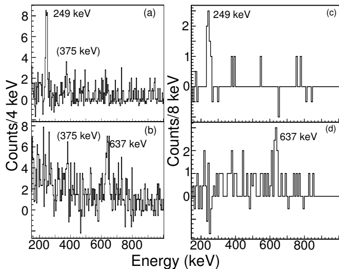
FIG. 3. \gamma\gamma coincidence spectra for ^{63}\text{Mn} detected in the SeGA (a) and (b) and GRETINA arrays (c) and (d), respectively. The top panels, (a) and (c), are gated on the 637-keV transition, and the bottom panels (b) and (d) on the 249-keV \gamma ray. The two transitions are clearly in coincidence.
