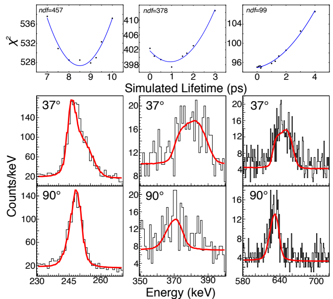
FIG. 5. (Color online) Fits of simulated (GEANT4) \gamma -ray transitions (smooth, red curve) to measured spectra (black histogram) used to determine the excited-state lifetimes of levels depopulated by the 249- (left column), 375- (middle column), 637-keV (right column) transitions. The simulated response is the sum of the simulated transitions and a linear background. Top row: reduced- \chi^2 values versus simulated lifetime used to determine the best-fit \tau value. The number of degrees of the freedom (ndf) entering each lifetime determination is quoted in the \chi^2 plots in the top row.
