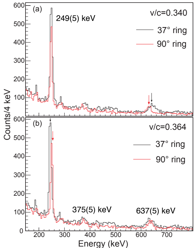
FIG. 4. (Color online) ^{63}\text{Mn} \gamma -ray spectra for the two rings of the SeGA array. In the top panel, v/c=0.340 was used for the event-by-event Doppler reconstruction of the \gamma rays emitted in flight, while in the bottom panel v/c = 0.364 . The position of the peaks in each ring relative to the other is different in each case, illustrating the impact of the excited-state lifetime.
