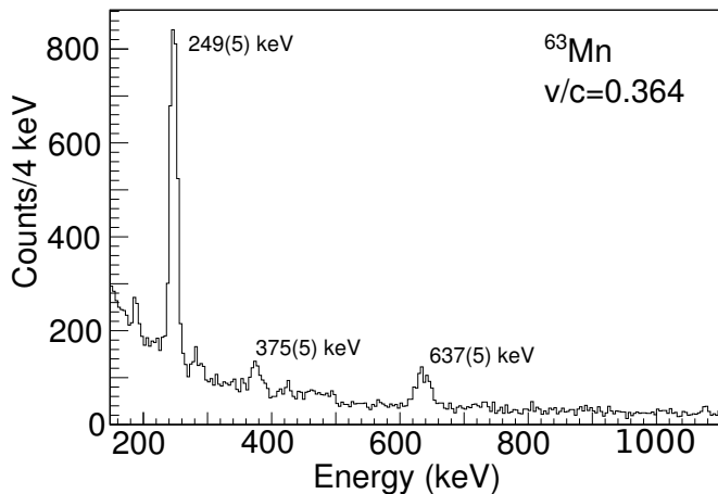
FIG. 2. Event-by-event, Doppler-reconstructed \gamma -ray spectrum detected by the SeGA array in coincidence with ^{63}\text{Mn} reaction products.
