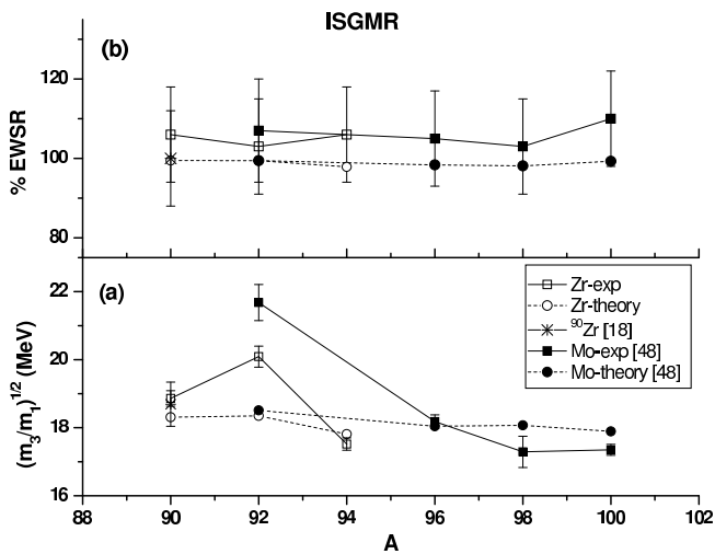
FIG. 9. The scaling energy parameter E_{GMR} = (m_3/m_1)^{1/2} and strength in Zr (this work) and Mo [48] isotopes are shown in the lower (a) and upper panel (b), respectively. The error bars indicate the uncertainty obtained using the errors shown in Figs. 5, 6, and 7. The calculated values using HF-RPA model are also shown.
