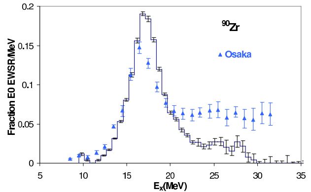
FIG. 8. (Color online) Comparison of ISGMR strength distribution for ^{90}\text{Zr} obtained in this work with that reported by Osaka [37].
