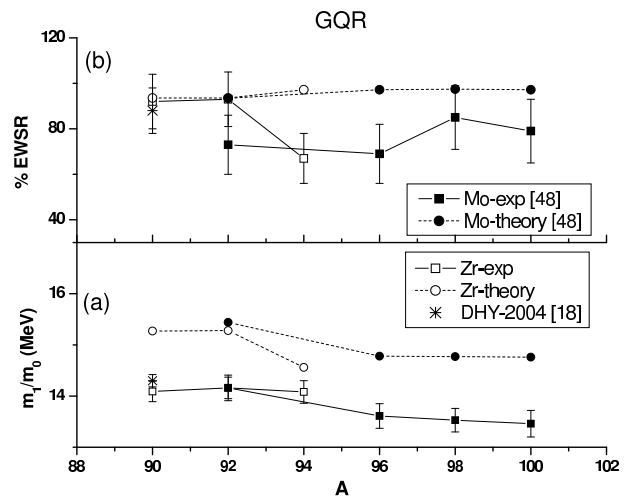
FIG. 12. The centroids and the strengths of the E2 distribution in Zr (this work) and Mo isotopes [48] are plotted against the mass number ( A ) in the lower (a) and upper panel (b), respectively. The error bars indicate the uncertainty obtained using the errors shown in Figs. 5, 6, and 7. Also shown by the circles are the values obtained from HF-RPA calculations with the KDE0v1 interaction.
