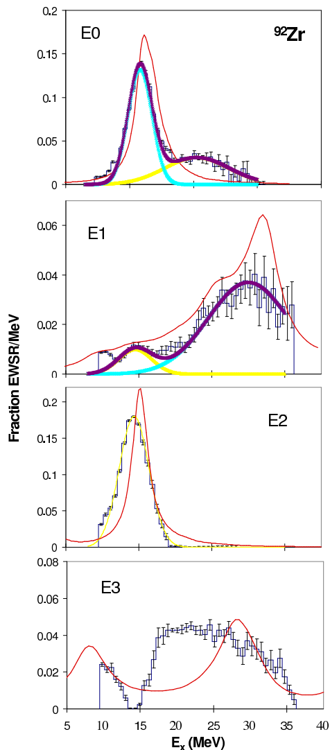
FIG. 6. (Color online) Same as Fig. 5 but for ^{92}\text{Zr} .
