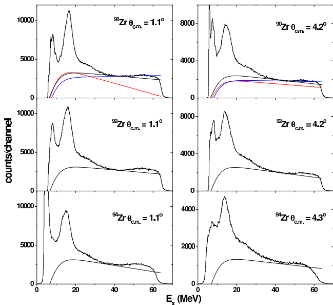
FIG. 1. (Color online) Inelastic \alpha spectra obtained for ^{90,92,94}\text{Zr} . The lines indicate continuum choices, with the variety of choices shown by the different lines in the ^{90}\text{Zr} spectra.
