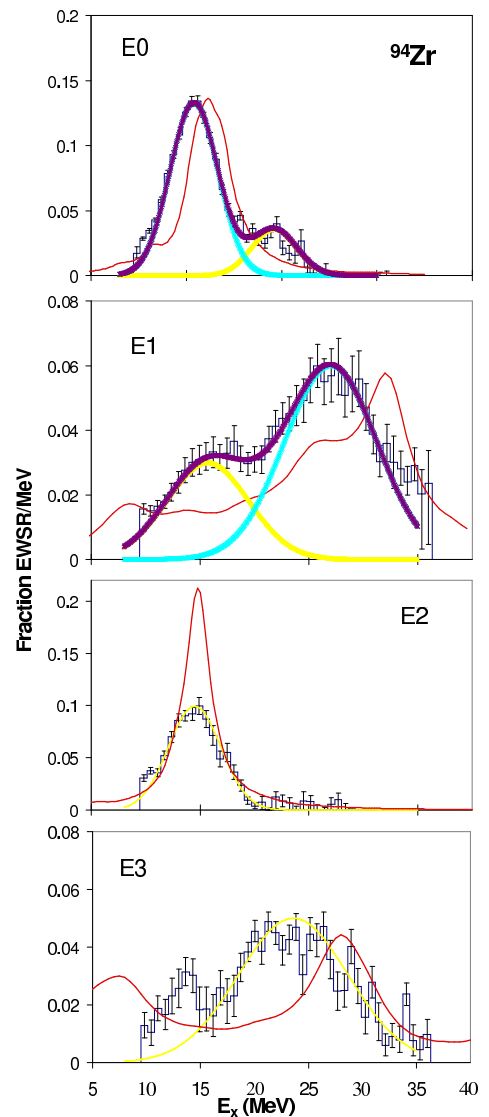
FIG. 7. (Color online) Same as Fig. 5 but for ^{94}\text{Zr} .
