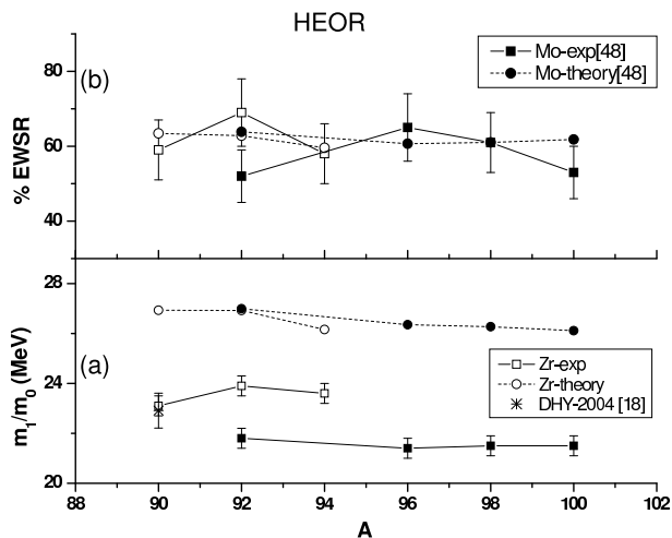
FIG. 13. The centroid of the E3 strength observed in the E3 strength observed above E_x = 15 MeV for each of the Zr (this work) and Mo ([48]) isotopes is plotted vs. A in the lower panel (a), while the strength in this region is plotted in the upper panel (b). The error bars indicate the uncertainty obtained using the errors shown in Figs. 5, 6, and 7. Empty circles show the centroid and strength of E3 distribution in Zr isotopes between E_x = 15 - 35 MeV obtained from the HF-RPA calculations with the KDE0v1 interaction.
